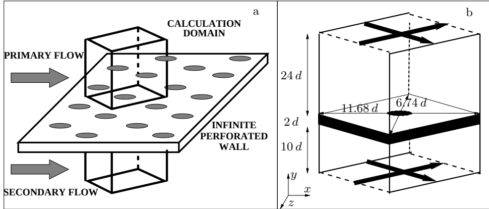
FIGURE 2. From the infinite plate to the ‘bi-periodic’ calculation domain. (a) : Geometry of the infinite perforated wall. (b) : Calculation domain centred on a perforation; the bold arrows correspond to the periodic directions. The dimensions of the computational domain are provided.
