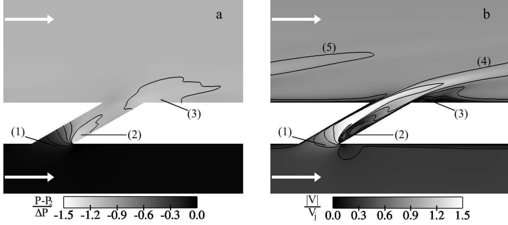
FIGURE 11. Time-averaged quantities from Run C on the centreline plane (zoom over the hole region) (a): Contours and isolines of the time-averaged pressure. (b): Contours and isolines of the time-averaged velocity magnitude |V| . White arrows show the flow direction in both channels.
