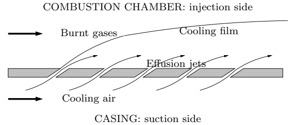
Figure 1: Principle of full-coverage film cooling: fresh air flowing in the casing is injected into the combustion chamber through the liner perforations.
