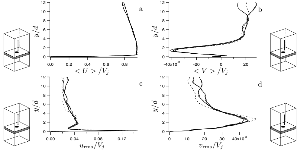
FIGURE 7. Velocity profiles from the 1-hole (---, Run B) and the 4-hole (—, Run D) computations at position (e) in figure 9 ( x = 0 , z = -1.5d ): (a): time averaged streamwise velocity, (b): time averaged normal velocity, (c): RMS of streamwise velocity, (d): RMS of normal velocity.
