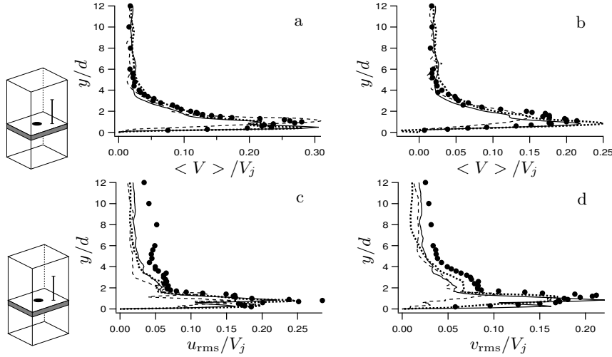
FIGURE 5. Velocity profiles: comparison between experimental results ( \bullet ), Run A ( --- ), Run B ( — ) and Run C ( ..... ). (a): time-averaged vertical velocity at station (c), x = 2.92 d , (b): time-averaged vertical velocity at station (d), x = 5.84 d , (c): streamwise RMS velocity at station (c), x = 2.92 d , (d): vertical RMS velocity at station (c), x = 2.92 d .
