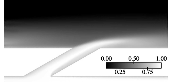
Figure 5: Temperature over the cutting plane located at z = 0 . Temperature is from 0, in the hot gases, to 1 in the cold gases.
