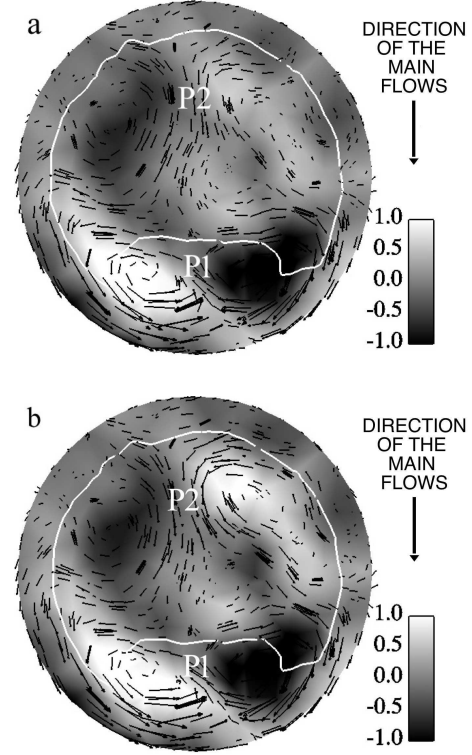
Figure 11: Vorticity in the direction of the hole over a cutting plane orthogonal to the hole axis and velocity vector. White iso-line: momentum magnitude equal to (\rho V)_{jet} . a : isothermal case. b : anisothermal case.
