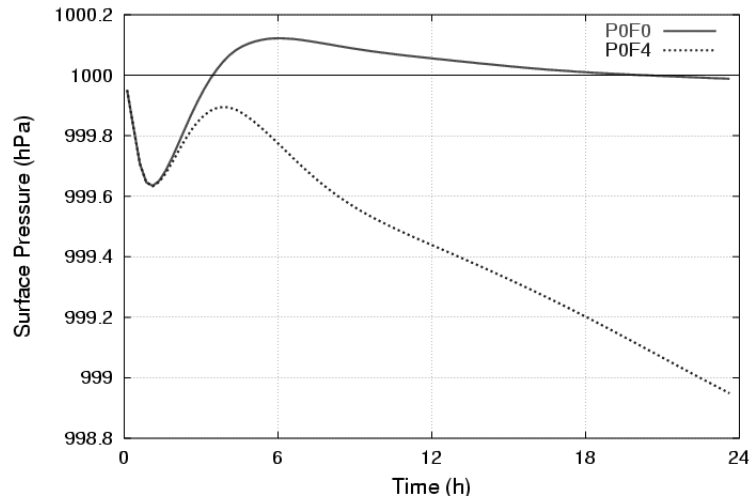
Figure 2.20 Surface pressure ( hPa ) at the center of the heating for F0 and F4 simulations.
