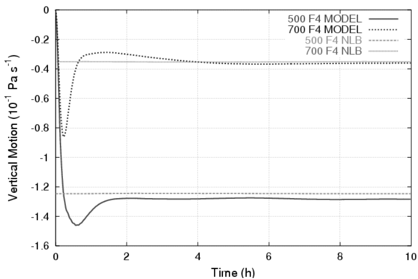
Figure 3.2 Time series of vertical motion \omega ( 10^{-1} Pa s^{-1} ) at 500 and 700 hPa comparing model vs NLB vertical motion, simulation HRF4.
