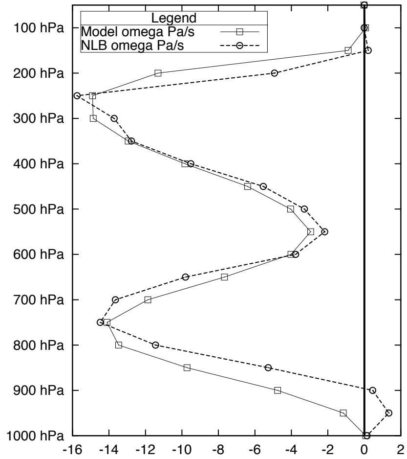
Figure 4.7 Same as fig. 4.5, but a vertical profile at X indicated in fig. 4.5. Horizontal axis is in Pa/s .
