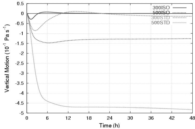
Figure 3.4 Time series of vertical motion \omega ( 10^{-1} Pa s^{-1} ) at 300 and 500 hPa for the isothermal (F0) and the US Standard Atmosphere (USF0) simulations (no rotation).
