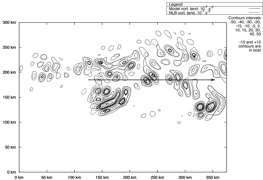
Figure 4.8 GEM-LAM Model (solid) and NLB diagnosed (dashed) vorticity tendency at 750 hPa over a subdomain of the model around the Mississippi Valley (region B highlighted in figure 4.2). 5 h forecast valid at 17 UTC July 7th. Contour interval 5 \times 10^{-7} s^{-2} .
