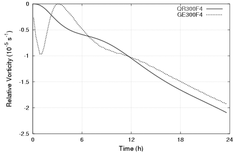
Figure 2.21 Relative and geostrophic vorticity ( 10^{-5} s^{-1} ) at 300 hPa at the center of the heating for the F4 simulation.
