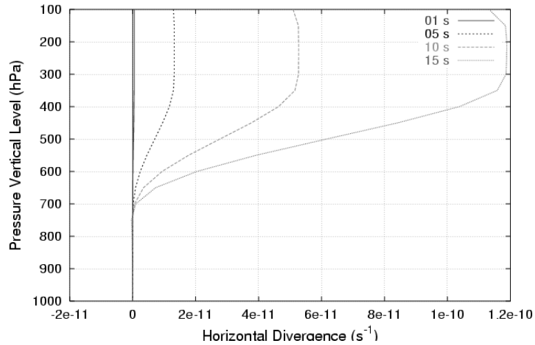
Figure 2.10 Vertical profiles of divergence ( s^{-1} ) at the center of the heating for the first 15 seconds of the simulation. A numerical integration time-step of 1 second is used in this F0 simulation.
