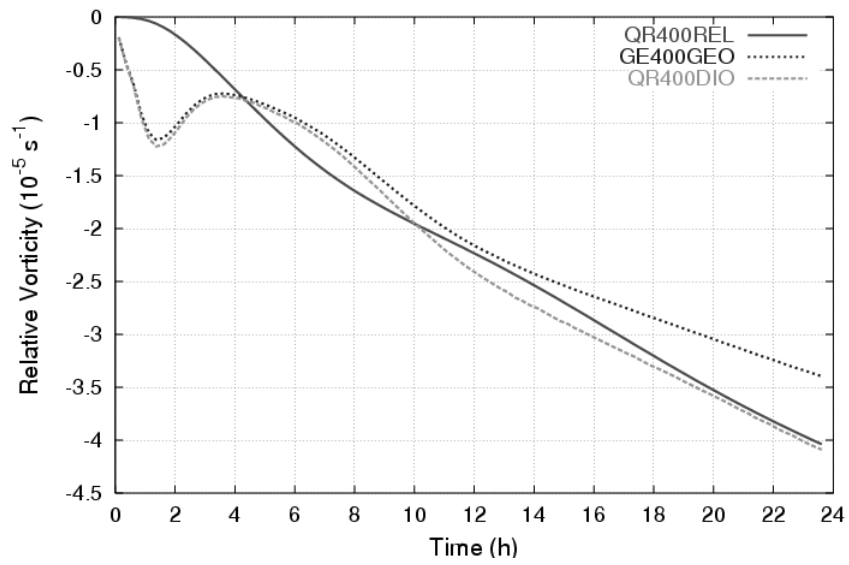
Figure 2.25 Time series of relative vorticity ( 10^{-5} s^{-1} ) at 400 hPa, comparing model (solid black line), NLB (dashed gray line) and geostrophic (dotted black line) for the F4 simulation.
