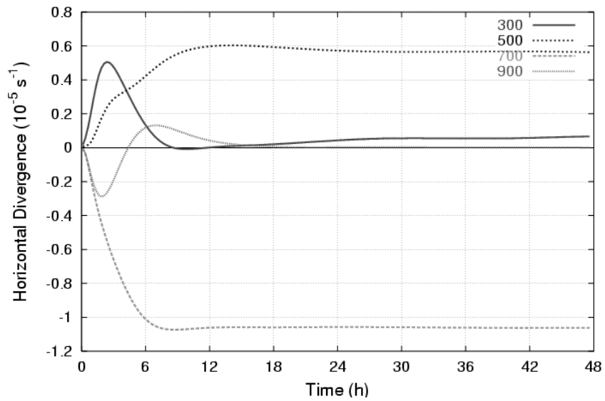
Figure 2.6 Time series of horizontal divergence ( 10^{-5} s^{-1} ) at the center of the heating for the 300, 500, 700 and 900 hPa vertical levels for the F0 simulation.
