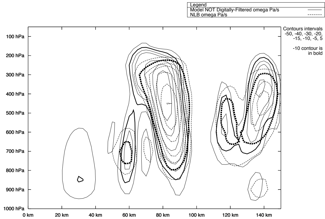
Figure 4.13 Same as fig. 4.12, but a vertical cross-section following the arrow on fig. 4.12.
