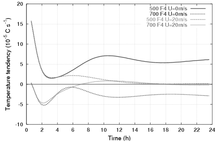
Figure 3.8 Temperature tendency ( 10^{-5}C s^{-1} ) at 500 and 700 hPa with 0 m/s (F4 simulation) and 20 m/s (BWF4 simulation) background winds compared.
