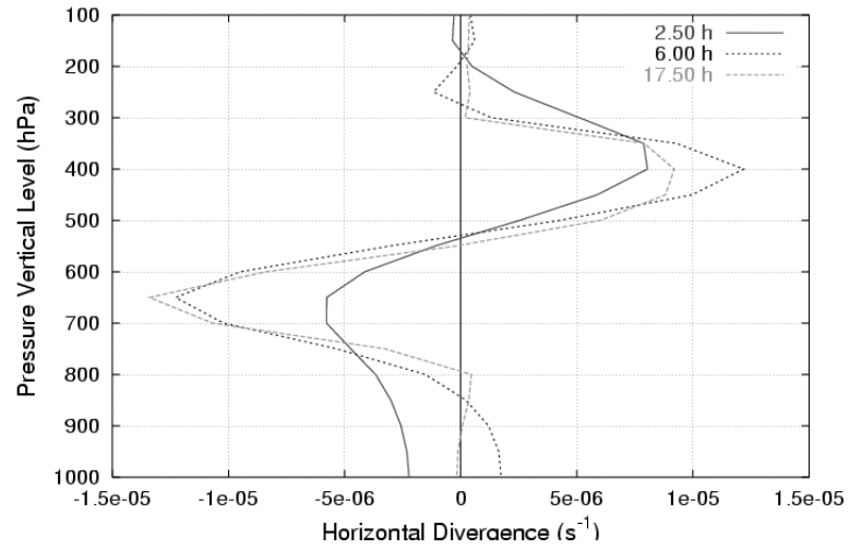
Figure 2.13 Divergence vertical profiles ( s^{-1} ) at the center of the heating at 2h30, 6h and 17h30 for the F0 simulation.
