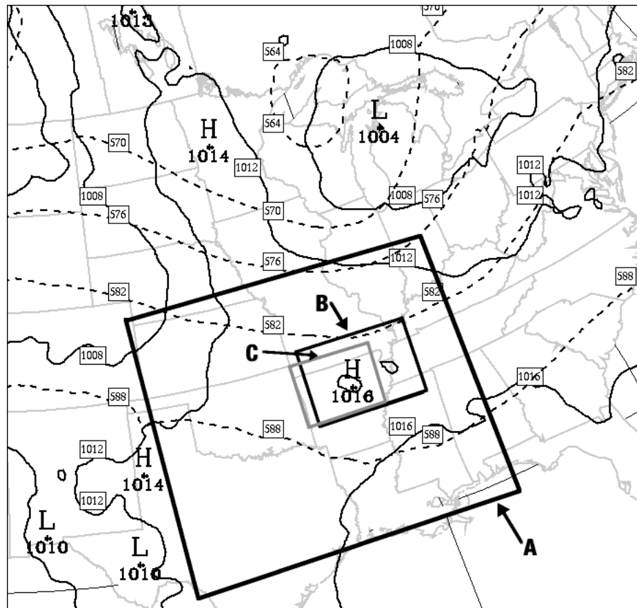
Figure 4.2 A portion of the GEM-REG pilot model domain is shown, along with Mean Sea-Level pressure (solid) and Geopotential Height at 500 hPa (dashed). This is a 17h forecast valid at 17 UTC July 7th 2004. GEM-LAM domain is highlighted (A), along with regions of interest, referenced thereafter (B and C).
