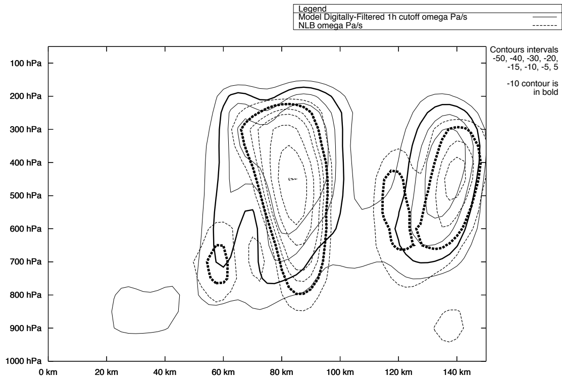
Figure 4.15 Same as fig. 4.14, but a vertical cross-section following the arrow on fig. 4.14.
