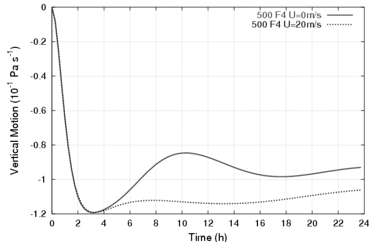
Figure 3.6 Vertical motion \omega ( 10^{-1} Pa s^{-1} ) at 500 hPa with 0 m/s (F4 simulation) and 20 m/s (BWF4 simulation) background winds compared.
