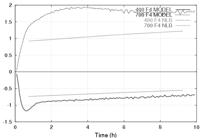
Figure 3.3 Time series of vorticity tendency ( 10^{-9} s^{-2} ) at 400 and 700 hPa comparing model vs NLB vorticity tendency, simulation HRF4.
