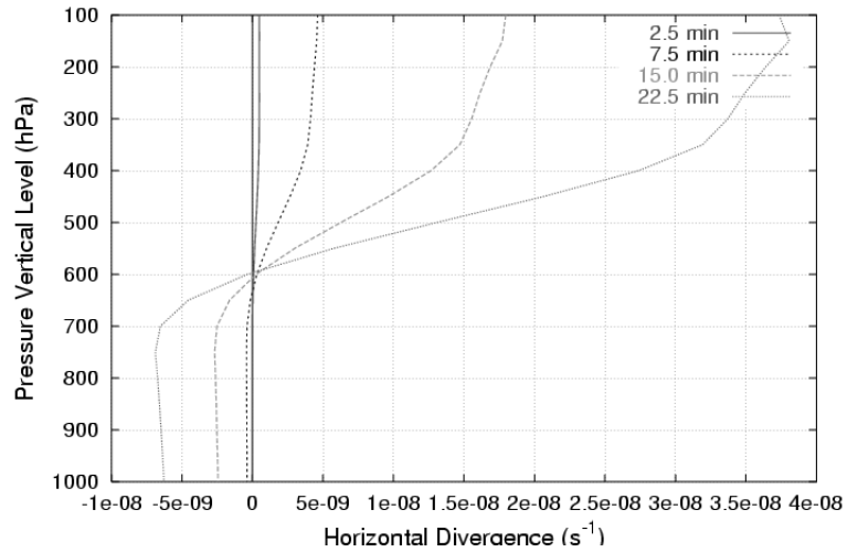
Figure 2.11 Vertical profiles of divergence ( s^{-1} ) at the center of the heating for the first 22.5 minutes of the simulation. A numerical integration time-step of 15 seconds is used in this F0 simulation.
