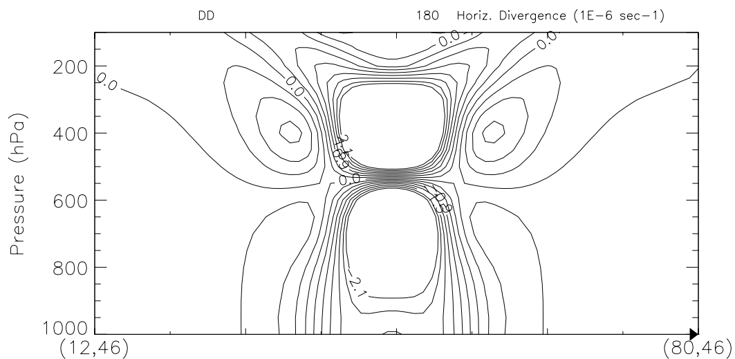
Figure 2.15 Cross-section of horizontal divergence ( 10^{-6} s^{-1} , intervals 0.3 from -2.1 to 2.1) after 3h into the simulation (F0 simulation) for all the horizontal domain up to the numerical sponge edge. Vertical axes are levels of vertical pressure.
