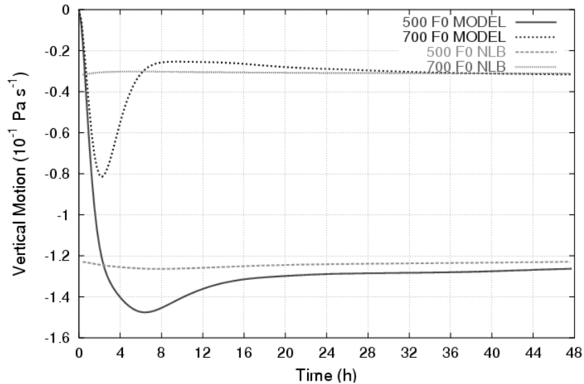
Figure 2.17 Time series of vertical motion \omega ( 10^{-1} Pa s^{-1} ) at 500 and 700 hPa comparing model vs NLB vertical motion for the F0 simulation.
