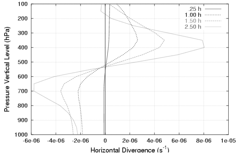
Figure 2.12 Divergence vertical profiles ( s^{-1} ) at the center of the heating at 15 min, 1h, 1h30 and 2h30 for the F0 simulation.
