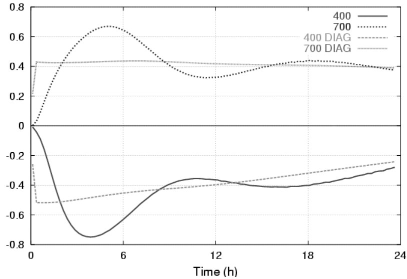
Figure 2.24 Time series of vorticity tendency ( 10^{-9} s^{-2} ) at 400 and 700 hPa comparing model vs NLB vorticity tendency for the F4 simulation.
