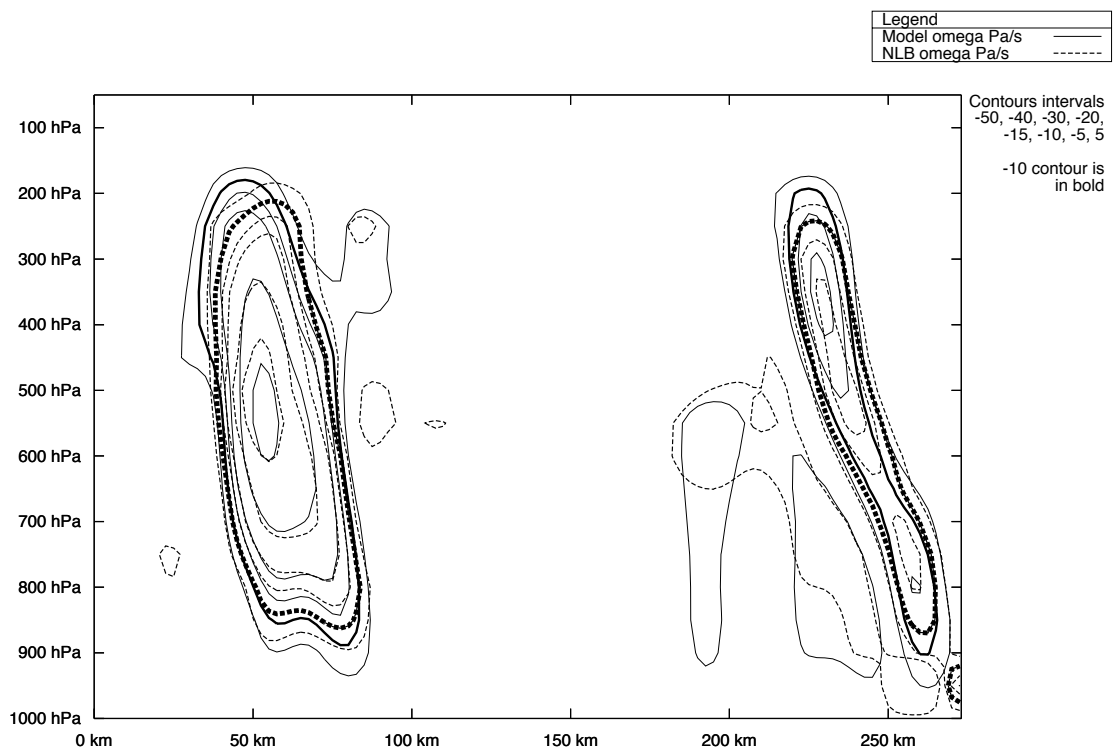
Figure 4.6 Same as fig. 4.5, but a vertical cross-section following the arrow on fig. 4.5.
