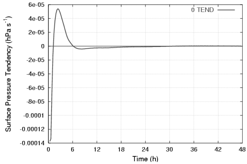
Figure 2.5 Time series of surface pressure tendency ( hPa s^{-1} ) at the center of the heating for the F0 simulation.
