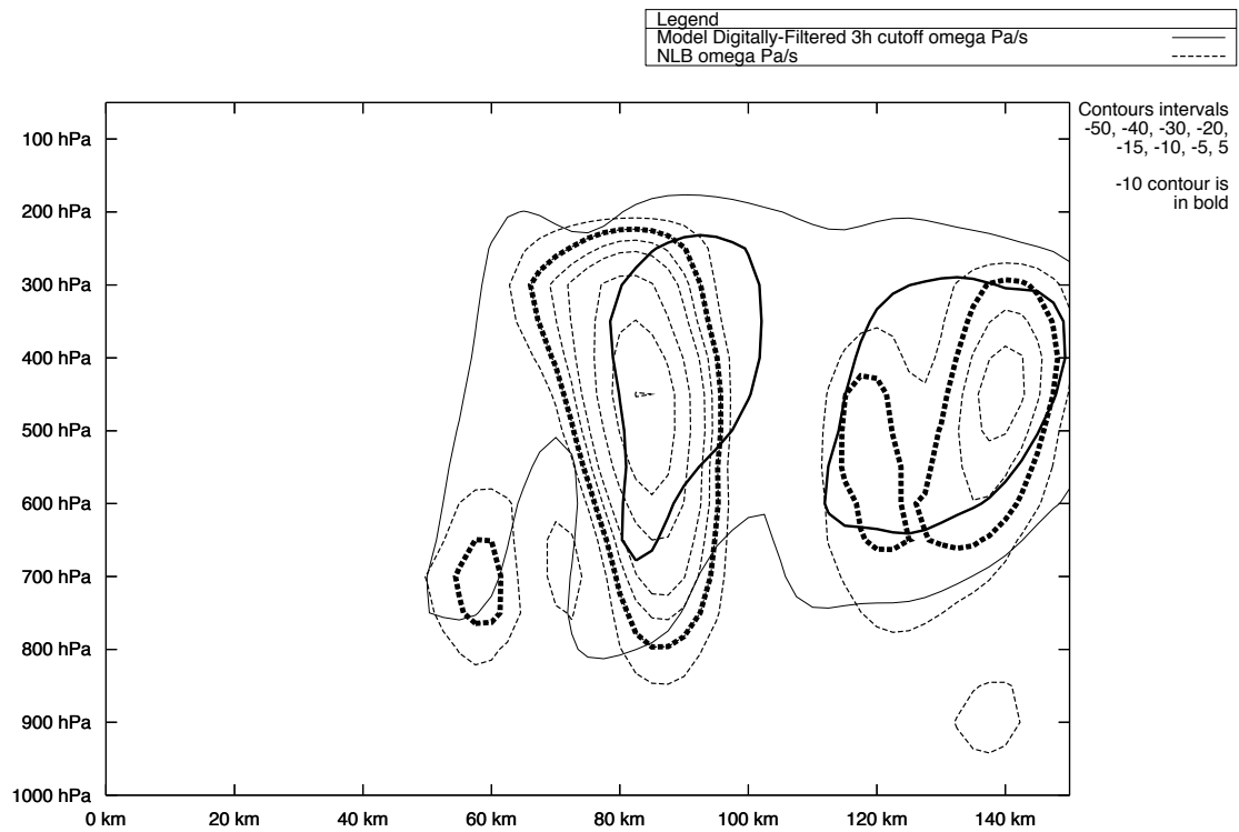
Figure 4.11 Same as fig. 4.10, but a vertical cross-section following the arrow on fig. 4.10.
