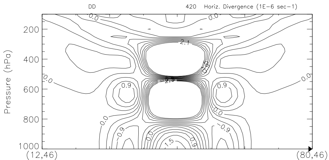
Figure 2.16 Cross-section of horizontal divergence ( 10^{-6} s^{-1} , intervals 0.3 from -2.1 to 2.1) after 7h into the simulation (F0 simulation) for all the horizontal domain up to the numerical sponge edge. Vertical axes are pressure vertical levels.
