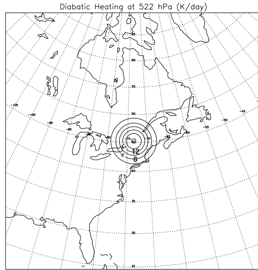
Figure 2.1 Idealized diabatic heating ( K/day ) for the F0 and F4 simulations at its maximum level ( 522 hPa ). Geography is shown for reference only ( f -plane)
