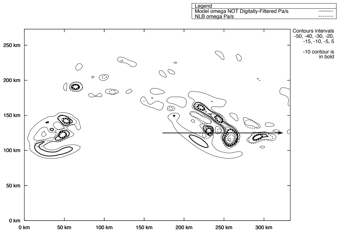
Figure 4.12 Same as fig. 4.10 except the model vertical motion is unfiltered.
