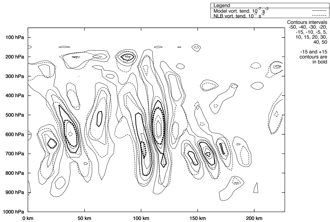
Figure 4.9 Same as fig. 4.8, but a vertical cross-section following the arrow on fig. 4.8.
