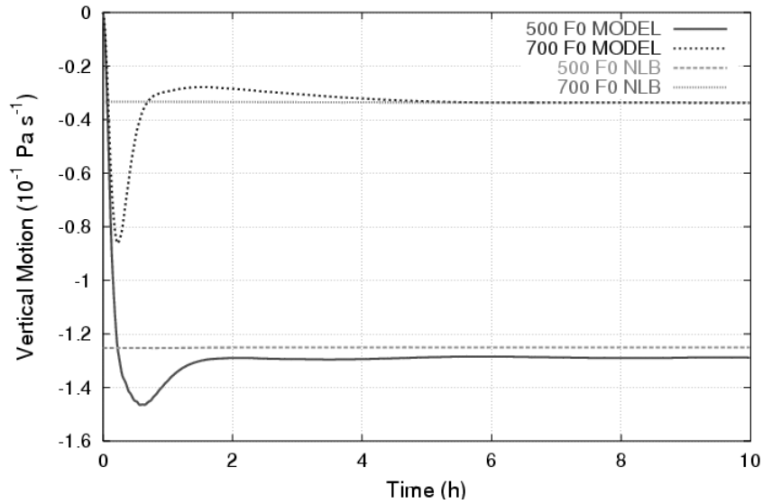
Figure 3.1 Time series of vertical motion \omega ( 10^{-1} Pa s^{-1} ) at 500 and 700 hPa comparing model vs NLB vertical motion, simulation HRF0.
