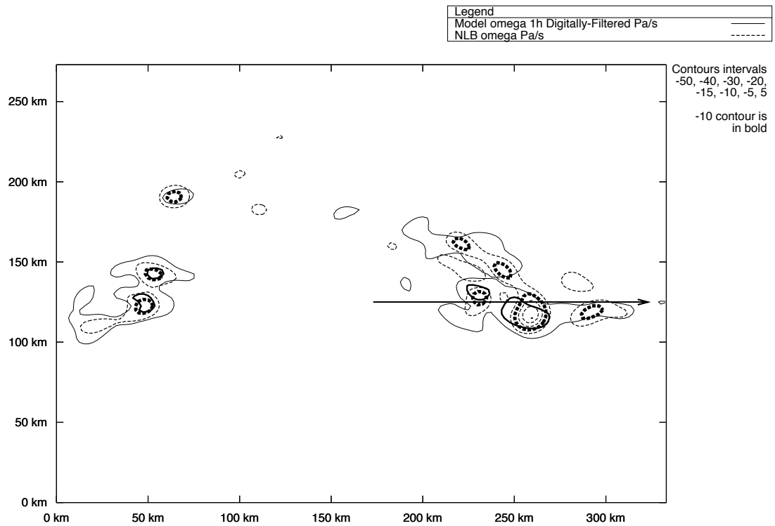
Figure 4.14 Same as fig. 4.10 except the model vertical motion is using a 1h cutoff digital filter.
