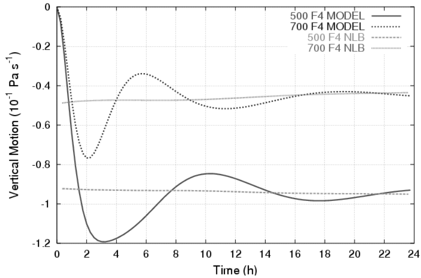
Figure 2.23 Time series of vertical motion \omega ( 10^{-1} Pa s^{-1} ) at 500 and 700 hPa comparing model vs NLB vertical motion for the F4 simulation. NLB vertical motion is identified as NLB in the figure legend.
