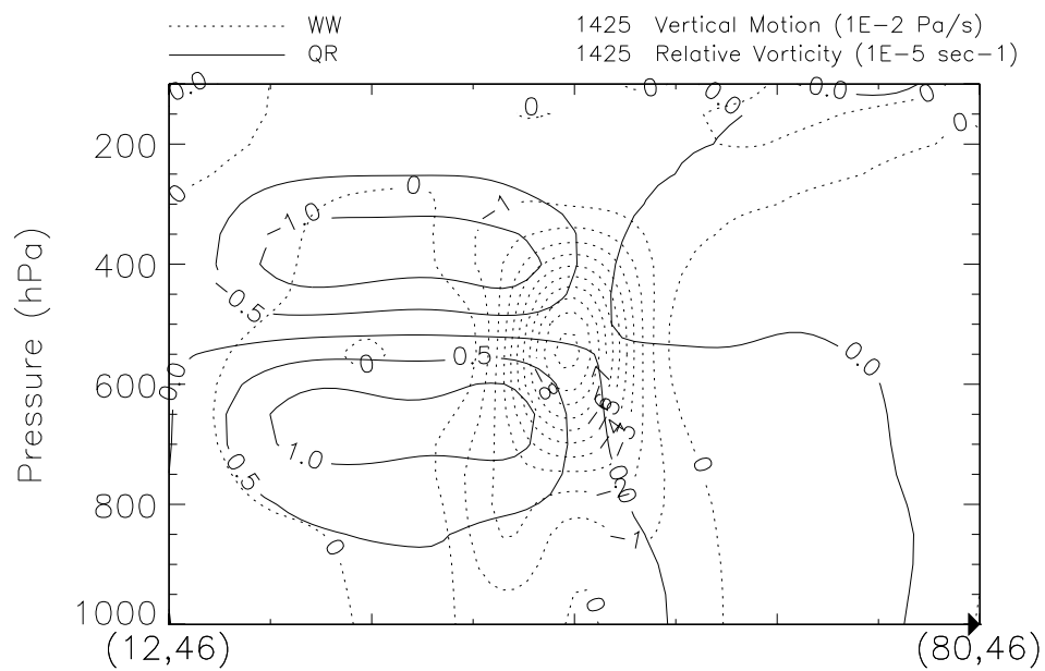
Figure 3.5 Vertical cross-section (west to east) through the center of the heating (on an x-axis) of vertical motion \omega ( 10^{-2} Pa s^{-1} dotted lines) and relative vorticity ( 10^{-5} s^{-1} solid lines) at 24h in the BWF4 simulation (easterly winds of 20 m/s). Vertical axis represents pressure levels.
