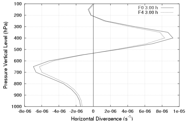
Figure 2.22 Divergence ( s^{-1} ) vertical profiles at the center of the heating for F0 and F4 simulations, after 3h of simulation, at the beginning of significant differences between the two simulations.
