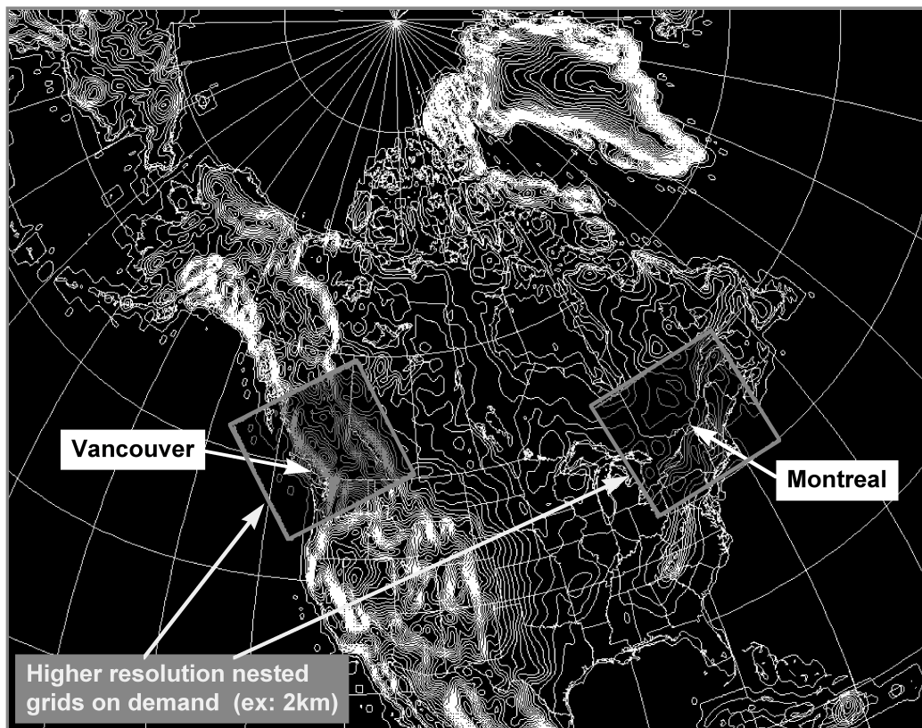
Figure 4.1 Target Grid for Regional 48H Forecast at 10 km using GEM-LAM
