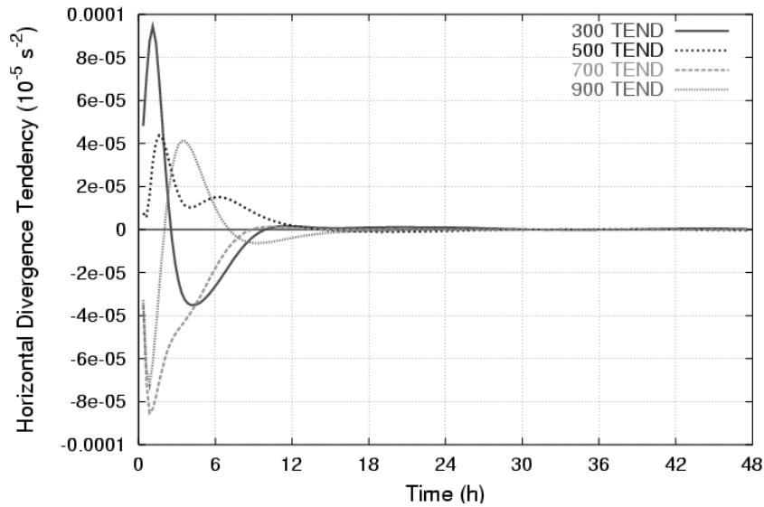
Figure 2.7 Time series of horizontal divergence tendency ( 10^{-5} s^{-2} ) at the center of the heating for the 300, 500, 700 and 900 hPa vertical levels for the F0 simulation.
