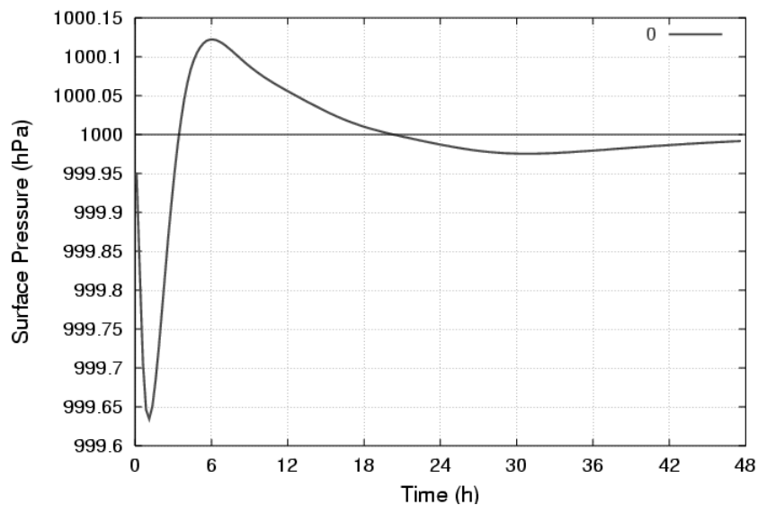
Figure 2.4 Time series of surface pressure ( hPa ) at the center of the heating for the F0 simulation.
