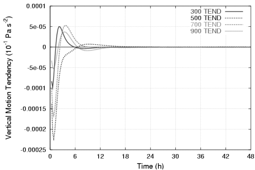
Figure 2.3 Time series of vertical motion tendency ( 10^{-1} Pa s^{-2} ) at the center of the heating for the 300, 500, 700 and 900 hPa vertical levels for the F0 simulation.
