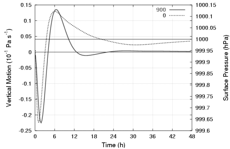
Figure 2.14 Time series of 900 hPa vertical motion \omega ( 10^{-1} Pa s^{-1} ) and surface pressure at the center of the heating for the F0 simulation.
