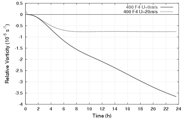
Figure 3.7 Relative vorticity ( 10^{-5} s^{-1} ) at 400 hPa with 0 m/s (F4 simulation) and 20 m/s (BWF4 simulation) background winds compared.
