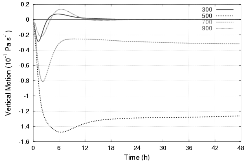
Figure 2.2 Time series of vertical motion ( 10^{-1} Pa s^{-1} ) at the center of the heating for the 300, 500, 700 and 900 hPa vertical levels for the F0 simulation.
