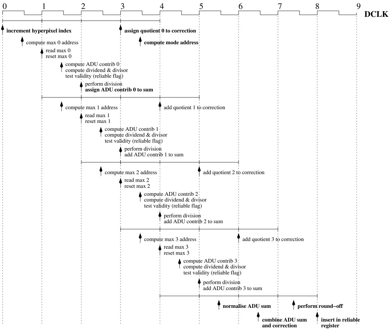
Figure 12.16: Exploded Mode pipeline (operations not carried out for every cycle are typeset with bold letters). The operations shown correspond to the determination of a single background estimate based on the max data words corresponding to the four histograms. The processing for the next estimate starts immediately after so that the each block should be replicated as soon as it ends (ie. the next “increment hyperpixel index” occurs for the rising of edge of DCLK numbered 4).
