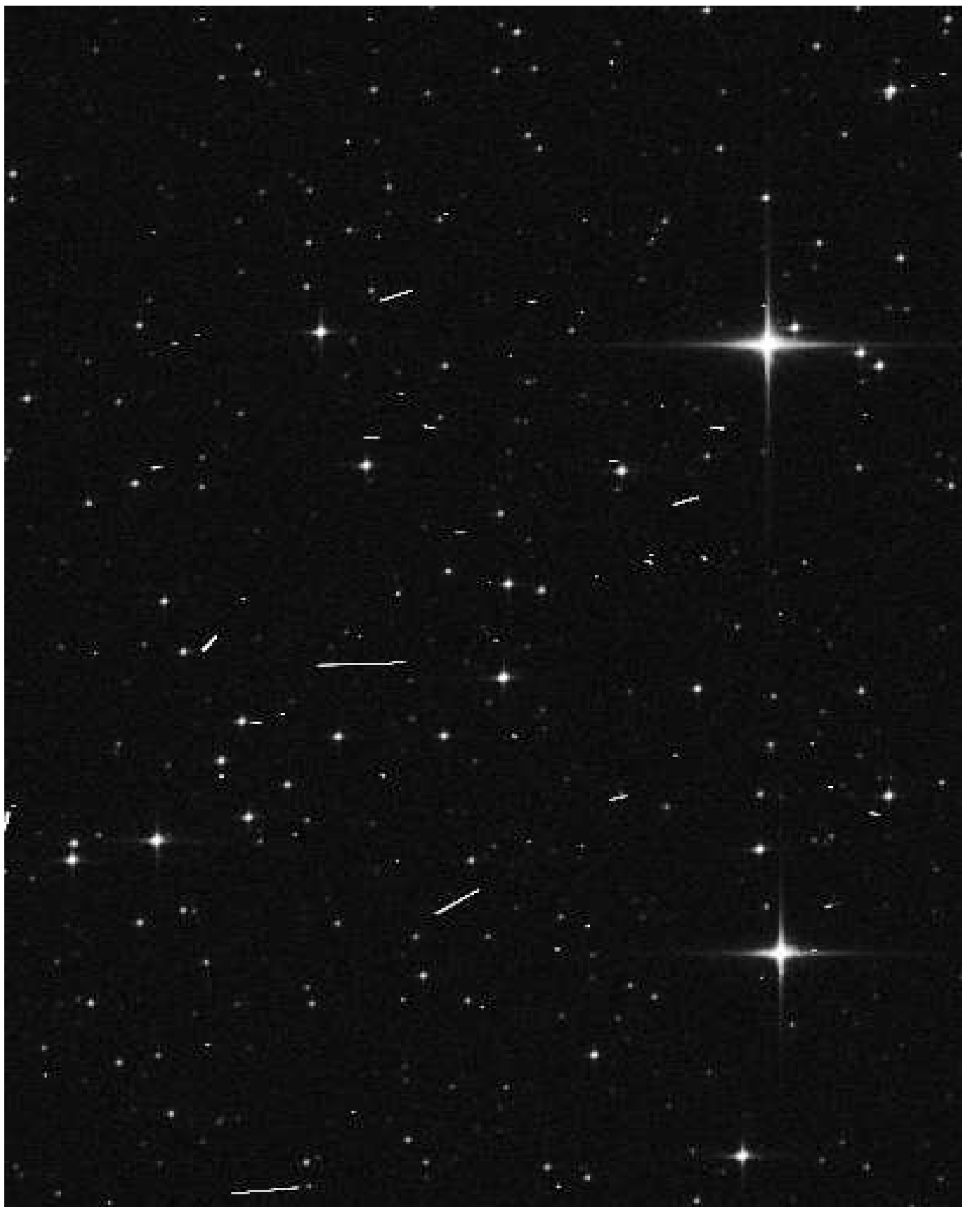
Figure C.4: The design density test case ( 609000 \text{ stars/deg}^2 ) at galactic coordinates l = 54 and b = 0 (in the disk). The snapshot is approximately 400 \text{ AL} \times 525 \text{ AC SM} samples.
