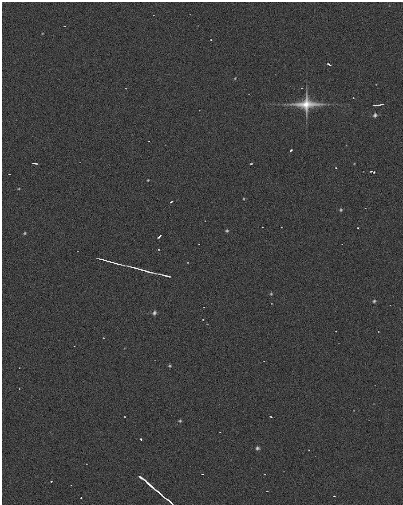
Figure C.2: The average density test case ( 22250 \text{ stars/deg}^2 ) at galactic coordinates l = 74 and b = 15 . The snapshot is approximately 400 \text{ AL} \times 525 \text{ AC} SM samples.
