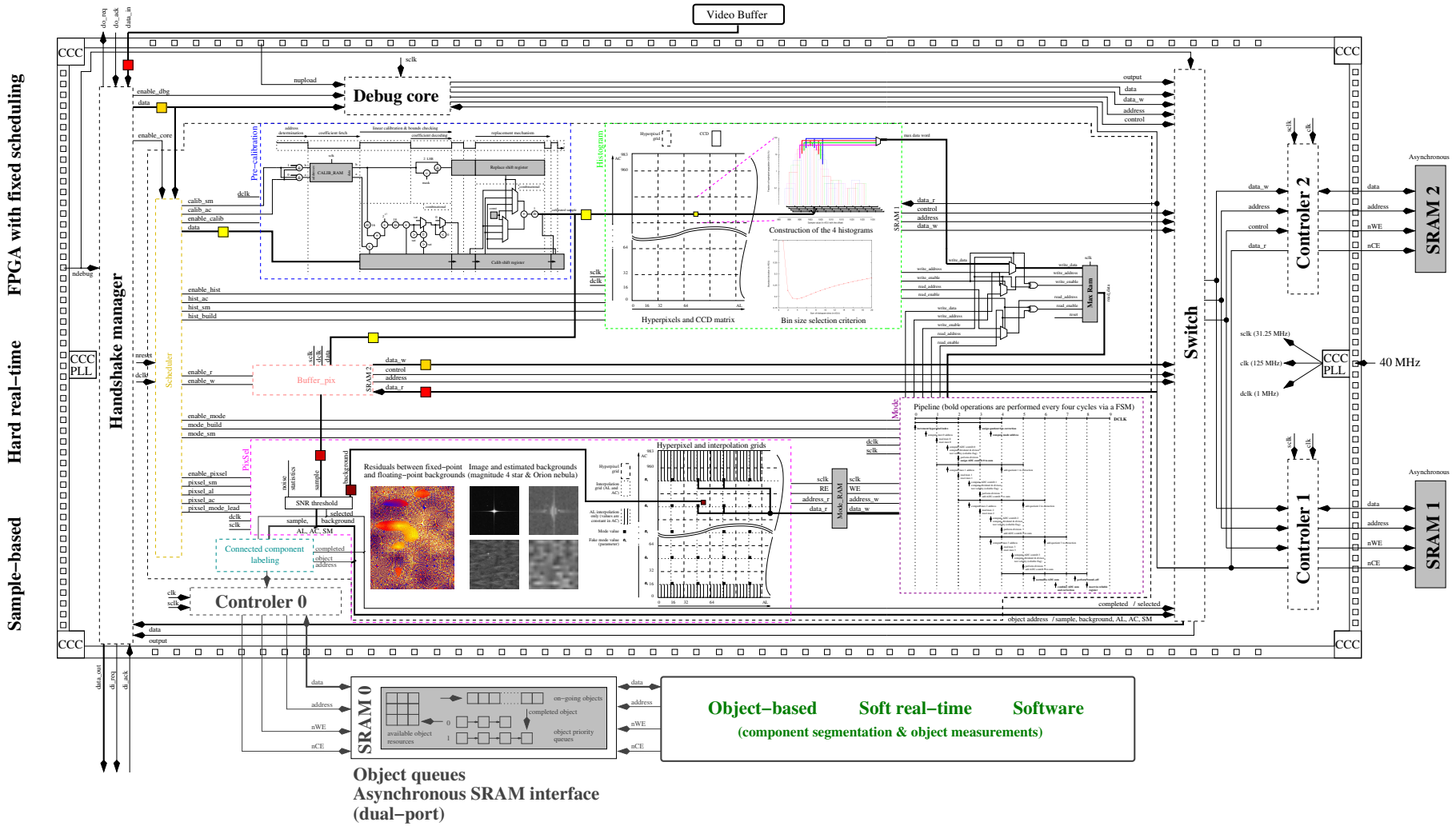
Figure 3.7: Overview of the internal structure of the FPGA.
