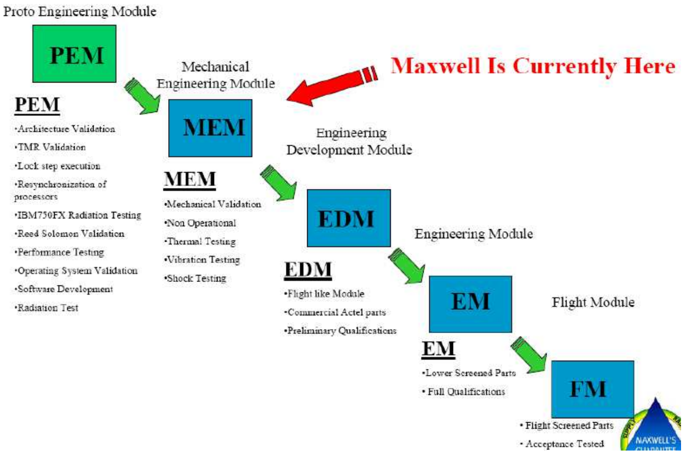
Figure 2.3: Maxwell’s development plan for the single board PPC750FX-based space computer (SCS750) and status at the end of the PDHE TDA (courtesy of Astrium GmbH [25]).
