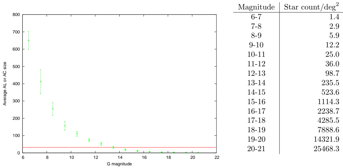
Figure 5.2: Left: average sizes of objects as a function of magnitude in units of SM samples (the line corresponds to the hyperpixel's selected AL and AC dimension: 32 samples). Right: object count previsions averaged over the entire sky per square degree according to [39] (extrapolated to low magnitudes).
