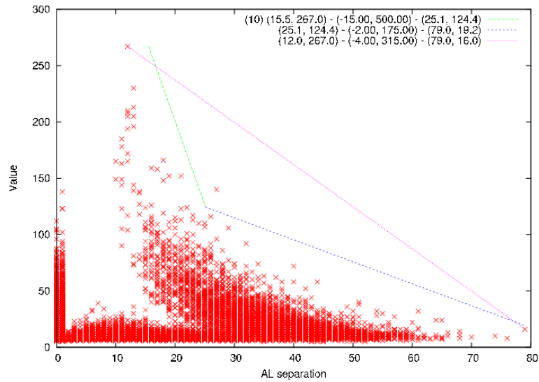
Figure 7.12: Spurious maxima and associated envelopes in the AL direction (in samples) for sources in the range G \in [10, 11[ . The key provides the coordinates of control points (A, B) and the parameters in the piece-wise linear equation connecting A and B ( y = a.x + b ) in the following format: (x_A, y_A) - (a, b) - (x_B, y_B) .
