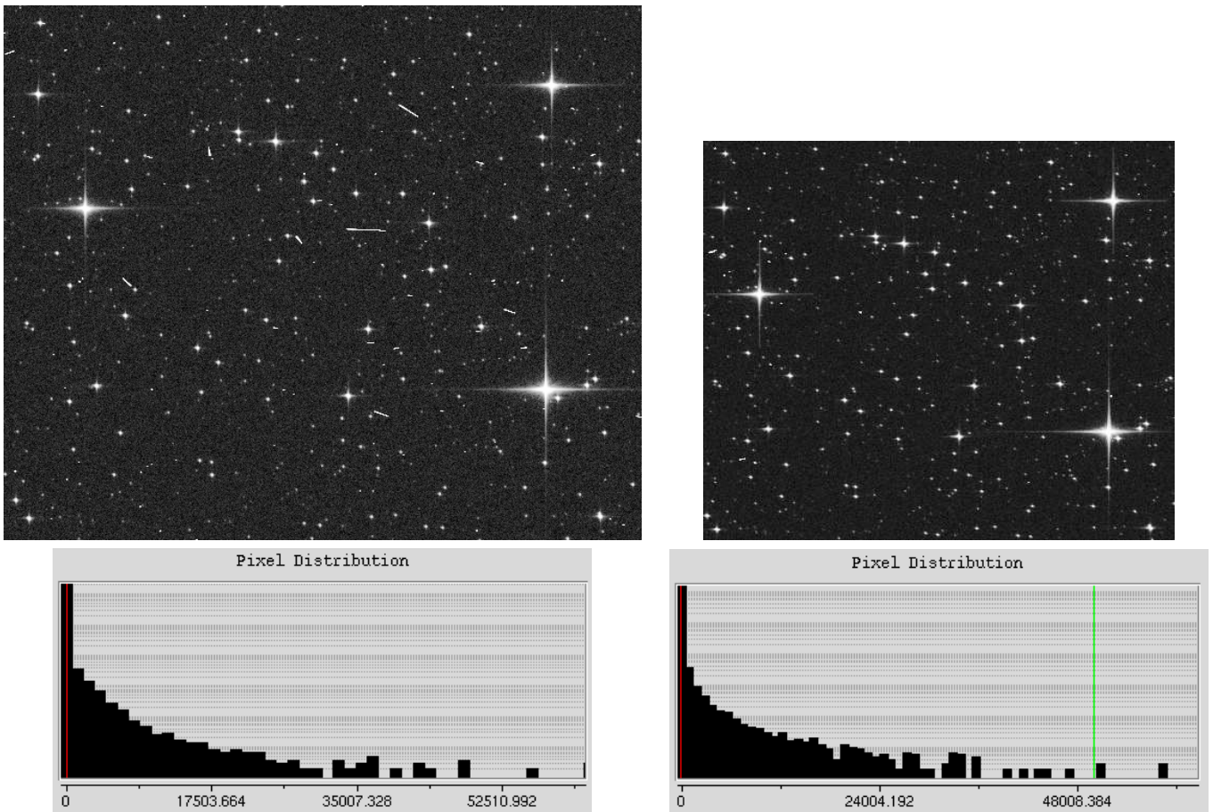
Figure 3.2: Illustration of the impact of the design changes on SM imaging with a high density synthetic example (left: 2002 baseline, right: 2006 design). The two images share the same scale and dynamics.
