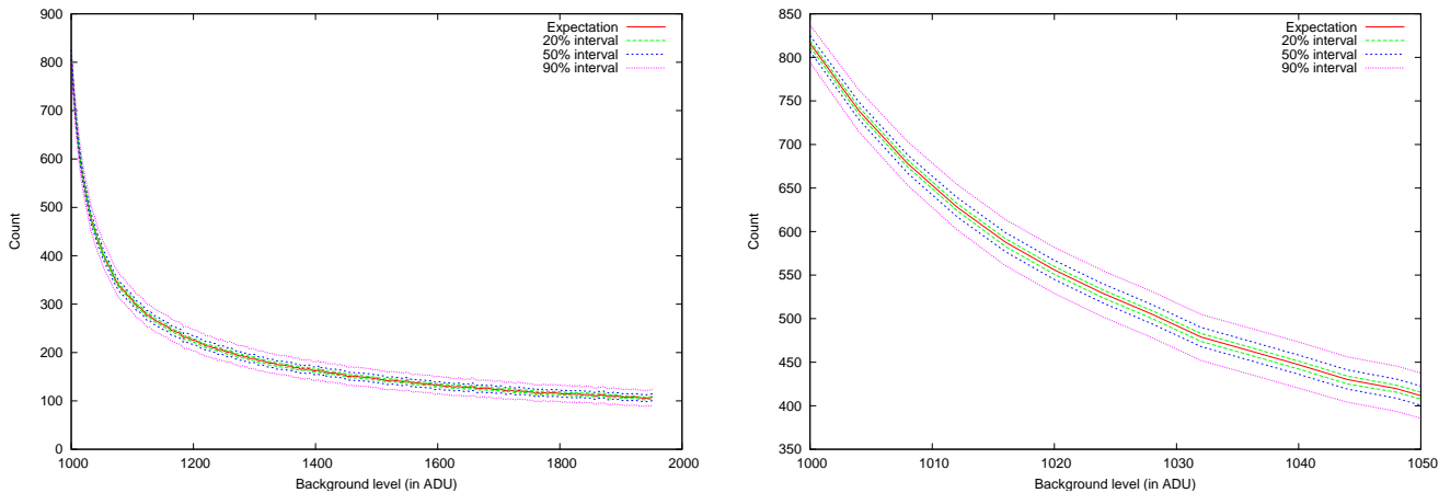
Figure 5.7: Thresholds for the reliability test at all levels accessible to the method (left) and close-up on the low backgrounds (right) for all possible 4-ADU bins. The expectation curve corresponds to: 1024 \cdot (\mathcal{P}(\tilde{S}_{ADU} = \frac{\lambda+4070}{4.07} - 2) + \mathcal{P}(\tilde{S}_{ADU} = \frac{\lambda+4070}{4.07} - 1) + \mathcal{P}(\tilde{S}_{ADU} = \frac{\lambda+4070}{4.07}) + \mathcal{P}(\tilde{S}_{ADU} = \frac{\lambda+4070}{4.07} + 1)) while the envelope curves limit the domains covering respectively 20, 50 and 90 % of realisations under the hypothesis \mathcal{H} .
