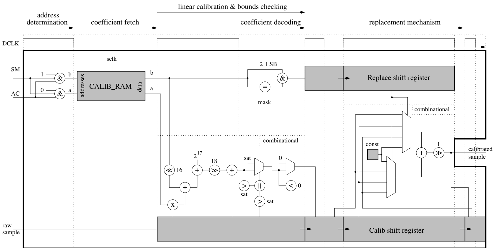
Figure 12.7: RTL representation of the Pre-calibration component and associated clocking (the logic introduced to round-off the equidistant cases ((11.23) and (11.24)) is not shown).
