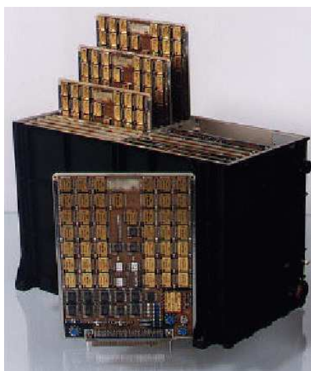
Figure 2.6: SSMM developed for Cluster (1994) by Astrium GmbH (courtesy of Astrium [30]).
