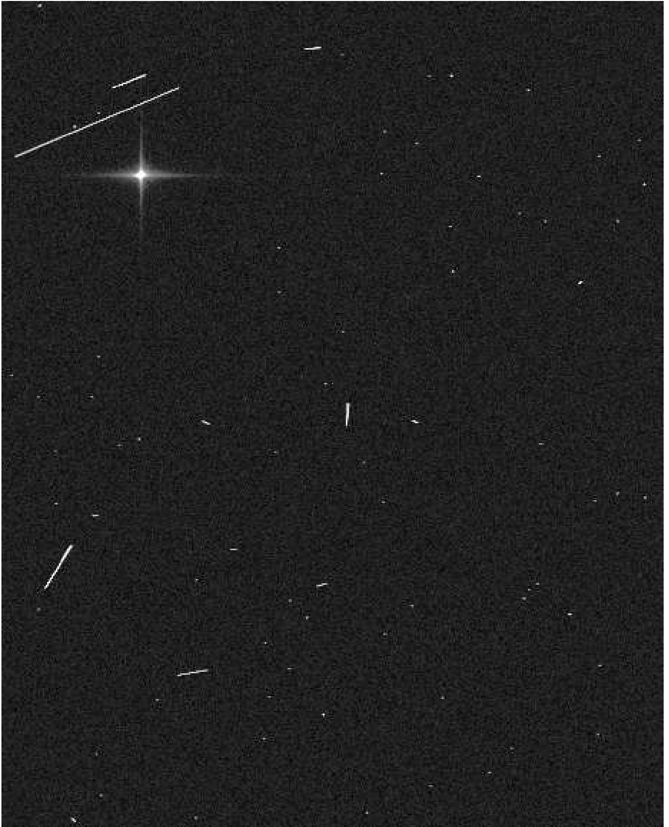
Figure C.1: The minimum density test case ( 3200 \text{ stars/deg}^2 ) at galactic coordinates l = 74 and b = 74 (close to the galactic pole). The snapshot is approximately 400 \text{ AL} \times 525 \text{ AC SM} samples.
