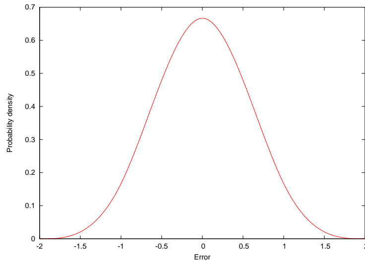
Figure 11.5: Distribution of numerical errors ( s\hat{u}m - sum ) for N = 2
