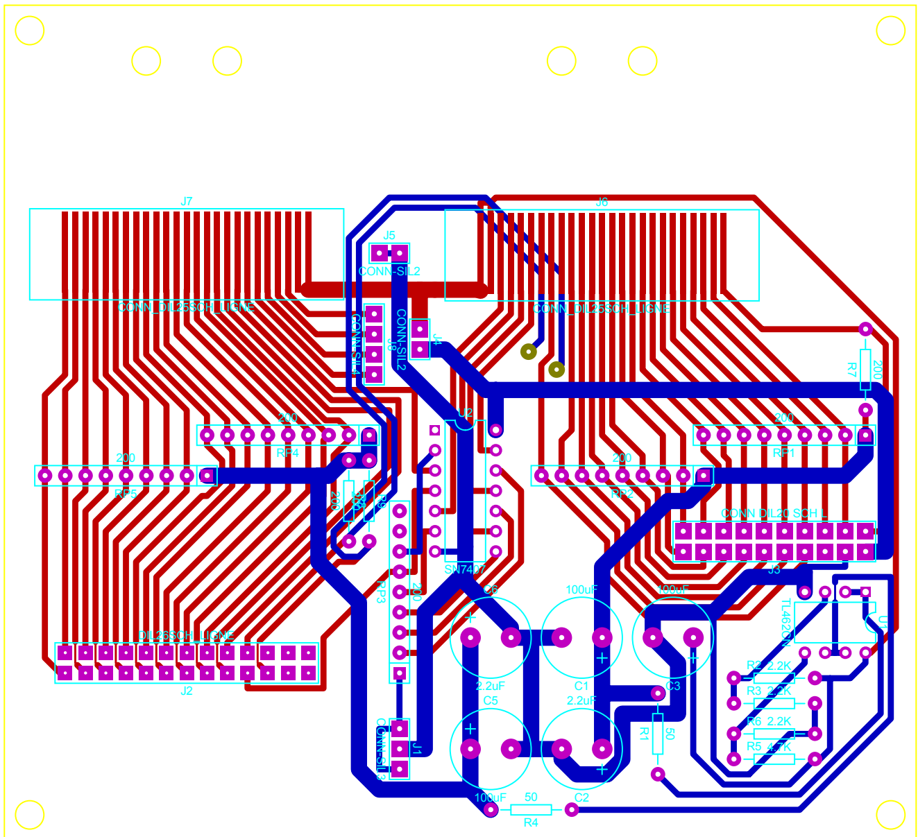
Figure A.4: Original layout of the PCB (C2) for the interface between the FPGA and the PC with its voltage adaptations and active terminations.
