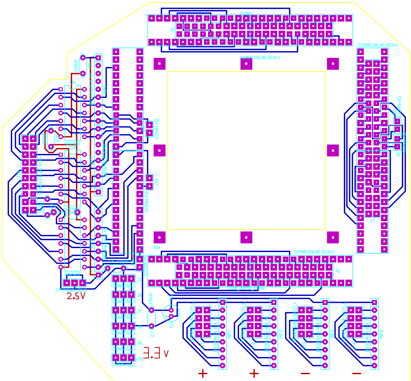
Figure A.2: Original layout of the intermediate PCB (C1) introduced between the FPGA and the SRAM and PC interface.
