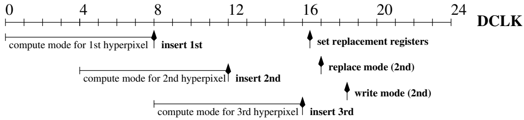
Figure 12.17: Replacement mechanism for unreliable mode values using adjacent hyperpixels. The indicated timescale is coherent with that of Fig. 12.16 and bold-faced operations are only carried out every four DCLK period.
