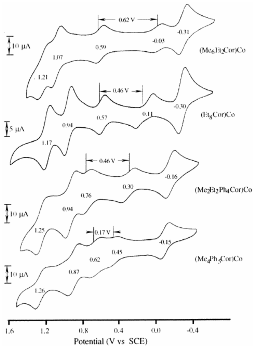
Figure 2-5. Cyclic voltammograms of 2.0 \times 10^{-3} M (\text{Me}_6\text{Et}_2\text{Cor})\text{Co} , 3.0 \times 10^{-3} M (\text{Et}_8\text{Cor})\text{Co} , 2.0 \times 10^{-3} M (\text{Me}_2\text{Et}_2\text{Ph}_4\text{Cor})\text{Co} , and 1.5 \times 10^{-3} M (\text{Me}_4\text{Ph}_5\text{Cor})\text{Co} in \text{CH}_2\text{Cl}_2 , 0.1 M TBAP. (Reproduced from ref. 108).
