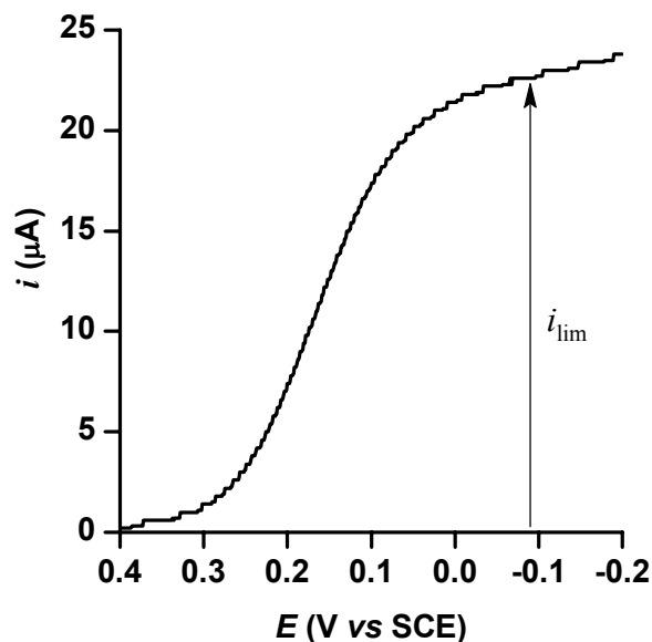
Figure 3-3. Current-potential curve for the reduction of O 2 in 1 M HClO 4 at a rotating graphite disk electrode coated with 2.4 \times 10^{-10} mol cm -2 of Co(TPP). Rotation rate: 100 rpm. Scan rate: 5 mV sec -1 .
