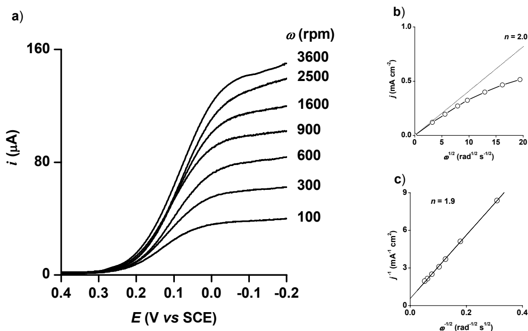
Figure 3-4. (a) Current-potential curves for the reduction of O_2 in 1 M HClO_4 at a rotating graphite disk electrode coated with 2.4 \times 10^{-10} mol cm^{-2} of Co(TPP) . Values of the rotational velocity ( \omega ) of the electrode in rpm are indicated on each curve. (b) Levich plot of the rotating limiting currents ( j ) vs square root of rotational velocity ( \omega ) 1/2 . The circle are experimental; the dotted line refers to the theoretical curve for the diffusion-convection-limited reduction of O_2 by two electrons, as indicated in the figure. (c) Koutecky-Levich plot of the reciprocal currents in part b vs ( \omega ) -1/2 .
