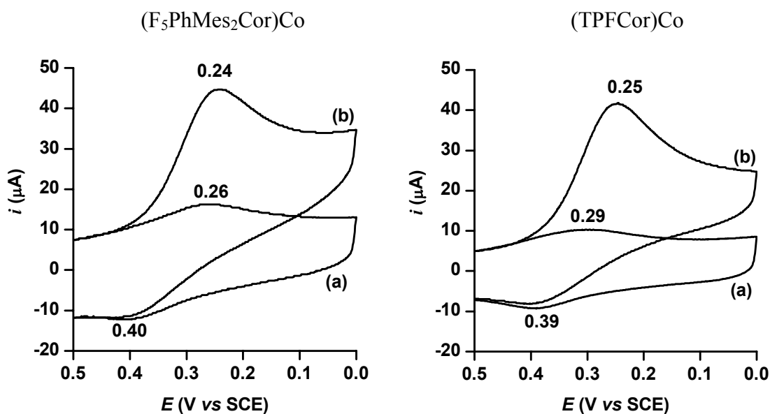
Figure 7-1. Cyclic voltammograms of cobalt corroles adsorbed on EPPG electrode. Supporting electrolyte: 1 M HClO_4 (a) saturated with argon and (b) saturated with air. Scan rate: 50 \text{ mV s}^{-1} .
