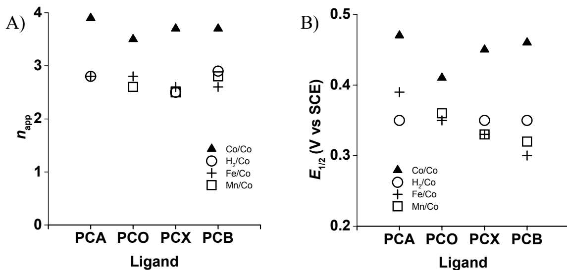
Figure 6-4. (A) apparent numbers of electrons transferred ( n_{app} ) vs Ligand and (B) Half-wave potentials ( E_{1/2} ) for O 2 reduction vs Ligand. (▲) (PCY)Co 2 , (○) (PCY)H 2 Co, (+) (PCY)FeClCoCl, (□) (PCY)MnClCoCl with Y = A, B, X or O.
