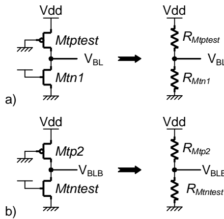
Figure II.1 – Principle of the DFD solution a) for the low level and b) for the high level
