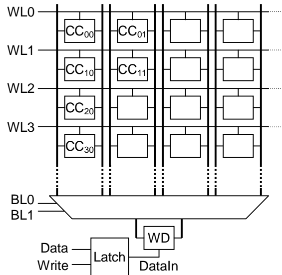
Figure I.12 – Basic view of a part of an SRAM array
