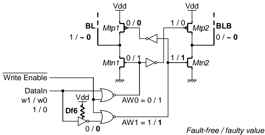
Figure I.11 – Faulty behavior of the write driver in presence of Df6
