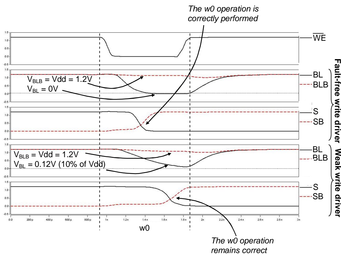
Figure II.1 – Fault-free and weak write driver operations
