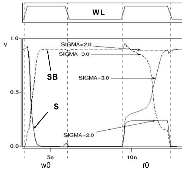
Figure I.39 – Read Destructive Fault (fs, 0.9V, 125°C – Mtn3 & Mtn2 )
