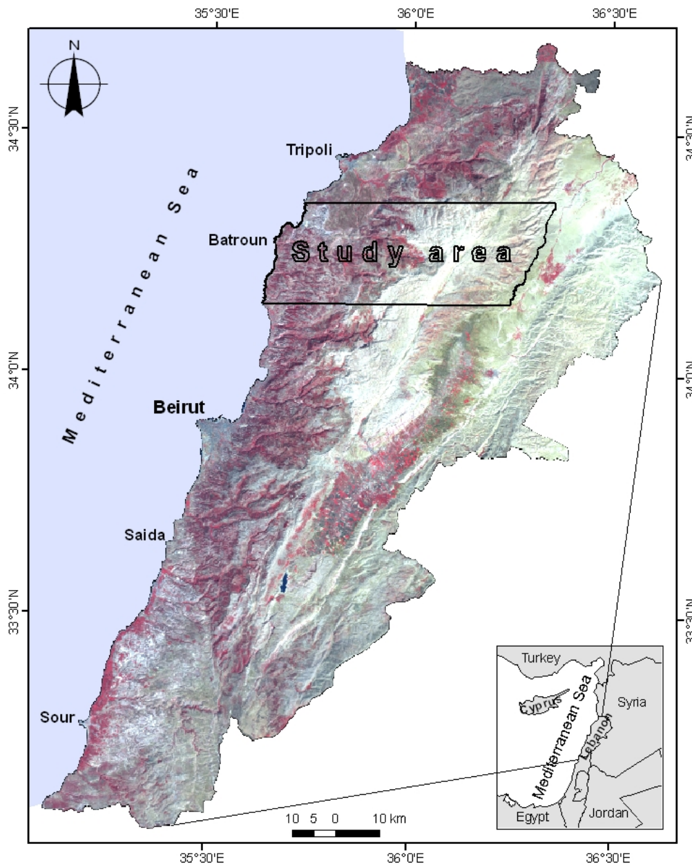
Figure 11. Location of the study area. (Background: Landsat image of 1989, band combination Red = 4, Green = 3 and Blue = 2).
