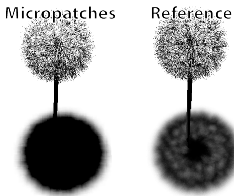
Fig. 10.22 : Gap-Filling Problem (Image by Bavoil et al. [BCS08])
