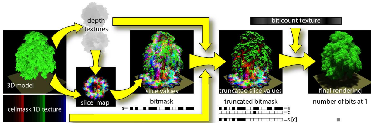
Fig. 8.2 : Overview of the transmittance shadow-map algorithm
