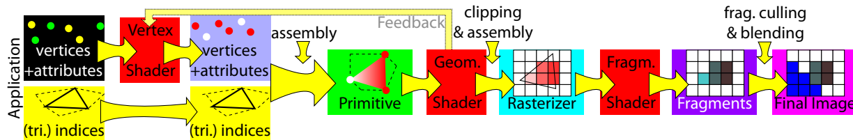
Fig. 2.2 : Graphics Pipeline
