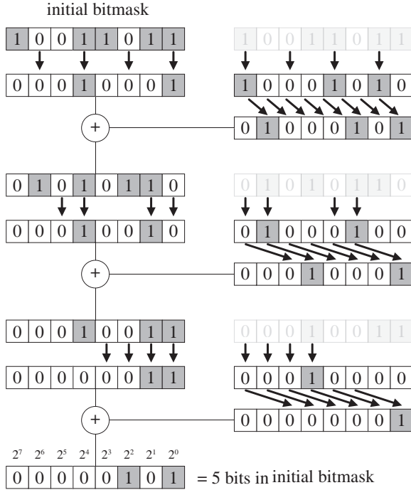
Fig. 8.3 : Logarithmic-Time Bit Counting
