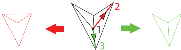
Fig. 4.8 : Triangle Flip - Merging vertex 1 and 2 gives an overlap, merging 1 and 3 is valid.
