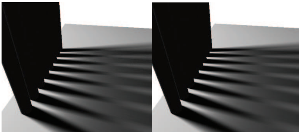
Fig. 13.13 : Shadow Quality
