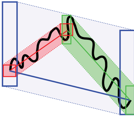
Fig. 4.7 : Conservative Estimate
