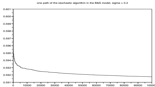
Figure 4.3: Path of the stochastic algorithm in the B&S model for the Partial Lookback put with \sigma = 0.2 .
