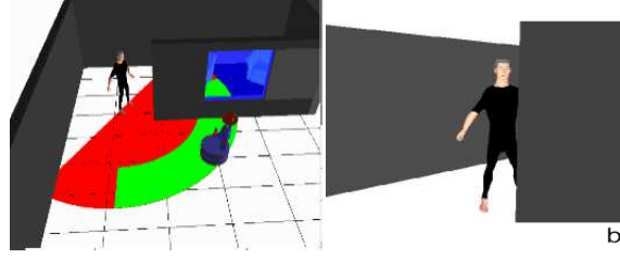
Figure 4.15: a) Robot positioned in the interaction area (Green). b) Robot's computed perception (2D projection)
