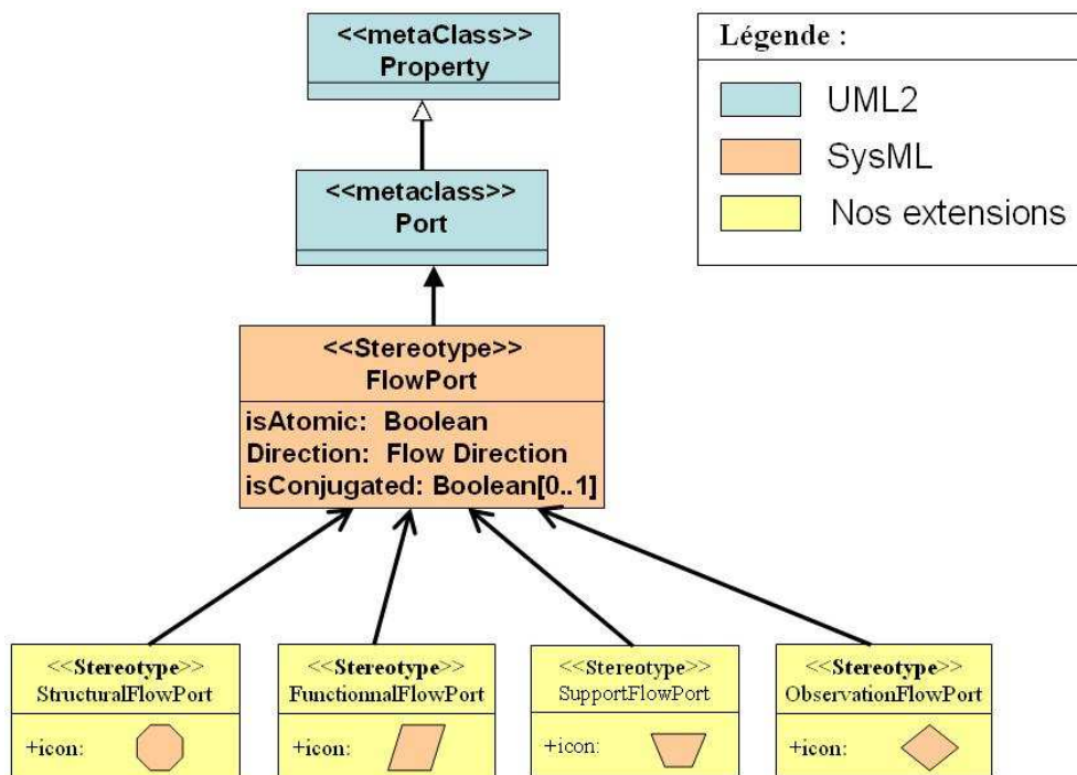
Figure 6.8. Stéréotypes du FlowPort SysML.
