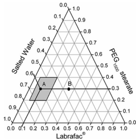
Figure 3. Ternary diagram allowing the determination of feasibility domain comprising nanocapsules with a size smaller than 150 nm and a polydispersity index inferior to 0.3. The composition A characterized by a water fraction F_w = 0.85 , led to the formation of nanocapsules with a size around 26 nm and a monomodal distribution. On the contrary, the formulation B composed of a lower water amount ( F_w = 0.5 ) was located outside of the feasibility domain.
