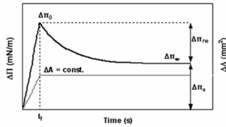
Figure 2. Fast compression and relaxation profile at constant area
