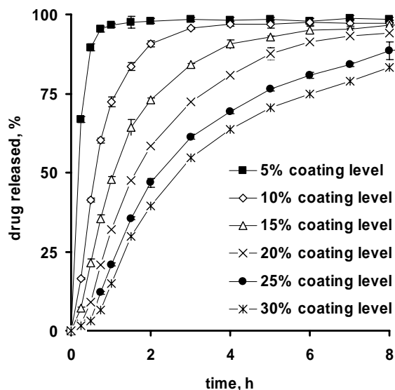
Figure 5.7: Importance of the coating level (indicated in the diagram) on drug release from diltiazem HCl layered sugar cores coated with ethylcellulose:PVA-PEG-graft-copolymer 90:10 in 0.1 N HCl (plasticizer: TEC, drug loading of the diltiazem HCl layered sugar cores: 10 %).
