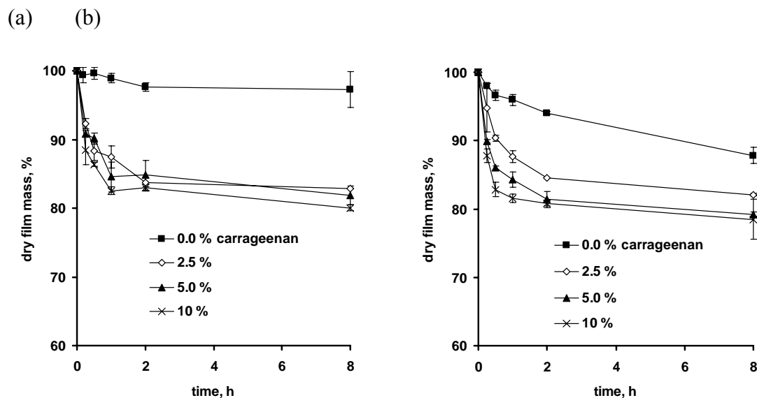
Figure 3.4: Effects of the addition of small amounts of carrageenan (indicated in the figures) on the dry mass loss of ethylcellulose-based films upon exposure to: (a) 0.1 N HCl; (b) phosphate buffer pH 7.4.
