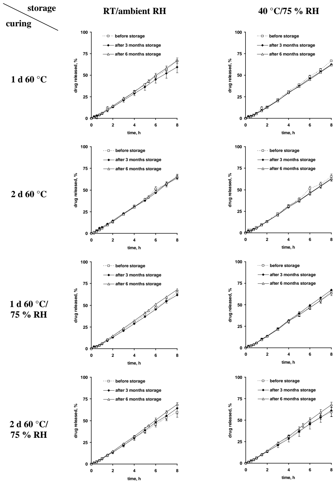
Figure 4.1: Storage stability of pellets coated with 85:15 ethylcellulose:PVA-PEG graft copolymer: Theophylline release in 0.1 N HCl before (dotted lines) and after 3 and 6 months
