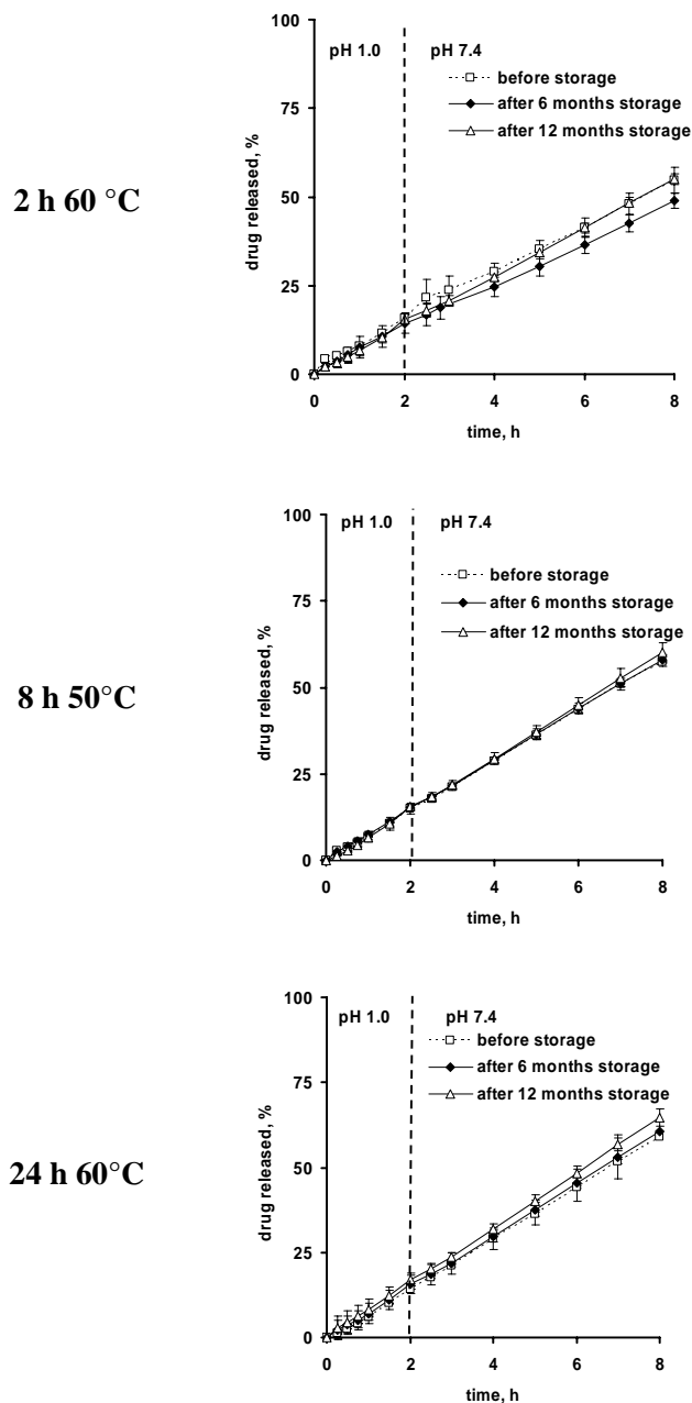
Figure 8.6: Storage stability of ethylcellulose:PVA-PEG graft copolymer 85:15 coated theophylline matrix cores cured under different conditions (indicated in the figure) before and after 12 months open storage under ambient conditions (coating level: 15 %): Drug release in 0.1 M HCl for 2 h, followed by phosphate buffer pH 7.4.
