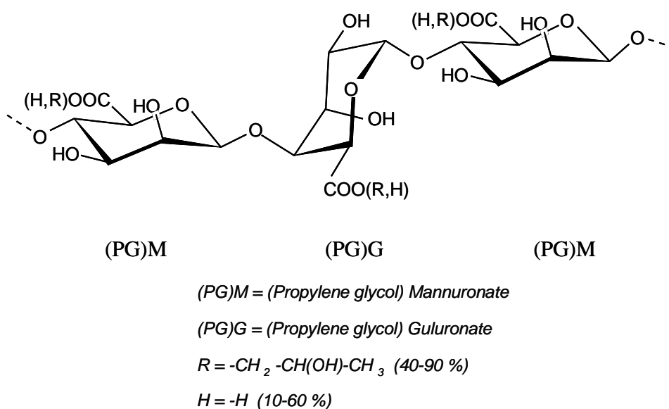
Figure 1.6: Chemical structure of PG alginate.
