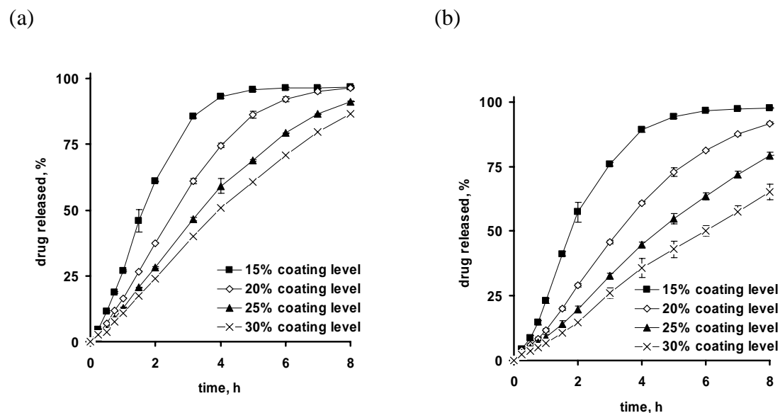
Figure 7.4: Effects of the coating level on theophylline release in 0.1 N HCl from pellets coated with ethylcellulose:PVA-PEG graft copolymer 90:10, containing: (a) drug layered sugar cores, and (b) drug layered MCC cores.
