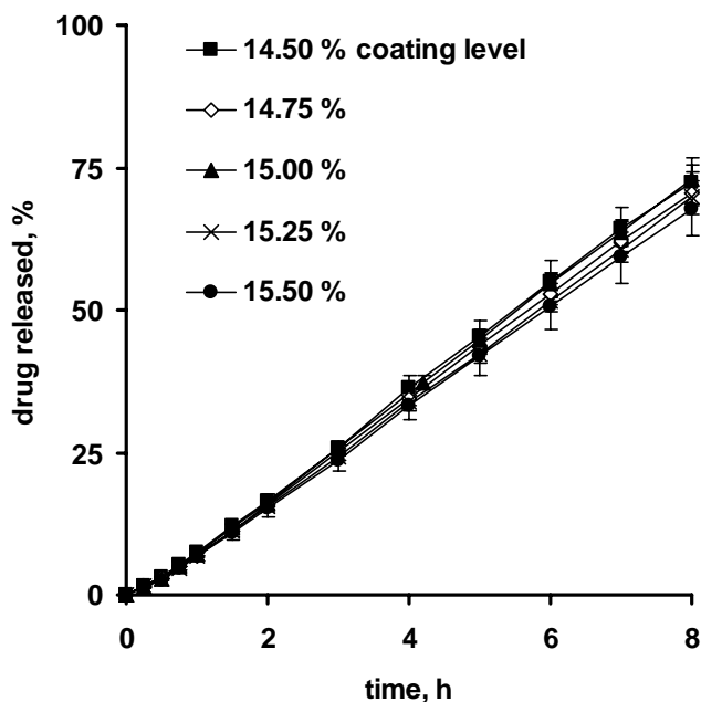
Figure 4.8: Robustness of the coating process with ethylcellulose:PVA-PEG graft copolymer blends: Effects of slight variations in the coating level (indicated in the diagrams) on theophylline release in 0.1 N HCl (polymer blend ratio = 85:15; curing = 1 d 60 °C).
