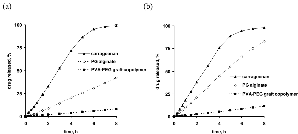
Figure 3.8: Importance of the type of additive (indicated in the figures) on theophylline release from pellets coated with ethylcellulose containing 10 % carrageenan, PG alginate or PVA-PEG graft copolymer upon exposure to: (a) 0.1 N HCl; (b) phosphate buffer pH 7.4 [20 % coating level; curing = 1 d at 60° C & ambient RH] (the results obtained with PVA-PEG graft copolymer and PG alginate are reproduced from [18] for reasons of comparison).
