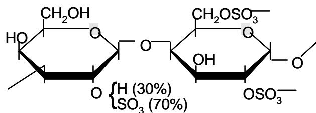
Figure 1.5: Chemical structure of \lambda -Carrageenan.
