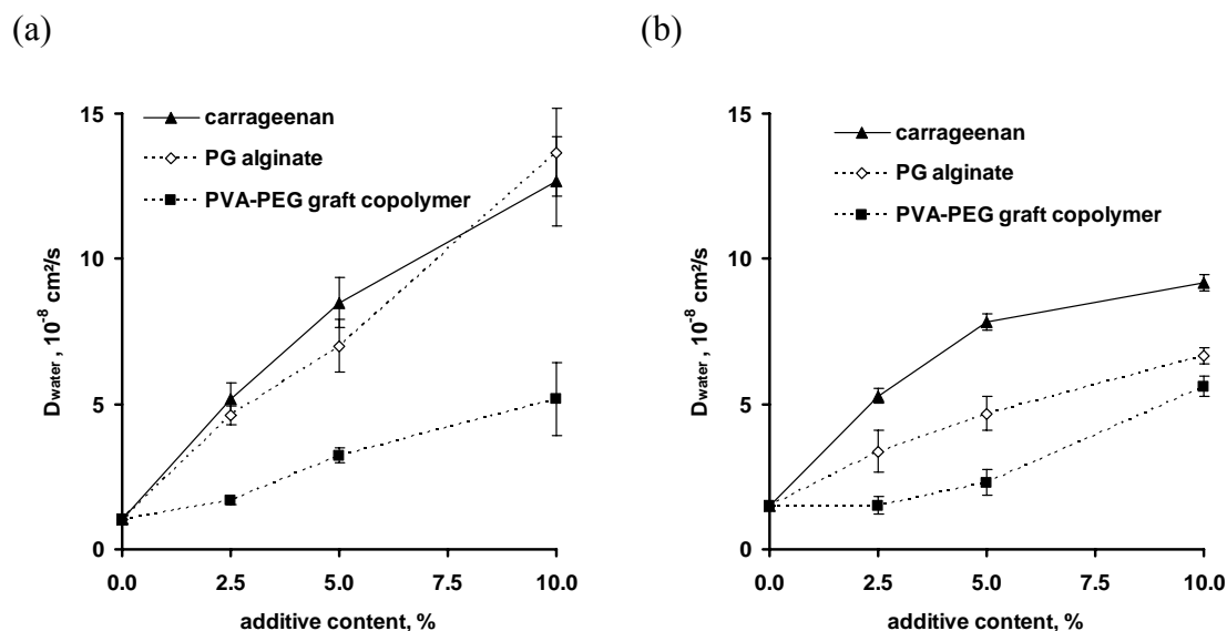
Figure 3.3: Water diffusivity in ethylcellulose-based films upon exposure to: (a) 0.1 N HCl; (b) phosphate buffer pH 7.4: Effects of the type and amount of additive (the results obtained with PG alginate and PVA-PEG graft copolymer are reproduced from [18] for reasons of comparison).
