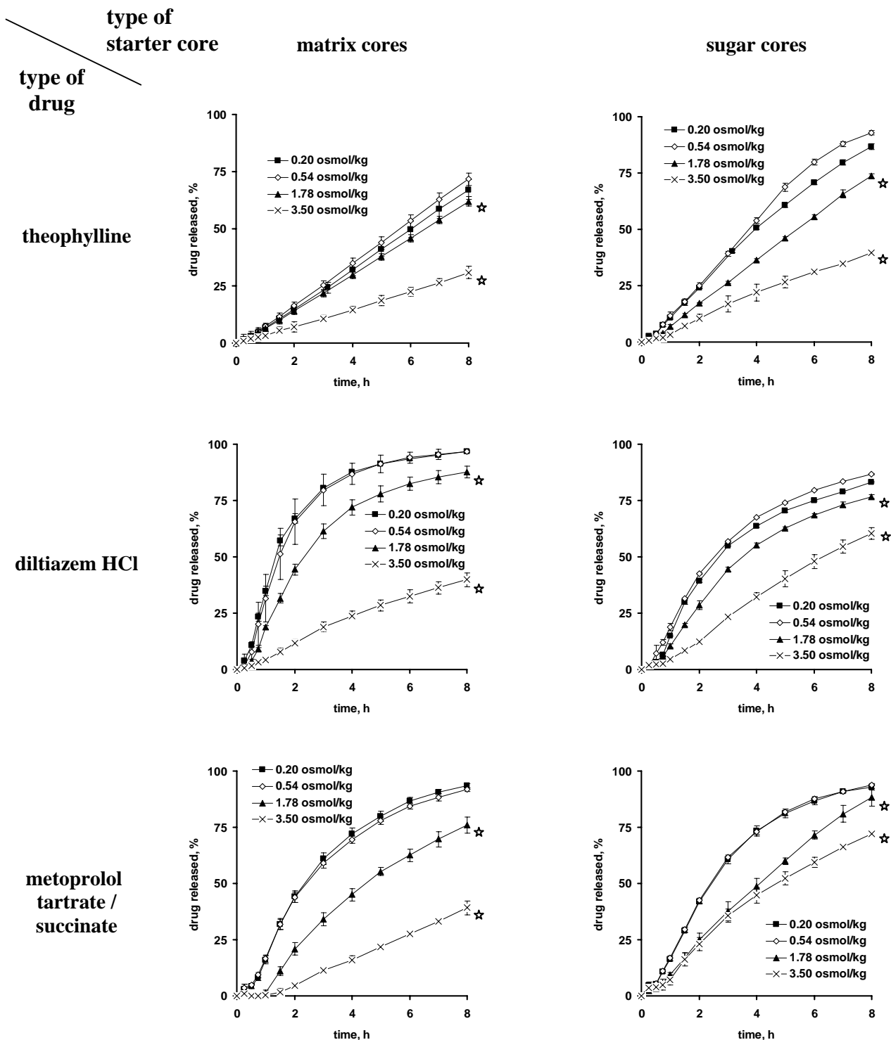
Figure 7.3: Importance of the osmotic pressure of the release medium for drug release from pellets coated with ethylcellulose:PVA-PEG graft copolymer containing different types of cores (as indicated on the top) loaded with different types of drugs (as indicated on the left) in 0.1 N HCl containing different amounts of NaCl (stars indicate non-physiological
