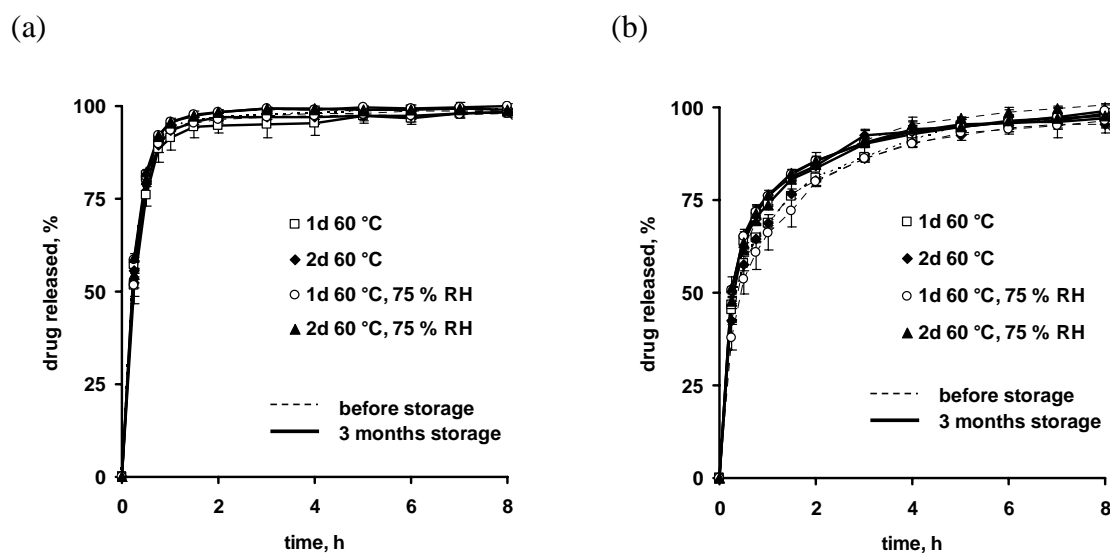
Figure 8.3: Diltiazem HCl release from drug layered sugar cores coated with ethylcellulose:PVA-PEG graft copolymer 85:15 before and after 3 months storage at 40 °C and 75 % relative humidity in: (a) 0.1 N HCl and (b) phosphate buffer pH 7.4 (curing conditions as indicated in the figures; drug loading: 10%; coating level: 15 %).
