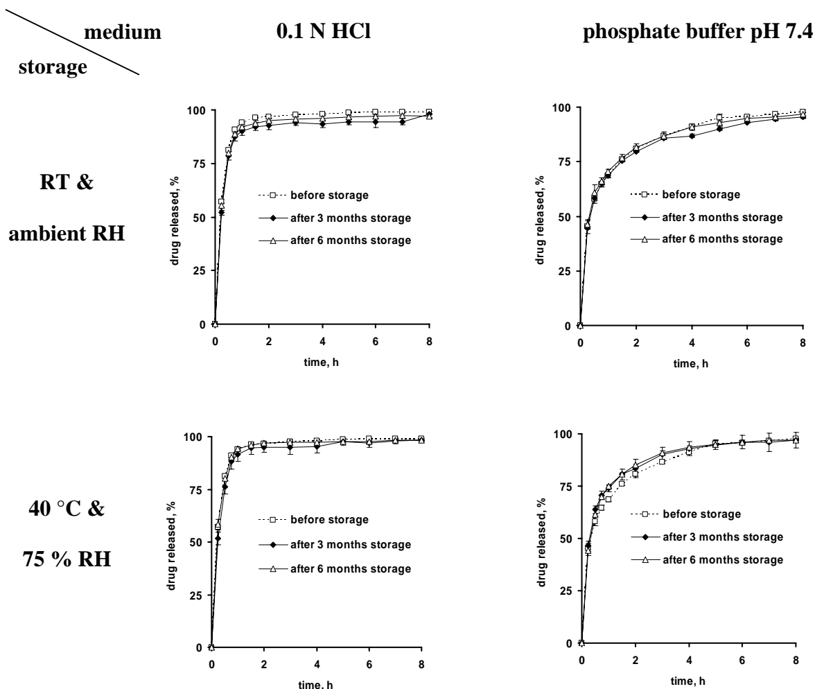
Figure 5.1: Drug release from diltiazem HCl layered sugar cores coated with ethylcellulose:PVA-PEG-graft-copolymer 85:15 before (dotted lines) and after 3 and 6 months storage (full lines, as indicated). The release media are shown at the top and the storage conditions on the left (coating level: 15 %, plasticizer: TEC, drug loading of the diltiazem HCl layered sugar cores: 10 %).
