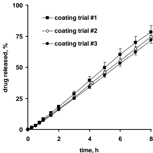
Figure 4.7: Reproducibility of the coating process with ethylcellulose:PVA-PEG graft copolymer 85:15 blends: Theophylline release in 0.1 N HCl from pellets coated in three different trials (the number is indicated in the diagrams) (coating level = 15 %; curing = 1 d 60 °C).
