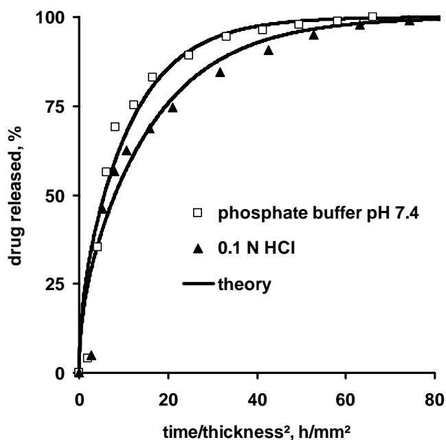
Figure 6.7: Diltiazem HCl release from thin polymeric films based on ethylcellulose:PVA-PEG graft copolymer 90:10 in 0.1 N HCl and phosphate buffer pH 7.4: Experiments (symbols) and theory (curves, Equations 6.7-6.9). Please note that the time plotted on the x-axis is normalized to the thickness of the films in order to account for slight, arbitrary variations of the latter. Each experiment was conducted in triplicate, but only one representative example is shown for each release medium.
