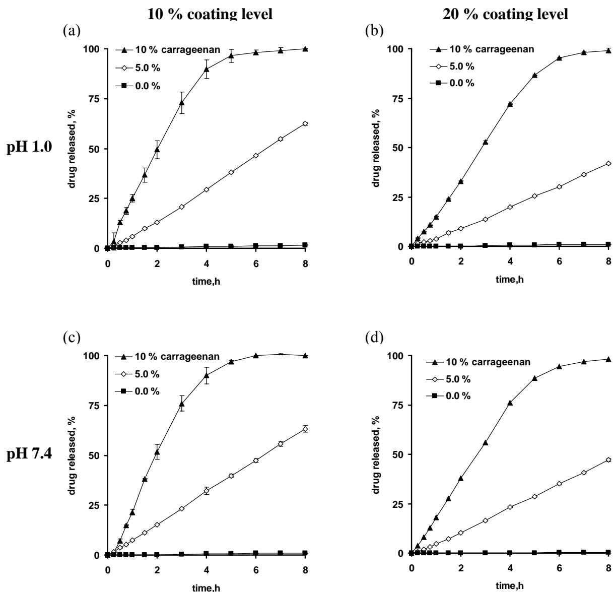
Figure 3.7: Theophylline release from pellets coated with ethylcellulose containing small amounts of carrageenan (indicated in the figures) upon exposure to: (a) 0.1 N HCl, 10% coating level; (b) 0.1 N HCl, 20% coating level; (c) phosphate buffer pH 7.4, 10% coating level; (d) phosphate buffer pH 7.4, 20% coating level (curing = 1 d at 60° C & ambient RH).
