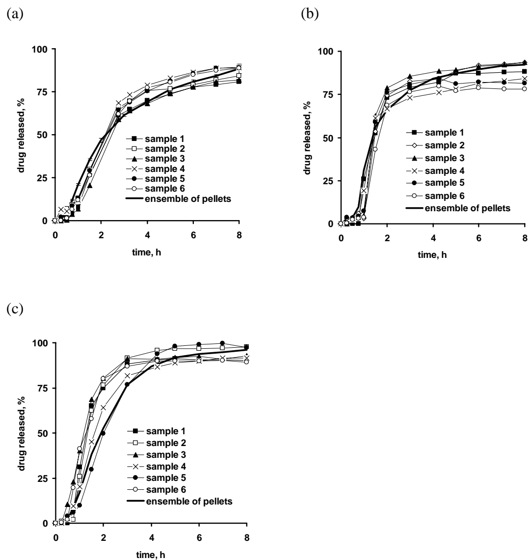
Figure 6.4: Drug release from single pellets coated with ethylcellulose:PVA-PEG graft copolymer 90:10 in 0.1 N HCl, containing: (a) sugar cores, (b) MCC cores and (c) sealed sugar cores (coating level: 25 %). For reasons of comparison also drug release from ensembles of pellets is shown.
