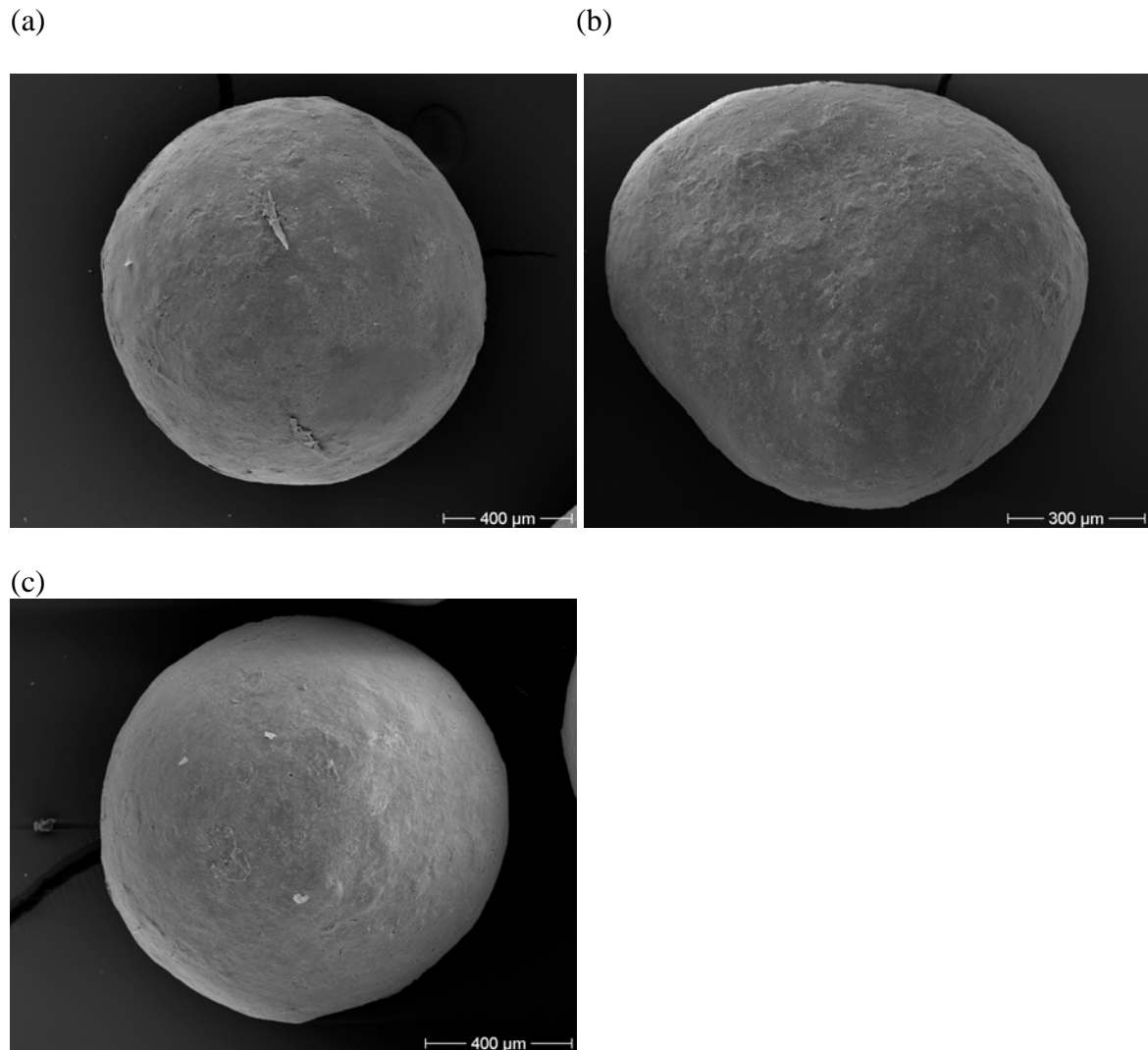
Figure 6.6: Scanning electron microscopy pictures of pellets coated with ethylcellulose:PVA-PEG graft copolymer 90:10, containing: (a) sugar cores, (b) MCC cores and (c) sealed sugar cores after 2 h exposure to 0.1 N HCl (coating level: 30 % in the case of sugar and MCC cores, 25 % in the case of sealed sugar cores).
