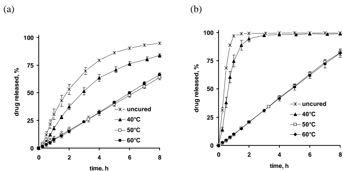
Figure 8.4: Influence of the curing temperature (indicated in the figures) on theophylline release from ethylcellulose:PVA-PEG graft copolymer 85:15 coated drug matrix cores in: (a) 0.1 N HCl and (b) phosphate buffer pH 7.4 (curing time: 24 h, coating level: 15 %).
