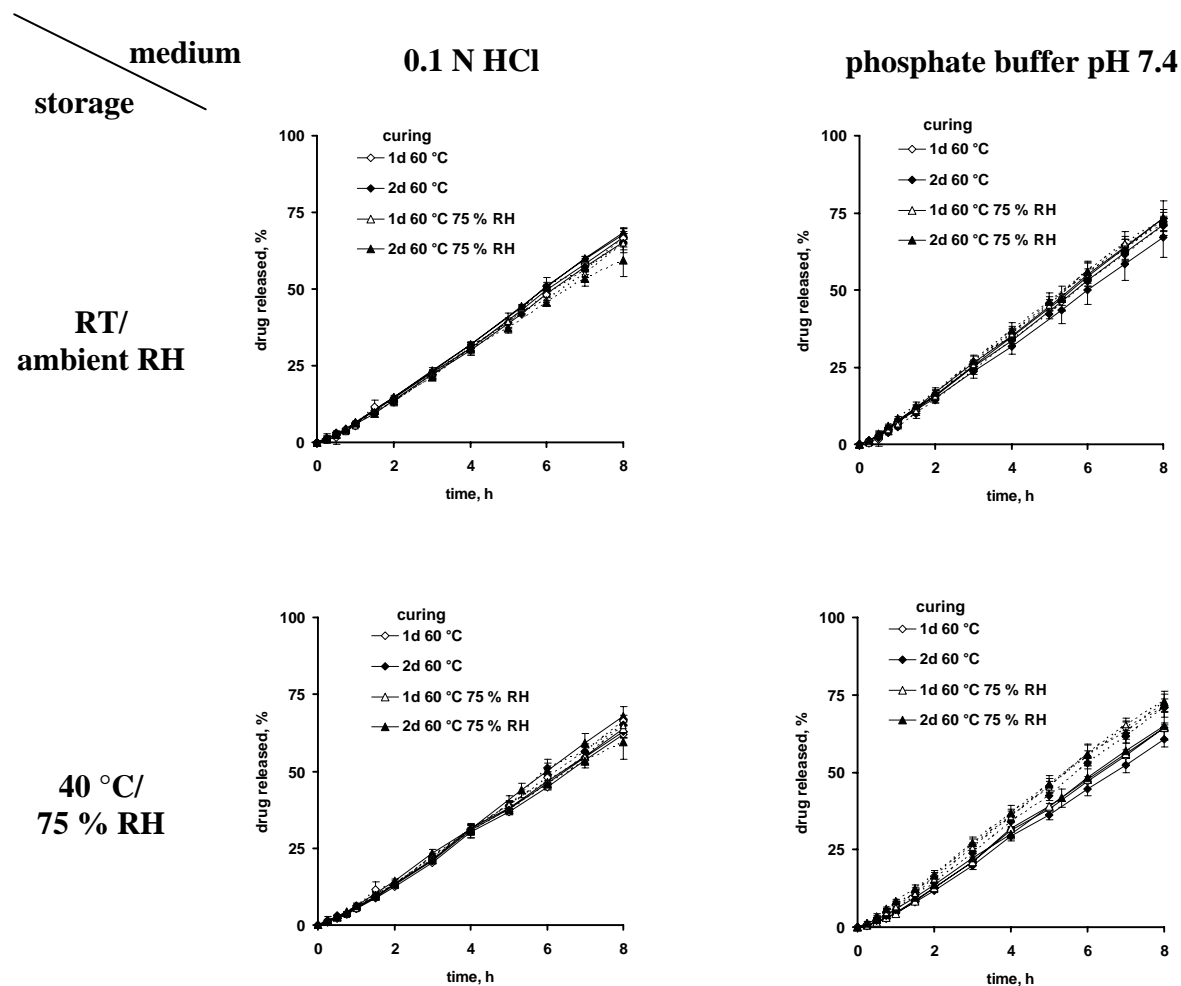
Figure 4.2: Effects of the curing conditions (indicated in the diagrams) on theophylline release from pellets coated with 85:15 ethylcellulose:PVA-PEG graft copolymer before (dotted lines) and after 6 months open storage (full lines) at different temperatures and relative humidities (as indicated on the left) in 0.1 N HCl or phosphate buffer pH 7.4 (as indicated at the top) (coating level = 20 %).
