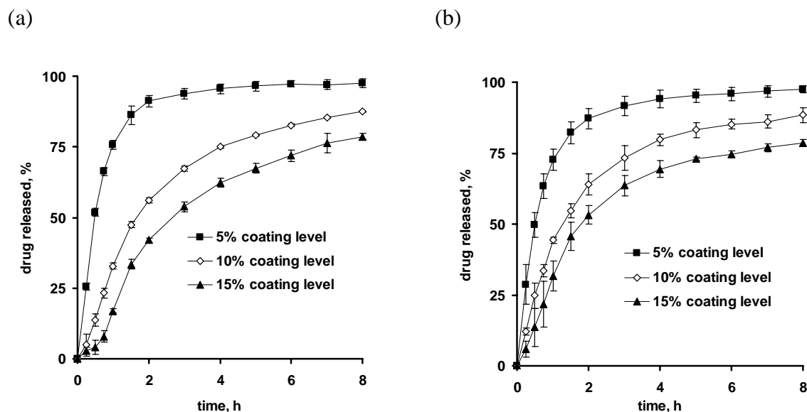
Figure 5.3: Effects of the coating level (indicated in the diagrams) on drug release from ethylcellulose:PVA-PEG-graft-copolymer 95:05 coated diltiazem HCl layered sugar cores in: (a) 0.1 N HCl and (b) phosphate buffer pH 7.4 (plasticizer: TEC, drug loading of the diltiazem HCl layered sugar cores: 10 %).
