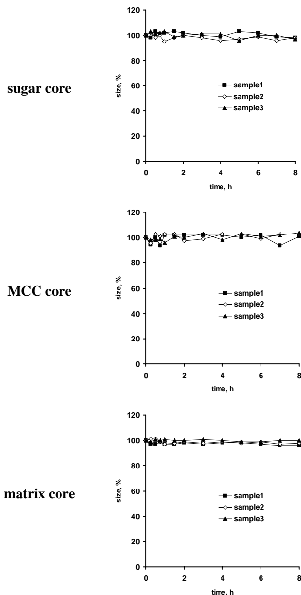
Figure 7.5: Swelling behaviour of theophylline loaded pellets containing different types of starter cores (indicated in the figure), coated with ethylcellulose:PVA-PEG graft copolymer upon exposure to 0.1 N HCl (sugar and MCC cores: polymer polymer blend ratio = 90:10; matrix cores: polymer:polymer blend ratio = 85:15) (coating level = 30 %, single pellets).
