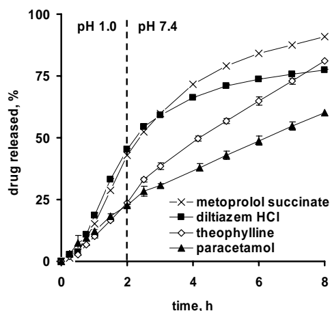
Figure 7.1 Effects of the type of drug (indicated in the figures) on the release patterns from pellets coated with ethylcellulose:PVA-PEG graft copolymer 90:10 in: (a) 0.1 N HCl for 8 h, and (b) 0.1 N HCl for 2 h and subsequent complete medium change to phosphate buffer pH 7.4 (coating level: 30 %, drug layered sugar cores).
