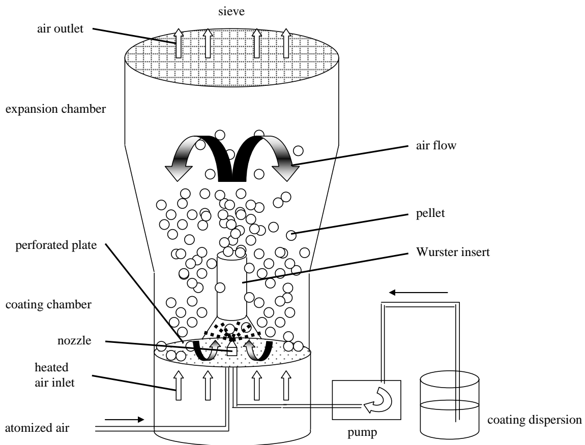
Figure 1.1: Schematic presentation of a fluidized bed coater with Wurster insert.
