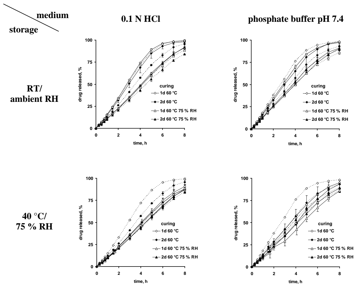
Figure 4.6: Importance of the curing conditions (indicated in the diagrams) for theophylline release from pellets coated with ethylcellulose:carrageenan 90:10 blends before (dotted curves) and after 6 months storage (full curves) at different temperatures and relative humidities (as indicated on the left) in 0.1 N HCl and phosphate buffer pH 7.4 (as indicated at the top) (coating level = 20 %).
