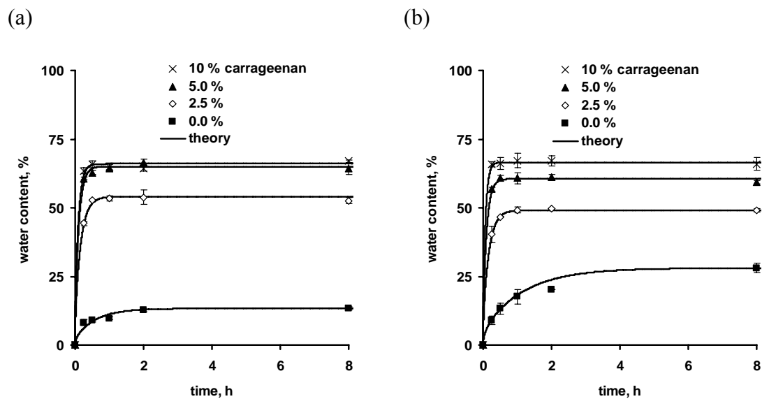
Figure 3.2: Water uptake behavior of ethylcellulose-based films containing different amounts of carrageenan (indicated in the figures) upon exposure to: (a) 0.1 N HCl; (b) phosphate buffer pH 7.4. The symbols represent the experimentally measured values, the curves the fitted theory (Equation 3.6).
