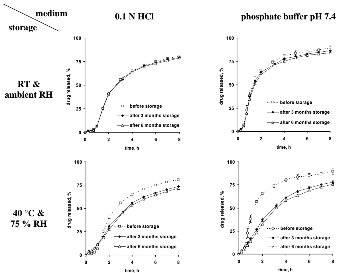
Figure 5.6: Drug release from diltiazem HCl layered sugar cores coated with ethylcellulose:PVA-PEG-graft-copolymer 95:5, plasticized with DBS, before (dotted lines) and after 3 and 6 months storage (full lines, as indicated). The release media are shown at the top, the storage conditions on the left (coating level: 15 %, drug loading of the diltiazem HCl layered sugar cores: 10 %).
