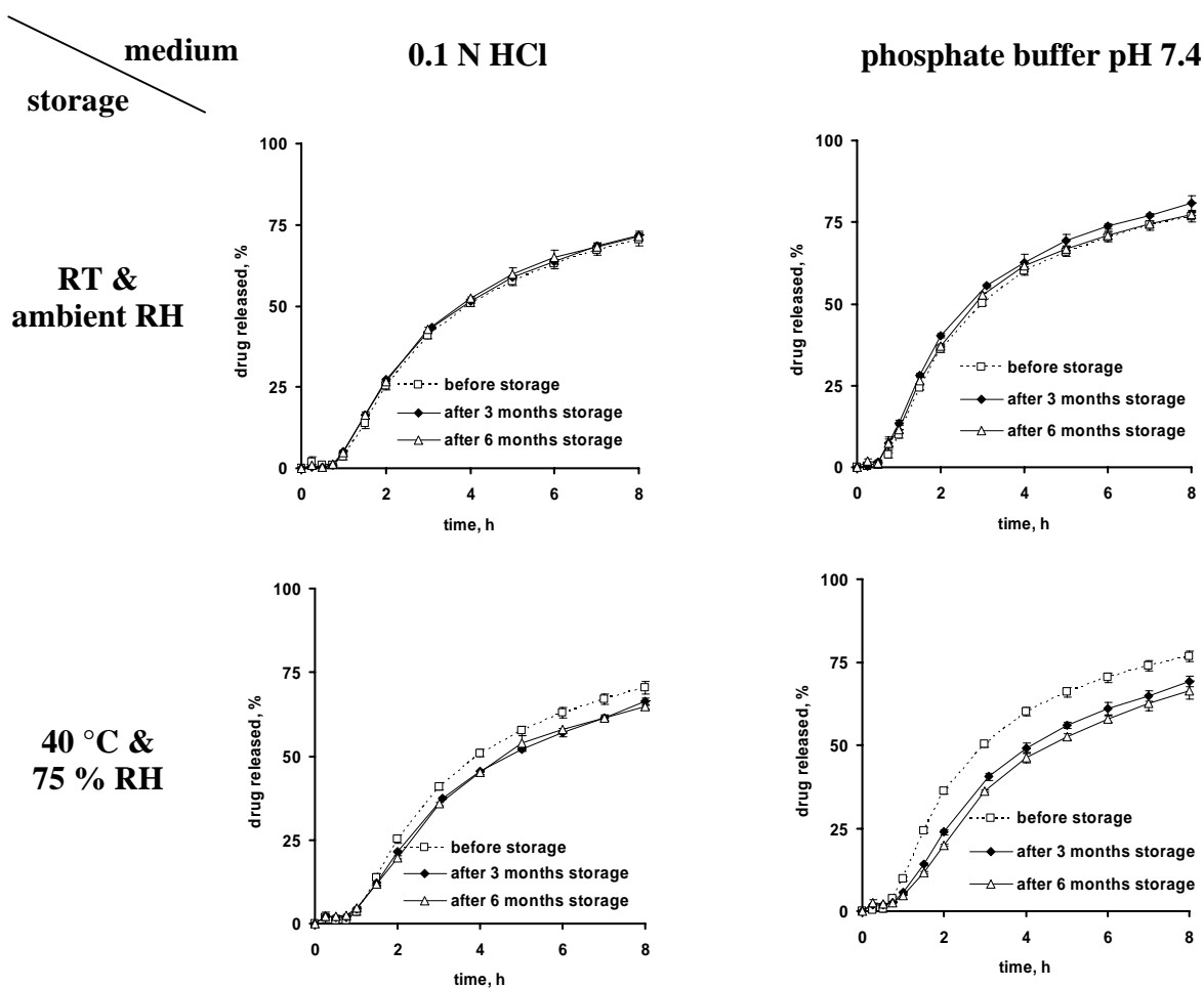
Figure 5.5: Drug release from diltiazem HCl layered sugar cores coated with ethylcellulose:PVA-PEG-graft-copolymer 95:5 before (dotted lines) and after 3 and 6 months storage (full lines, as indicated). The release media are shown at the top, the storage conditions on the left (coating level: 15 %, plasticizer: TEC, drug loading of the diltiazem HCl layered sugar cores: 20 %).
