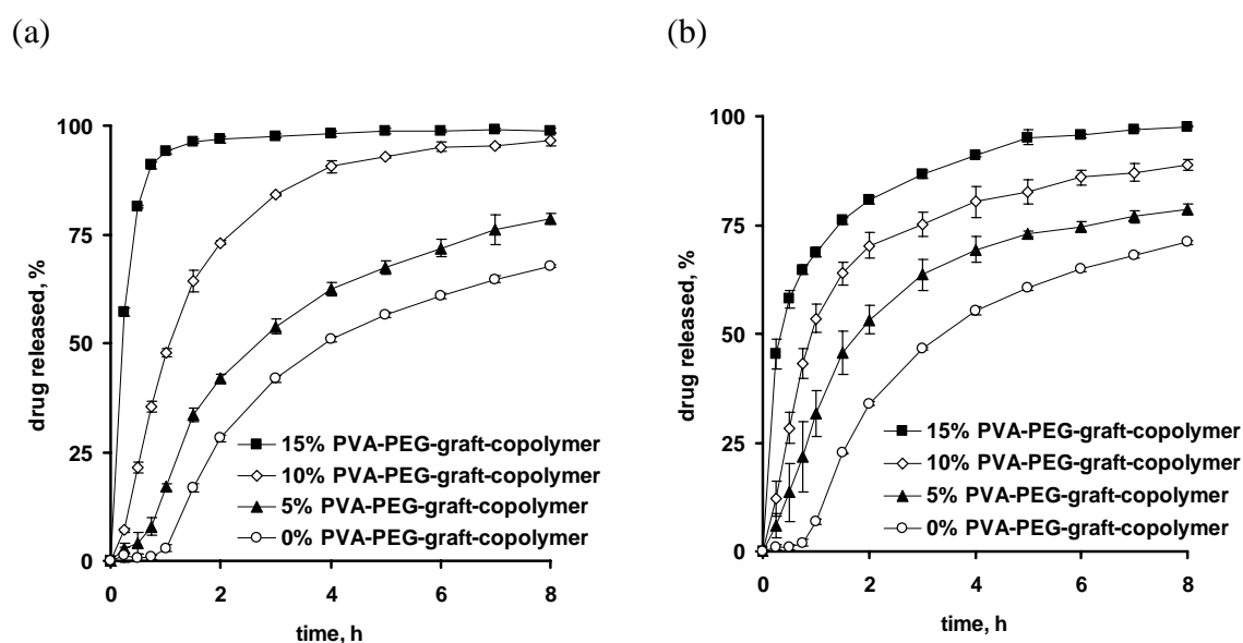
Figure 5.2: Effects of the PVA-PEG graft-copolymer content (indicated in the diagrams) in the ethylcellulose-based film coatings on drug release in: (a) 0.1 N HCl and (b) phosphate buffer pH 7.4 (coating level: 15 %, plasticizer: TEC, drug loading of the diltiazem HCl layered sugar cores: 10 %).
