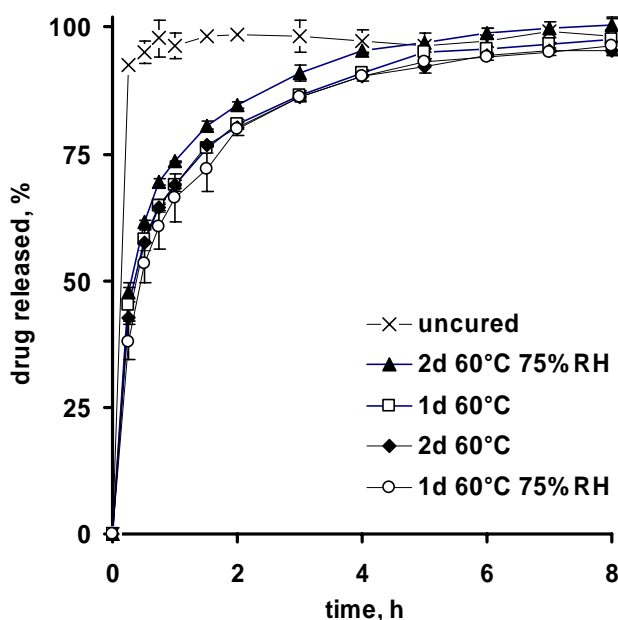
Figure 8.1: Influence of curing conditions (indicated in the figure) on drug release from diltiazem HCl layered sugar cores coated with ethylcellulose:PVA-PEG graft copolymer 85:15 in phosphate buffer pH 7.4 (drug loading: 10%; coating level: 15 %).
