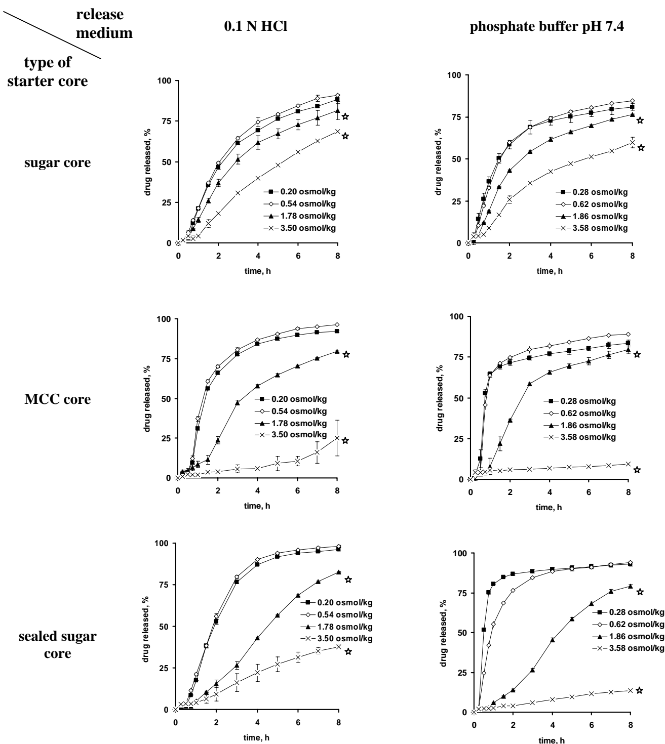
Figure 6.3: Impact of the osmolality of the release medium (indicated in the figures) on drug release from different types of diltiazem HCl layered starter cores coated with ethylcellulose:PVA-PEG graft copolymer 90:10. The release media are shown at the top, the type of cores is indicated on the left (coating level: 25 %, the stars indicate non-physiological conditions).
