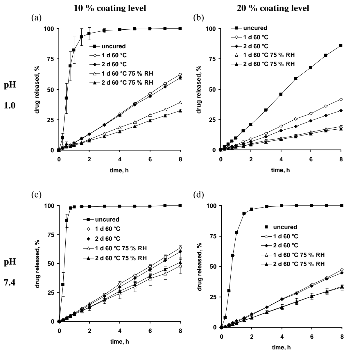
Figure 3.9: Effects of the curing conditions (indicated in the figures) on theophylline release from pellets coated with ethylcellulose containing 5 % carrageenan upon exposure to: (a) 0.1 N HCl, 10 % coating level; (b) 0.1 N HCl, 20 % coating level; (c) phosphate buffer pH 7.4, 10 % coating level; (d) phosphate buffer pH 7.4, 20 % coating level.
