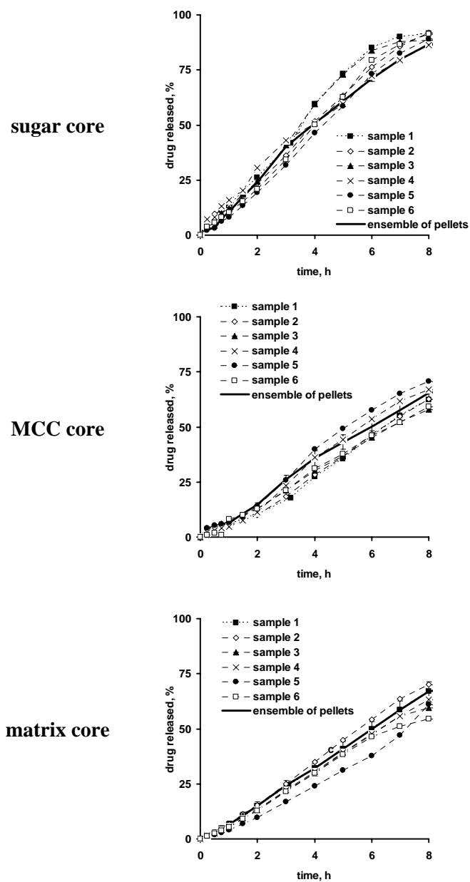
Figure 7.7: Theophylline release from single pellets in 0.1 N HCl from drug layered sugar and MCC cores, coated with ethylcellulose:PVA-PEG graft copolymer 90:10 (coating level: 30 %) as well as from drug matrix cores, coated with ethylcellulose:PVA-PEG graft copolymer 85:15 (coating level: 15 %). For reasons of comparison also drug release from ensembles of pellets is shown.
