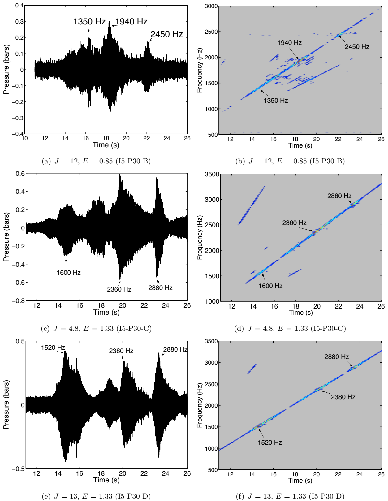
Fig. III.11: Pressure signals and short Time Fourier transform analysis for a linear frequency sweep. The data correspond to three different operating points I5-P30-B, I5-P30-C and I5-P30-D.
