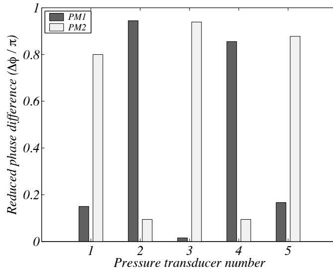
Fig. II.19: Reduced phase difference between the two PM and the five pressure transducers at the modulation frequency (2345 Hz).
