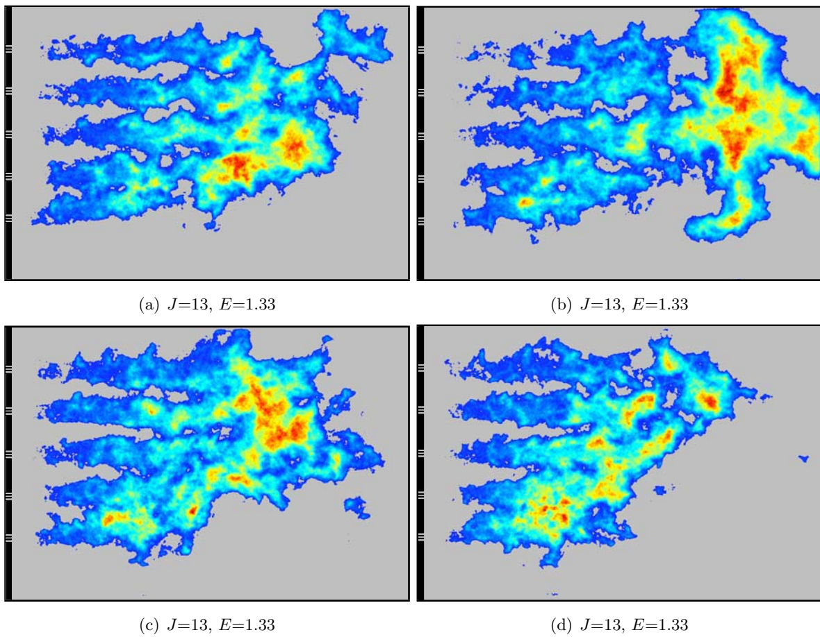
Fig. III.17: Set of four instantaneous OH* emission images for the operating point I5-P30-D modulated 2380 Hz.
