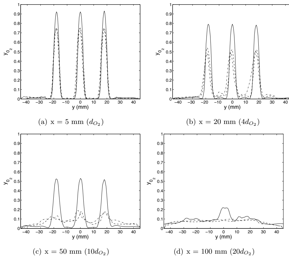
Fig. IV.10: Oxygen mass fraction in different transverse sections. The plot shows natural (continuous line), 1 \text{ m s}^{-1} modulated (dashed line) and 3 \text{ m s}^{-1} modulated (dot-dashed line) cases.
