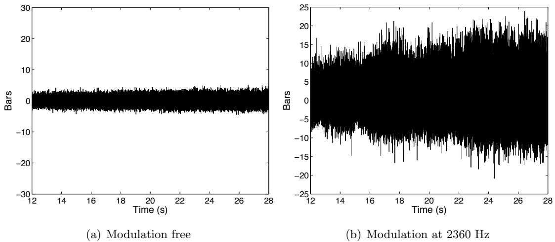
Fig. III.21: Pressure signal in the liquid oxygen cavity, feeding simultaneously the five elements, without (a) and with external modulation applied in the main combustion chamber at 2360 Hz.
