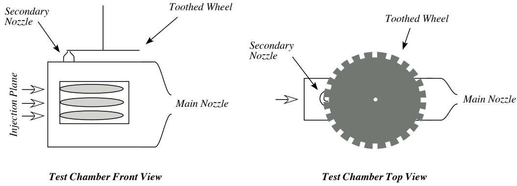
Fig. I.11: Lateral and top schematic views of the test chamber equipped with the toothed wheel modulator (TWM).
