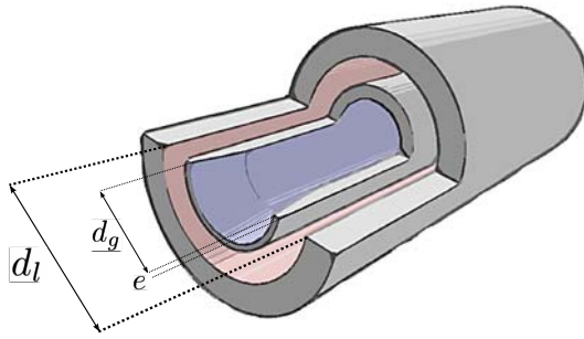
Fig. I.7: Geometrical characteristics of a typical injector used in the low pressure ( p = 1 MPa) experiments.
