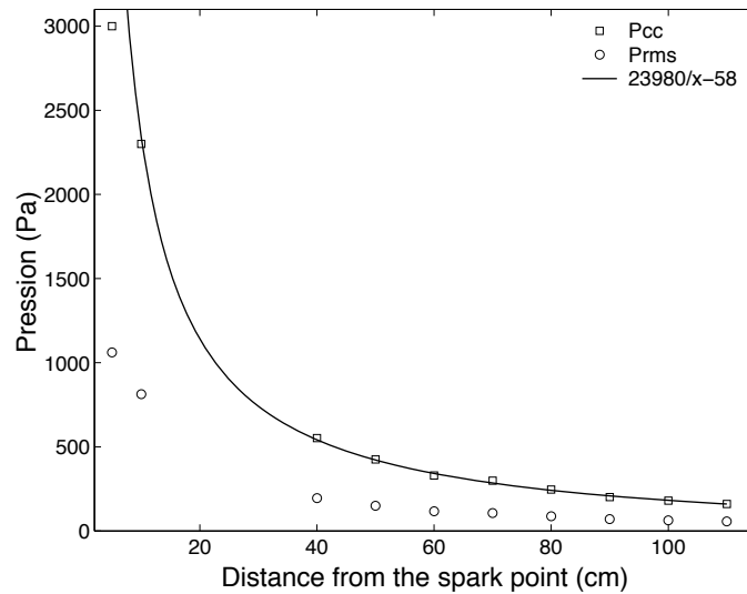
Fig. 1.17: Peak intensity of the pressure wave generated by a focused laser beam as a function of distance from the spark. □ Peak to peak pressure, ○ Root mean square pressure, - hyperbolic curve fit.
