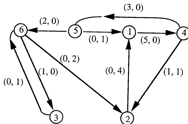
Figure V.4 Solution du biflot.
