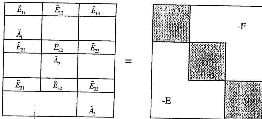
Figure II.6 Forme bloc-diagonale de la base optimale.
