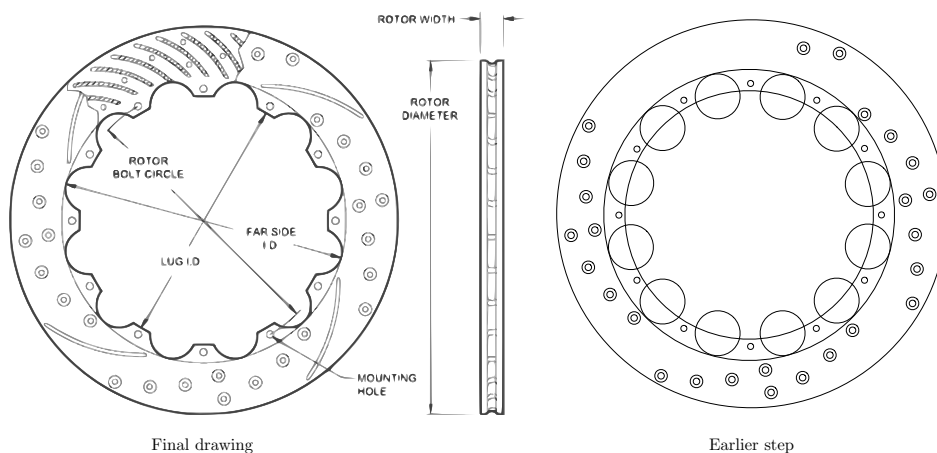
Figure 3.1: Modeling of a disc brake rotor: final drawing and earlier step.
