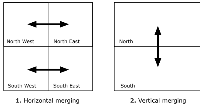
Figure 4.6: Merging schema.
