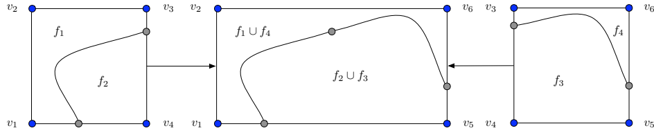
Figure 4.5: Fusion of regions.
