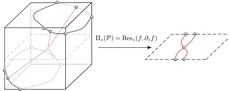
Figure 6.4: Regularity criterion for a 0-dimensional stratum.
