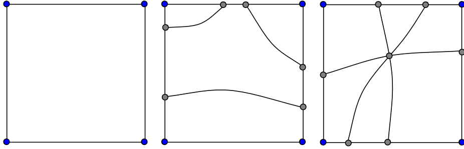
Figure 4.1: Regular cells in the plane.
