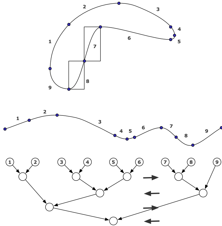
Figure 4.7: Building the region segmentation.
