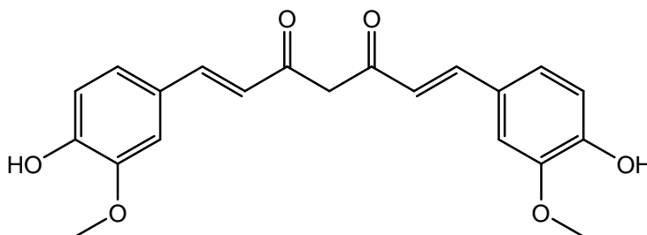
Figure 19 : Structure du Curcumin
