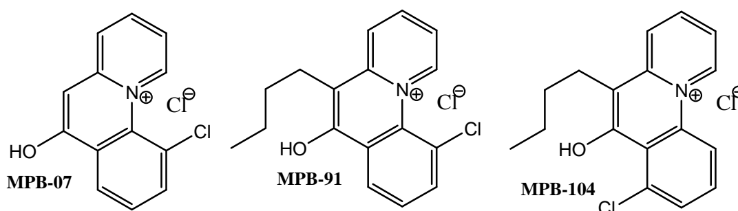
Figure 12 : Structures de trois benzo[ c ]quinoliziniums (MPB)
