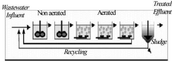
Fig. 2. Plant layout
