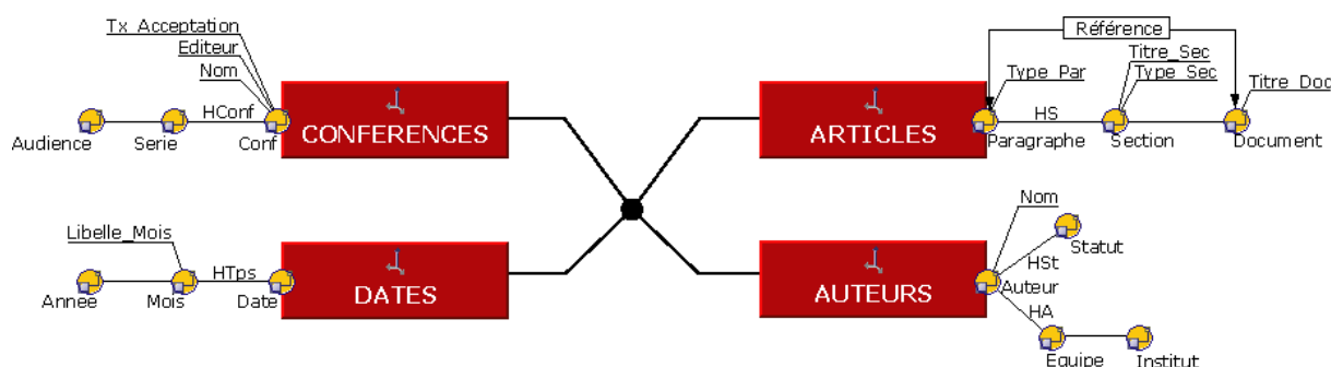
Figure 73 – Galaxie G_2 .
