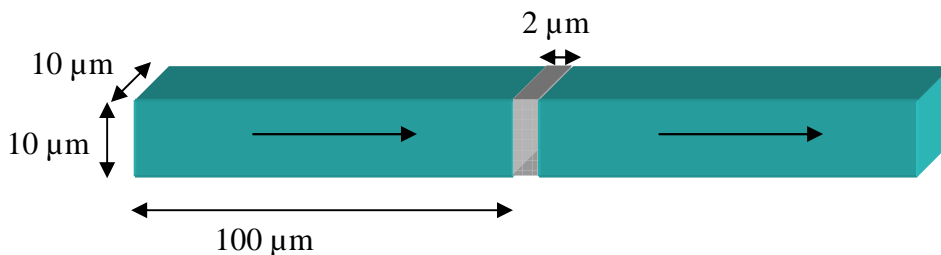
Figure 0-5 : aimants en contact (Magnets in contact)
