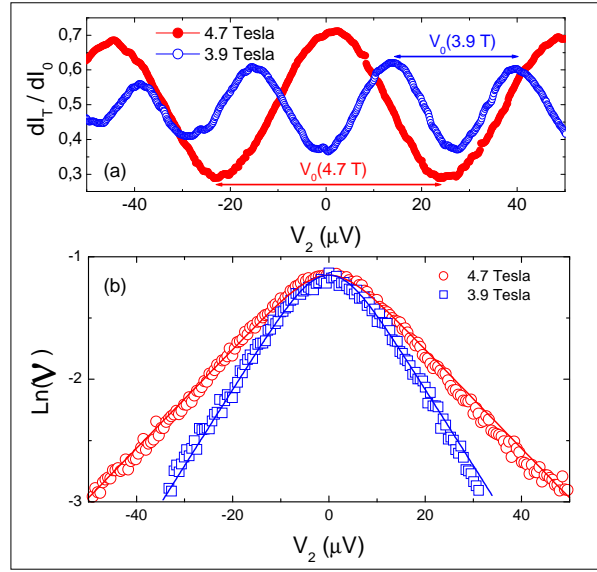
FIGURE 7.17 – (color online) a :Phase sweeping by varying V_2 with T_0 = 1 for two different magnetic fields 4.7 and 3.9 T. The periodicity V_0 depends on the magnetic field. b : Visibility decrease of the interferometer as a function of V_2 at T_0 = 1/2 for two different magnetic fields 4.7 and 3.9 T. The solid lines are fit to the data V = V_0 e^{-2\pi^2 \Delta S_{22} \Delta \nu / V_0^2} with an electronic temperature of 25mK (for a base temperature of 20mK) and T_0 = 1/2 . The high bias fit of the exponential decrease V = V_0 \exp(-T_0(1 - T_0)V_2/V_\varphi) allows us to determine V_\varphi which is found to depends on the magnetic field.
