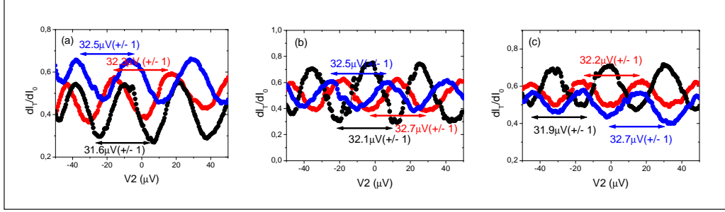
FIGURE 5.20 – Conductance oscillations versus the bias voltage V_2 applied on S_2 , for different values of V_1 and T_1 . In blue V_1 = -18 \mu\text{V} , in black V_1 = 0 \mu\text{V} and in red V_1 = 18 \mu\text{V} . (a) T_1 = 0.12 (b) T_1 = 0.6 (c) T_1 = 0.92 . In these regimes V_0 remains constant \sim 32.5 \mu\text{V} .
