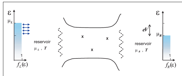
FIGURE A.3 – Schematic representation of a 2D reservoir. We note W_L ( W_R ) the left(right) reservoir width.
