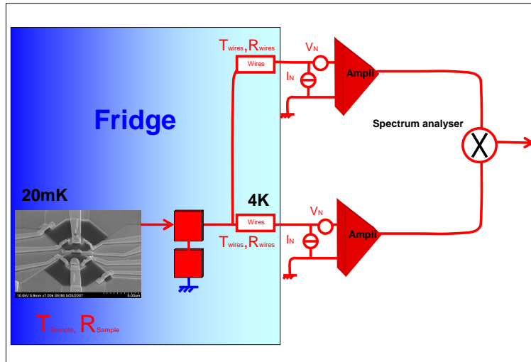
FIGURE 4.11 – Two amplification lines set up. Both amplified signals are sent on the spectrum analyzer that performs the cross correlation. Thanks to the cross correlation, the measurement is not sensitive anymore to the voltage noise of amplifiers and to the Johnson Nyquist noise of the wires.
