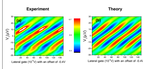
FIGURE 5.22 – Color plot of the MZI transmission versus V_1 and the voltage applied on the lateral gate. The X axis represents the lateral gate voltage, and the Y axis the bias voltage V_1 . The color plot indicates maximum and minimum of Aharonov Bohm oscillations. (a) Experimental evolution of the phase with the bias voltage V_1 when T_0 is tuned to 2. Contrary to T_0=1 when the phase is rigid, the phase now increases linearly with the bias voltage. (b) Color plot of the MZI transmission versus V_1 calculated with our formula 5.12. We notice a perfect agreement between our model and experimental data.
