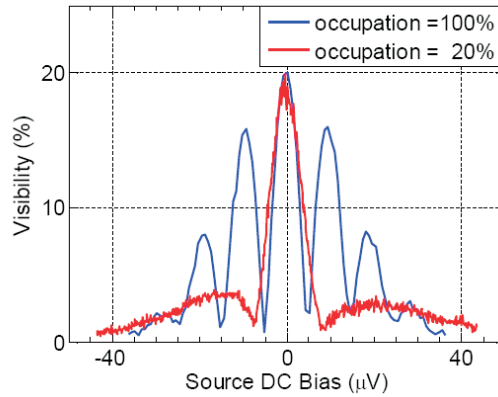
FIGURE 5.5 – The effect of beam dilution on the lobe pattern of the visibility. The dilution was performed by reflecting a part of the impinging channel with G_0 . When the occupation of the incoming edge channel was reduced to 20 %, the higher order lobes stretched and vanished while the main lobe remained almost unaffected (Neder et al. [56]).
