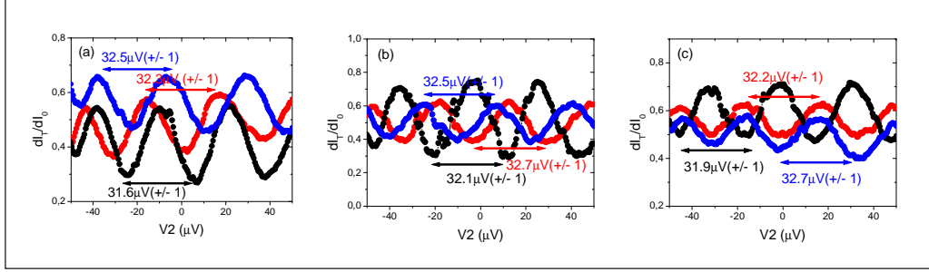
FIGURE 4.20 – Conductance oscillations versus the bias voltage V_2 applied on S_2 , for different values of V_1 and T_1 . In blue V_1 = -18 \mu V , in black V_1 = 0 \mu V and in red V_1 = 18 \mu V . (a) T_1 = 0.12 (b) T_1 = 0.6 (c) T_1 = 0.92 . In these regimes V_0 remains constant \sim 32.5 \mu V .
