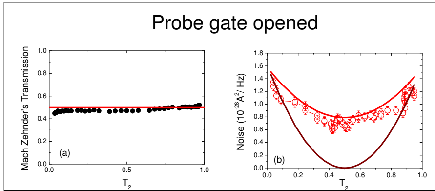
FIGURE 7.11 – (a) Mean value of the output current. Since the Mean value is equal to 0.5 when T_2=1 , transmission of the first gate T_1 \sim 0.5 . (b) Shot Noise measurement (at filling factor 2) as a function of T_{G2} when T_{G1}=1/2 and the lateral gate opened. A 58 \mu V DC voltage is applied for the shot noise measurement. The excess noise measured at 58 \mu V is shown in red circles. In red solid line, inelastic relaxation approach considering that there is no inelastic relaxation in the upper path. The dark red solid line corresponds to complete inelastic relaxation occurring in both path.
