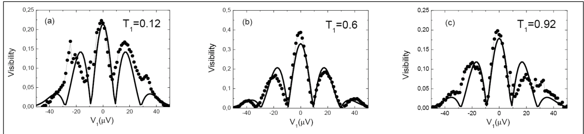
FIGURE 5.31 – Visibility as a function of the bias V_{ds} for different transmissions of the first beam splitter. In solid lines, fits using formula 5.7 (a) T_1 is set to 0.12.(b) T_1 is set to 0.6.(c) T_1 is set to 0.92. The lobe width does not depend on the transmission of the first beam splitter.
