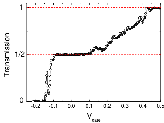
FIGURE 4.7 – Transmission behavior of a quantum point contact with the gate voltage at filling factor \nu=2 . For a gate voltage of +0.5V (when the sample is cooled down, gates are biased with +0.5V ) both edge states are transmitted, the transmission is equal to 1. When the gate voltage is null, the transmission is equal to 1/2 , only the outer edge state is transmitted, the inner one being totally reflected. Since, we will reveal Aharonov Bohm oscillations on the outer edge state, with a transmission equal to T_{out}=1/2 , gate voltages usually applied in our experiments are \sim -0.15V .
