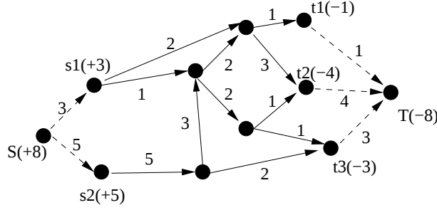
Figure 2.6: Flow between several sources and several sinks
