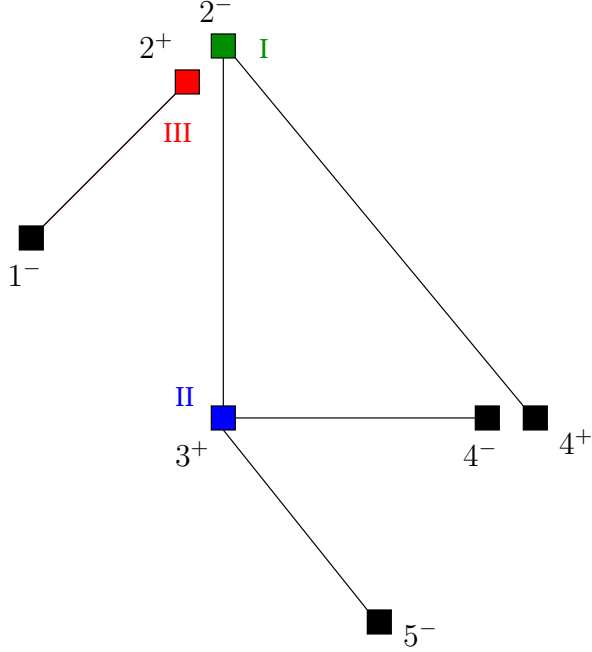
Figure 3.4: Associated bipartite graph
