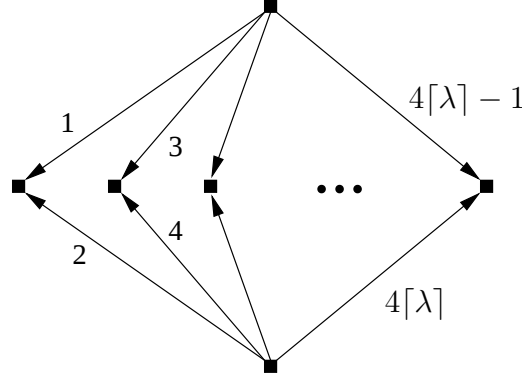
Figure 3.5: Instance for which the algorithm is far from optimality
