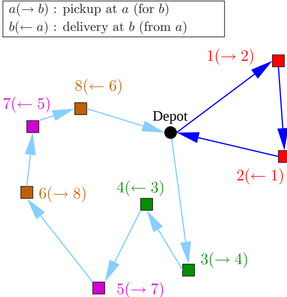
Figure 2.1: Example a of PDP solution
