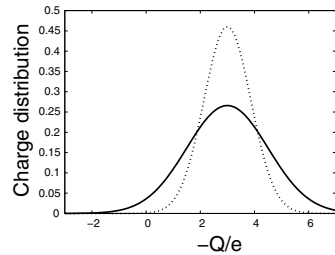
FIG. 9. Charge distribution with and without image force correction. The dotted line represents the distribution with \Delta Q = 0.5\sqrt{Q} . The solid line represents the distribution with \Delta Q = 0.87\sqrt{Q} [37].
