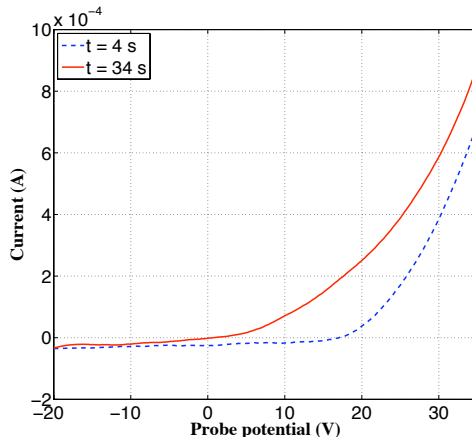
Figure 4.13: I-V Langmuir probe characteristics at different instants of the discharge life ( P = 1.75 \text{ Torr} and V_{pp} = 280 \text{ V} ). The curves have been smoothed.
