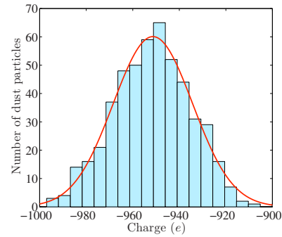
FIG. 3. (Color online) Dust charge distribution for 190 nm radius dust particles with n_{i0} = 5 \times 10^9 \text{ cm}^{-3} and n_d = 5 \times 10^4 \text{ cm}^{-3} .
