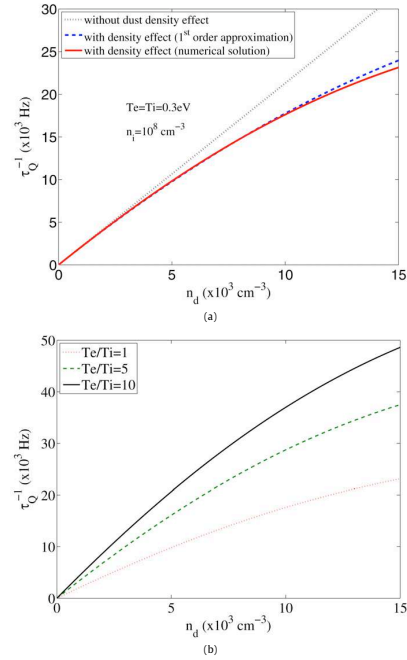
Fig. 1. (Color online.) Particle absorption frequency as a function of the dust density. (a) With or without taking into account the dust density effect. (b) Numerical solution for different T_e/T_i .
