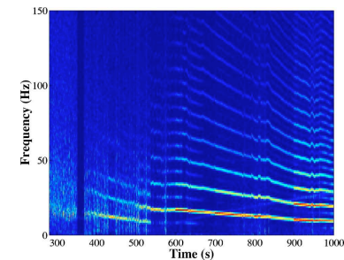
FIG. 13. (Color online) Spectrogram of a particular case of the second chaotic regime corresponding to void rotation in a horizontal plane.
