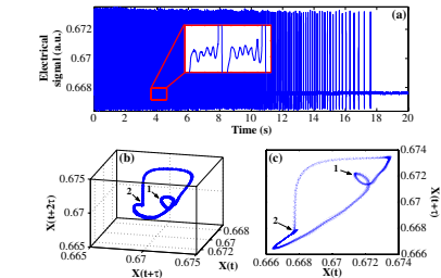
FIG. 2 (color online). (a) Evolution of the electrical signal during the instability ending phase. The insert is a zoom of a transition between 1^4 and 1^5 states. Corresponding phase space is represented in (b) 3D and (c) 2D. Arrows labeled 1 and 2 show, respectively, the loop due to the additional peak observed on the right-hand side of spikes [see Fig. 1(a)] and the region containing the loops corresponding to failed peaks.
