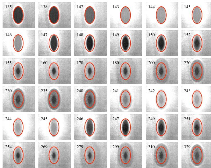
Figure 5.13: Simultaneous record of the plasma glow and the dust cloud in the void region during the setting up of the heartbeat instability. From image 135: stable open void (delineated by a red ellipse) followed by a first contraction. A new contraction starts at image 241 before the original conditions have been restored
