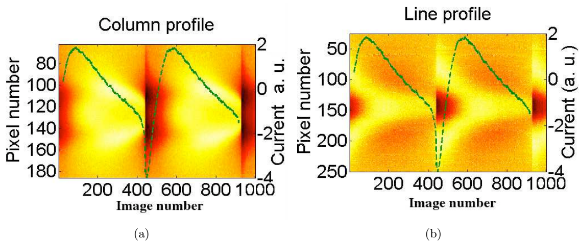
Figure 5.24: Evolution of glow luminosity extracted from the video images presented in Fig.5.23 (in false colour from dark red to bright yellow). (a) Evolution of the central column luminosity. (b) Evolution of the central line luminosity (frame rate: 1789 fps). In both cases, the time average value of each pixels has been subtracted in order to enhance luminosity variations. The dashed green line superimposed on each picture represents the discharge current (AC component) during the delivery instability.
