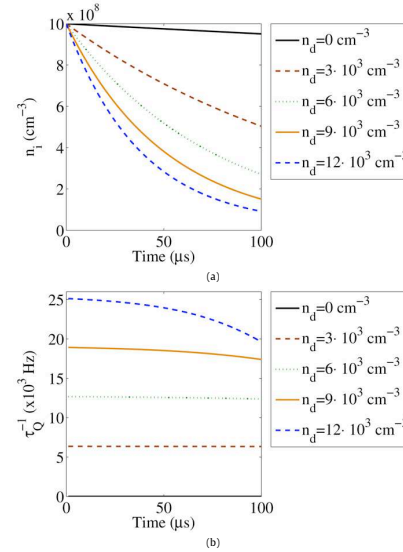
Fig. 3. (Color online.) Top: evolution of ion density n_i during the first microseconds of a plasma afterglow for different dust density. Bottom: evolution of the dust particle absorption frequency \tau_Q^{-1} during the first microseconds of a plasma afterglow for different dust density. The plasma diffusion frequency is \tau_D^{-1} = 500 Hz and T_e = T_i = 0.3 eV.
