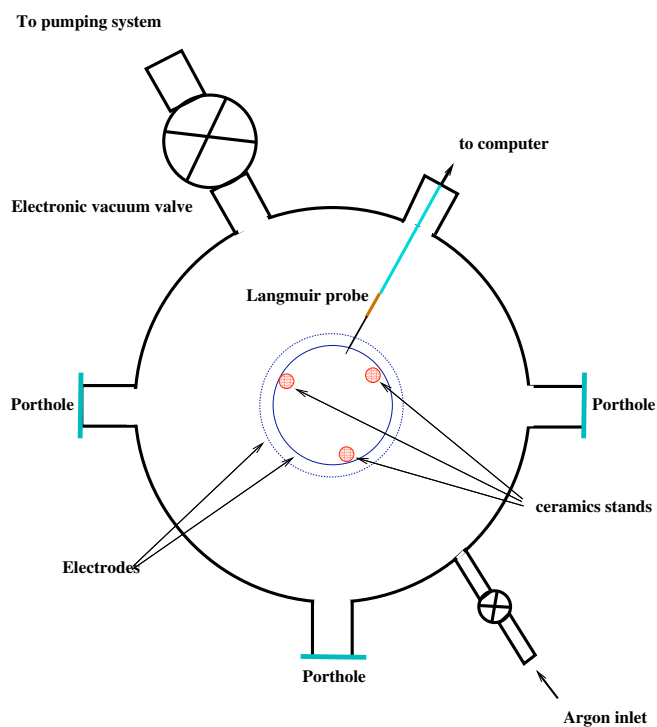
Figure 3.11: Langmuir probe measurement schematic
