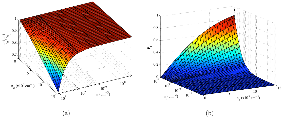
Figure 6.4: (a) Ratio of the dust particle absorption frequency taking into effect dust density effect \tau_A^{-1} relative to the dust particle absorption frequency not taking into effect dust density effect \tau_{A_0}^{-1} for different values of dust and plasma densities. (b) Havnes parameter P_H for different values of dust and plasma densities.
