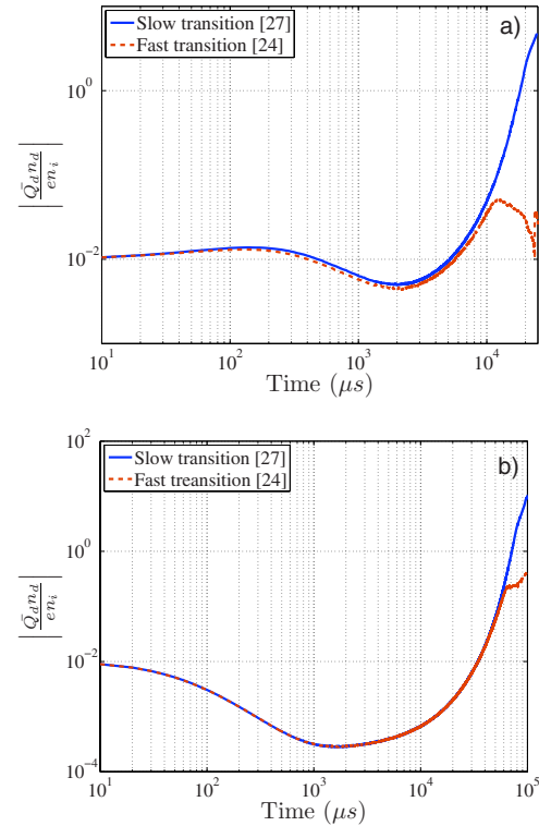
FIG. 8. (Color online) Evolution of |\bar{Q}_d n_d / en_i| . (a) P=0.4 mbar. (b) P=1.2 mbar.
