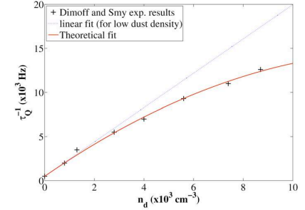
Fig. 4. (Color online.) Fit of experimental results of Ref. [14] using the first order approximation (Eq. (14)).
