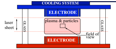
FIG. 1. (Color online) Schematic of the experimental apparatus.
