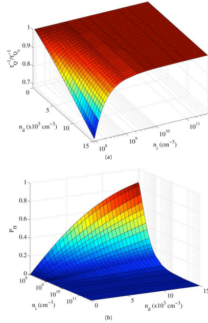
Fig. 2. (Color online.) (a) Ratio of the dust particle absorption frequency taking into account dust density effect \tau_Q^{-1} over the dust particle absorption frequency not taking into account dust density effect \tau_{Q_0}^{-1} for different dust density and plasma density. (b) Havnes parameter P_H for different dust density and plasma density.
