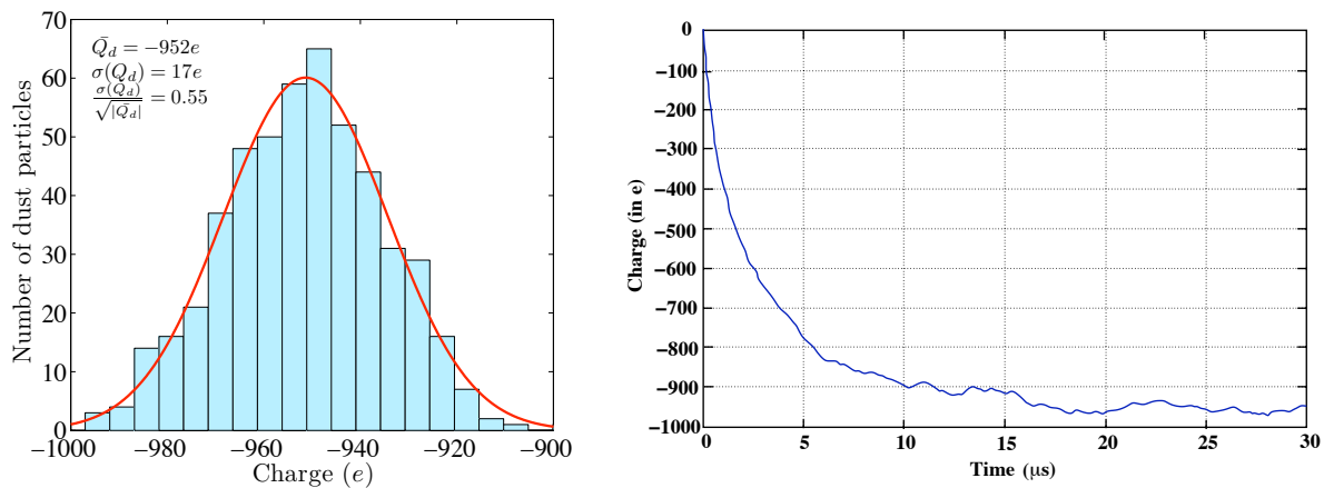
Figure 2.2: Calculation of dust particle charges using a Fokker-Planck algorithm [93] for 190 nm radius particles in a plasma with T_e = 3 eV, T_i = 0.03 eV and n = n_e = n_i = 5 \cdot 10^9 cm ^{-3} . Left: Dust particle charge distribution for 500 iterations. Right: Dust particle charge evolution when immersed in the plasma
