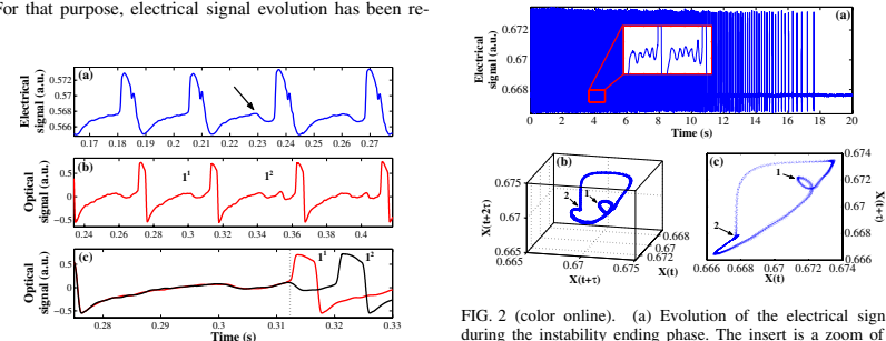
FIG. 1 (color online). (a) Electrical signal with a transition between 1^0 and 1^1 states (arrow: failed peak). (b) Optical signal with a transition between 1^1 and 1^2 states. (c) Superimposition of the two consecutive states shown in (b).
