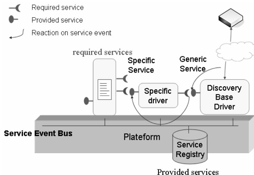
Figure 49 Chaine de pilotes : "Discovery Base Driver" et "Specific Driver"
