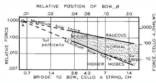
Figure 3.5: Schelleng diagram, from [71]. The figure shows the maximum and the minimum bow force limits for Helmholtz motion vs. bow-bridge distance, at a given bow velocity. Usual descriptions of the tone color are indicated in different regions.
