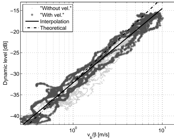
Figure 6.10: Representation of the variations of the sound level versus v_b/\beta during the crescendo - diminuendo for the two experiments (“with velocity”, stars, and “without velocity”, dots). A good fit is obtained with L \propto 7.7 \log(v_b/\beta) (black line). The theoretical variation L \propto 8.7 \log(v_b/\beta) is shown in dashed line.
