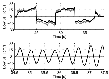
FIG. 11. Computed bow velocity signals obtained by piece-wise integration of bow acceleration between bow changes for sequences of whole notes (top) and semi-quavers (bottom). The gray curves show bow velocity obtained by motion capture.
