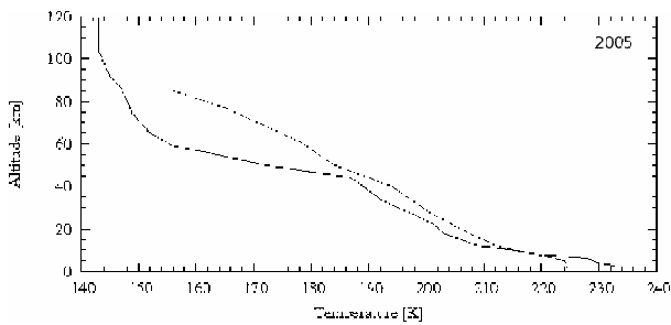
Fig. 12. Atmospheric temperature profile in 2005 derived from the observations (solid lines) and from Clancy et al. (2006) (dashed lines).
