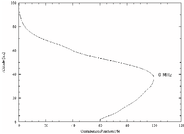
Fig. 4. Contribution function for the central frequency of the ^{13}\text{CO}(2-1) line in 2001.
