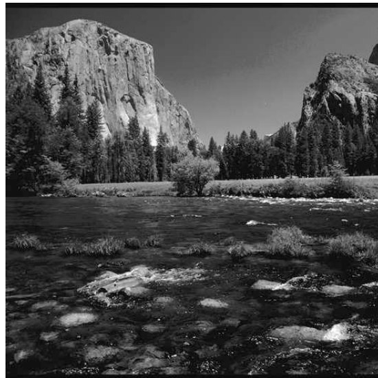
FIGURE C.15 – yosemite
