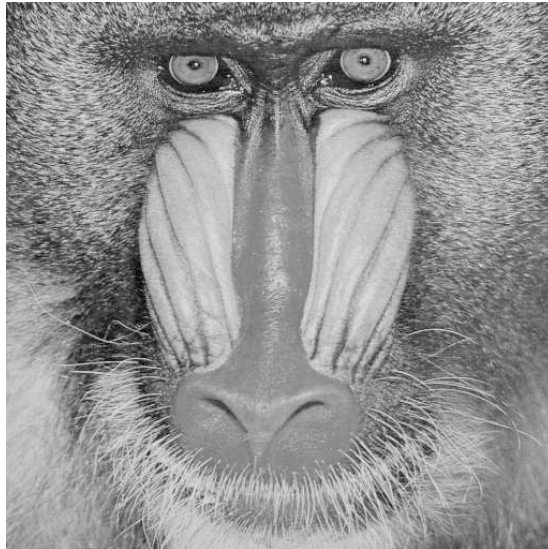
FIGURE C.1 – baboon
