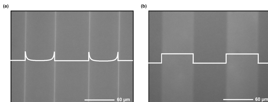
Figure 3.12: Optical micrographs (parts (a) and (b) ) of stamps placed against glass slides, obtained by imaging through the stamps. The lines schematically illustrate the shape of the relief (500 nm height) on the stamp after contact. Part (a) indicates complete sagging of the recessed regions of a conventional single component poly(dimethylsiloxane) (PDMS) stamp. Part (b) shows a similar image of a composite stamp that uses the same PDMS chemistry, but in a thin film ( \sim 25 \mu\text{m} ) geometry supported by a thin ( 25 \mu\text{m} ) polyimide sheet. This stamp shows no evidence of sagging.
