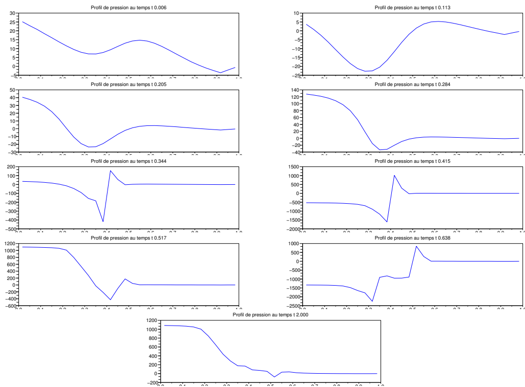
Figure 5.22: Pressure for different times
