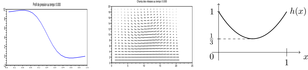
Figure 5.7: Pressure, velocity field and form of the domain for a medium ratio \frac{h_M}{h_m}
