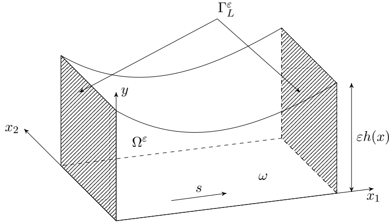
Figure 2.1: Domain \hat{\Omega}_\varepsilon
