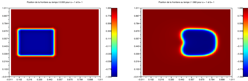
Figure 5.15: Repartition of the fluids for a = 1, b = 1
