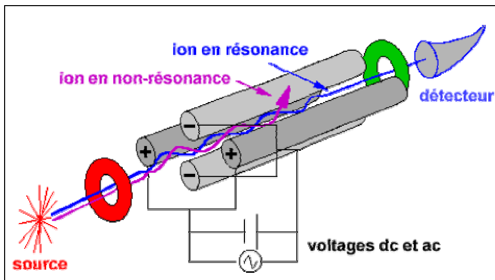
Figure I.17 : Quadripôle
