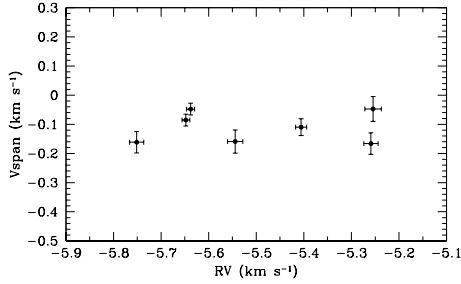
Figure 4. Analysis of line-bisectors in WASP-3 shows the bisector velocity ( v_{span} ) does not correlate with stellar radial-velocity. This demonstrates that the cross-correlation function remains symmetric, and that the radial-velocity variations are not likely to be caused by line-of-site binarity or stellar activity.
