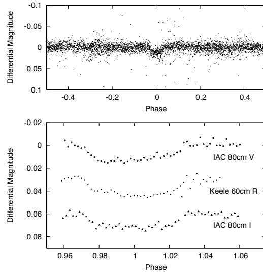
Figure 1. Light Curves for 1SWASP J183431.62+353941.4 (WASP-3) obtained with SuperWASP-N (top panel), the IAC 80-cm telescope (V and I) and the Keele 60-cm telescope (R) as marked. All the data (apart from that from SuperWASP-N) was averaged in 300 second bins. The data was phased using the ephemeris derived in Section 3.2.1, T_0 = 2454143.8504 and P = 1.846834 days.
