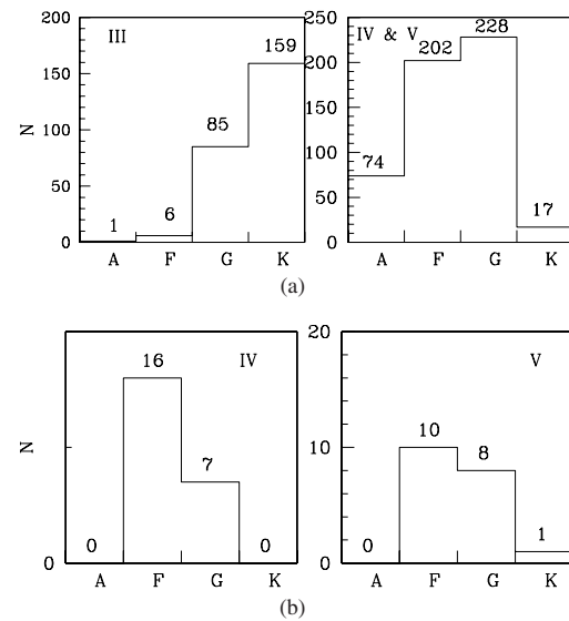
Fig. 2. Distribution of the sample of observed stars with the GIRAFFE (a) and the UVES/FLAMES ; (b) spectrograph over the spectral type for dwarfs and giants. The sample is completed by a O-type dwarf star and a M-type giant star.
