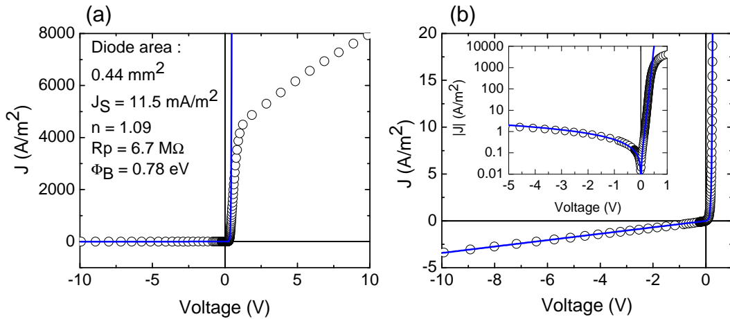
Figure 4.14: 4-point probe I-V measurements of a Au/Si (n-type) Schottky diode. The thermionic emission model was used to fit the data. Plot (b) is a zoom of plot (a), while the log scale inset demonstrates the agreement between experiment and fitting.
