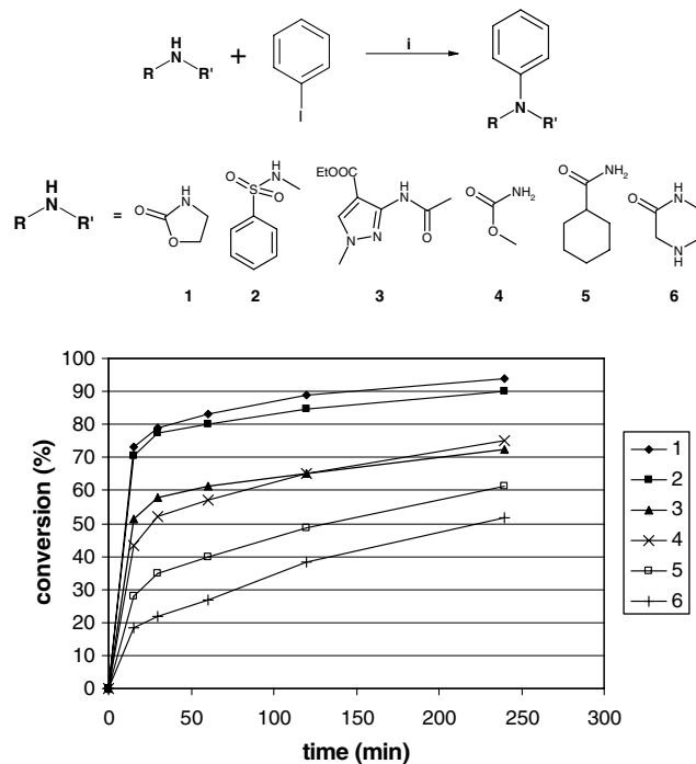
Figure 1. Iodobenzene conversion by nucleophiles 1 to 6 . Reagents and conditions: (i) 1 equiv of nucleophile, 1 equiv of iodobenzene, 0.1 equiv of CuI, 2 equiv of K 3 PO 4 , 0.2 equiv of N,N' -dimethyl-cyclohexane-1,2-diamine, 0.5 equiv of 1,2,4,5-tetramethylbenzene (durene), dioxane (0.5 M), 110 °C. Sampling performed under an argon overpressure. Ratio determined by UV detection at 215 nm.
