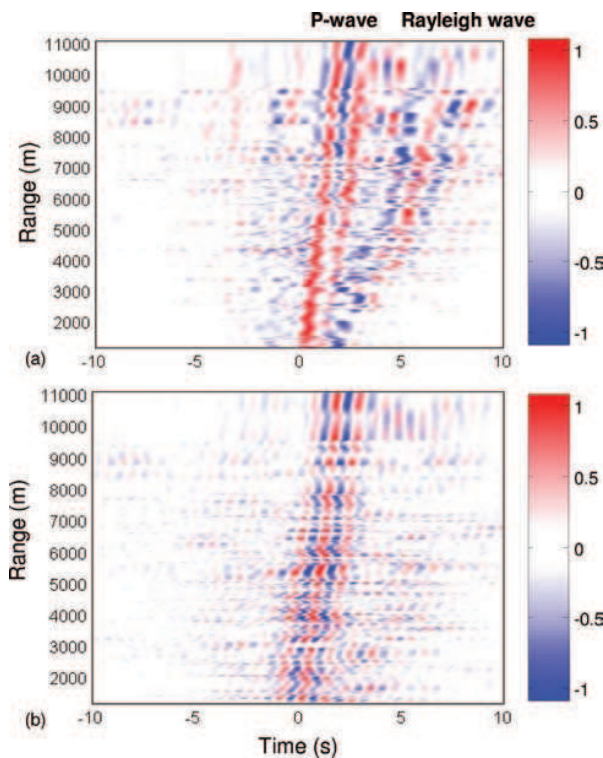
Figure 8 Range-time representation of the Z-Z component of the noise correlation tensor averaged over one month in two frequency bands (a) [0.1–1.3 Hz], and (b) [0.6–1.3 Hz]. Each plot has been normalized by its own maximum.
