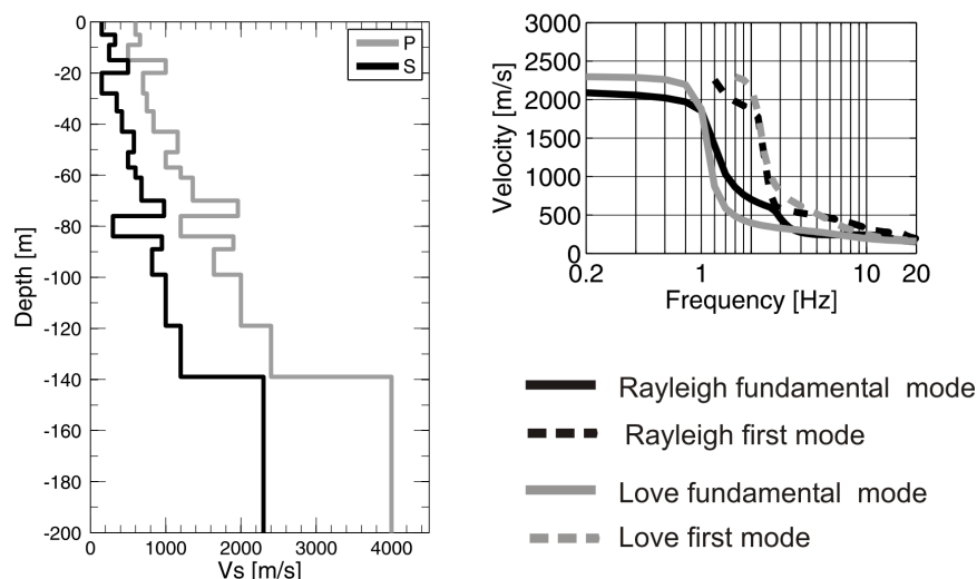
Figure 3.1: (Left-hand panel) P- and S-wave velocity profiles (grey and black curves, respectively); (right-hand panel) corresponding Rayleigh and Love waves dispersion curves for the fundamental and first higher modes.
