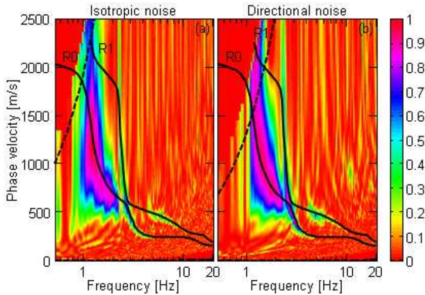
Figure 3.7: Frequency-velocity diagrams for NCSS applied to the Z - Z component of the correlation tensor in the case of isotropic (a) and directional (b) noise. The two first theoretical Rayleigh modes (R0 and R1 modes) are indicated by full lines. Limits of array response given the following wavelength limits [ \lambda_{min} = 2d_{min} , \lambda_{max} = 3d_{max} ] are indicated by dashed lines (low velocity limits corresponding to \lambda_{min} is very close to the frequency axis).
