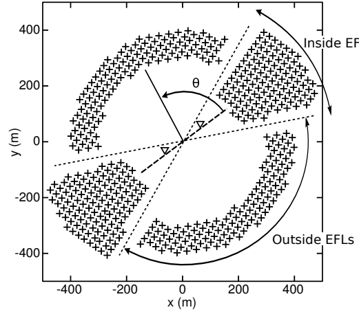
Figure 2.2: The two geometries we considered, based on \theta . The first is |\theta| < 20^\circ and 180 - |\theta| < 20^\circ , for which sources are inside the EFLs of the receiver pair. the second is 150^\circ > |\theta| > 30^\circ , for which sources are outside the endfire lobes. In both cases, radii R1 and R2 are changed to 200–515 m and 300–400 m, respectively, to include the same number of sources as in Figure 2.1a.
