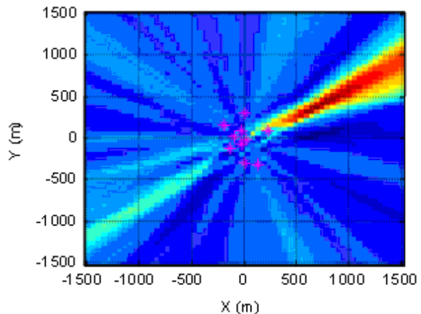
Figure 3.8: Matched field processing indicates impinging sources (red-colour region) propagating with a backazimuth of N61^\circ . (Y positive direction indicates North and X positive direction indicates East). Purple stars indicate station locations.
