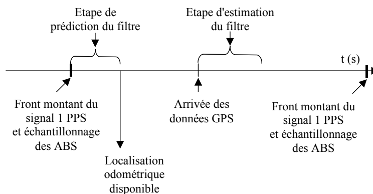
Figure 4.33. Chronogramme.
