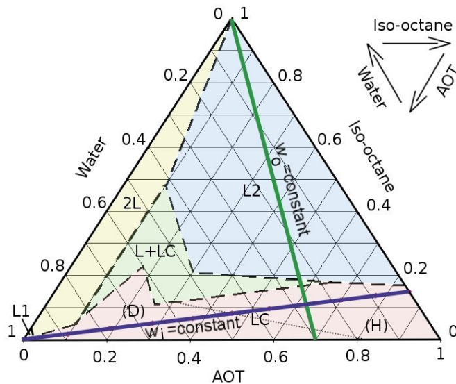
Figure 1.7: Simplified phase diagram of the AOT / Iso-octane / water ternary mixtures at 25C [10].
