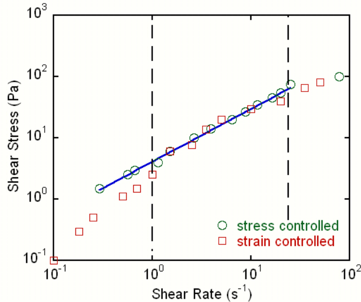
Figure 5.7: Apparent steady stress as a function of the shear rate from strain-controlled and stress-controlled rheometry. Plain line is the power law to which the measured data fit for intermediate shear rates and stresses:
