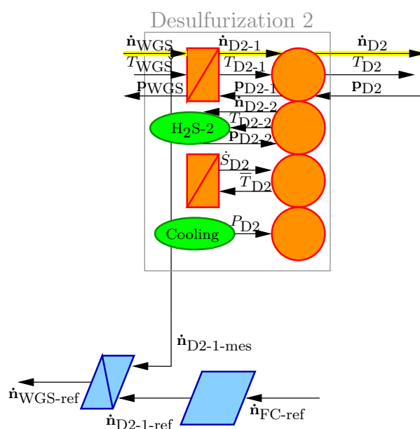
Figure 5.11: EMR and control structure of Desulfurization 2
