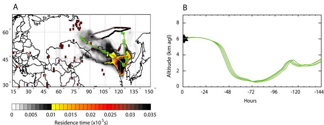
Figure 6.9. Footprint of the high CO concentrations ( \text{CO} > 220 \text{ppb} ) computed using the FLEXPART model. FLEXPART releases a large number of particles at the receptor (instrument) location and computes time-reversed transport. ECMWF reanalysis wind field is used. The footprint, or potential emission sensitivity (PES) is defined as the geographic distribution of the cumulative counts of the particles residence time. The colour scale represent the footprint in the lowest 1500 m, and therefore the sensitivity to emissions occurring in these areas. The green curves represent 3 typical high CO back-trajectories computed using the HYSPLIT model. In the right panel, the variation of altitude with time is plotted for these 3 back-trajectories.
