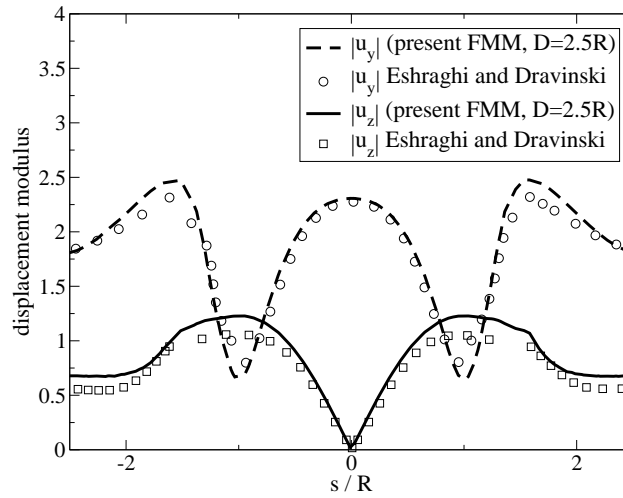
Figure 2.27: Diffraction of an incident ( \theta = 0^\circ ) plane SV-wave by a semi-spherical canyon: Comparison of horizontal and vertical computed displacements for D = 2.5a , against normalized arc-length coordinate s/a along ABC (normalized frequency k_{SA}/\pi = 0.75 ) with results of Eshraghi and Dravinski [73].
