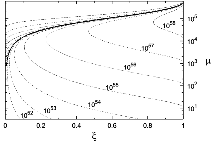
Fig. 16. Selected lines corresponding to fixed values of the E_{\text{dya}} are given as a function of the two parameters \mu , \xi , only the solutions below the continuous heavy line are physically relevant. The configurations above the continuous heavy lines correspond to unphysical solutions with r_{\text{ds}} < r_+ .
