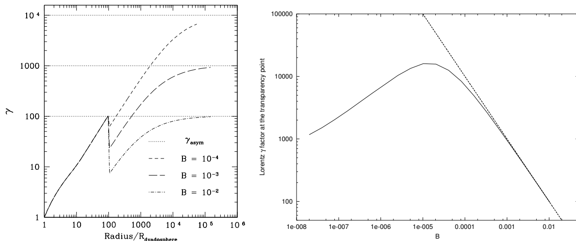
Figure 3.7: Left) The \gamma factors are given as functions of the radius in units of the dyadosphere radius for selected values of B for the typical case E_{\text{dya}} = 3.1 \times 10^{54} erg. The asymptotic values \gamma_{\text{asym}} = E_{\text{dya}}/(M_B c^2) = 10^4, 10^3, 10^2 are also plotted. The collision of the PEMB pulse with the baryonic remnant occurs at r/r_{\text{ds}} = 100 where the jump occurs. Right) The \gamma factor (the solid line) at the transparency point is plotted as a function of the B parameter. The asymptotic value (the dashed line) E_{\text{dya}}/(M_B c^2) is also plotted.
