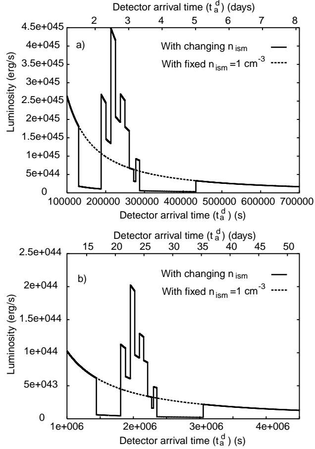
Fig. 5. – a) Same as fig. 3b with the ISM cloud located at a distance of 3.17 \times 10^{17} cm from the EMBH, the time scale of the burst now extends to \sim 1.58 \times 10^5 s. b) Same as a) with the ISM cloud at a distance of 4.71 \times 10^{17} cm from the EMBH, the time scale of the burst now extends to \sim 1.79 \times 10^6 s.
