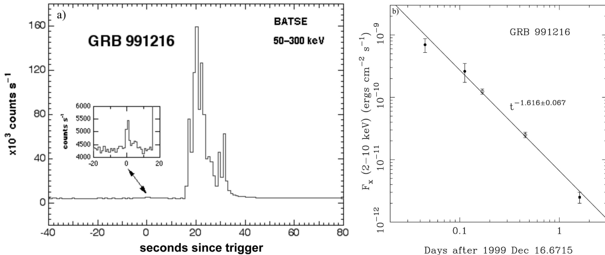
Figure 4.3: a) The data on the GRB 991216 obtained by BATSE (reproduced from BATSE 1999) and b) the corresponding data for the afterglow from both RXTE and Chandra (the last point after 10^5 s) are given as a function of the detector arrival time (reproduced from [58]).
