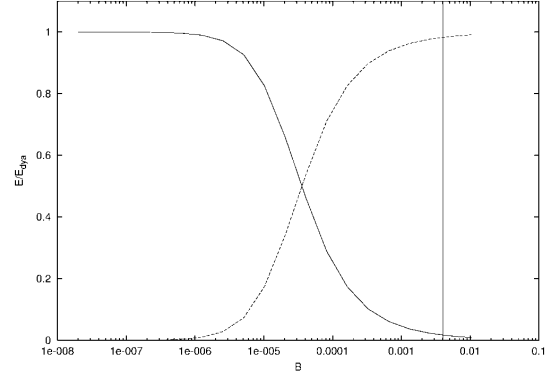
FIG. 4.—Relative intensities of the afterglow ( dashed line ) and the P-GRB ( solid line ), as predicted by the EMBH model corresponding to the values of the parameters determined in Fig. 3, as a function of B . Details are given in (Bianco et al. 2001a). The vertical line corresponds to the value B = 4 \times 10^{-3} .
