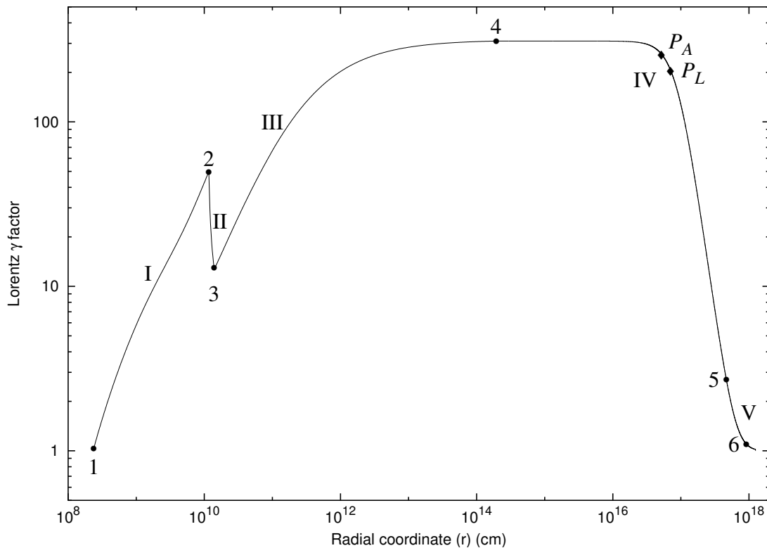
Figure 4.2: The theoretically computed \gamma factor for the parameter values E_{dya} = 4.83 \times 10^{53} erg, B = 3 \times 10^{-3} is given as a function of the radial coordinate in the laboratory frame. The corresponding values in the comoving time, laboratory time and arrival time are given in Tab .1 in [109]. The different eras indicated by roman numerals are illustrated in the text (see sects. 3.3,3.4,3.5,4.2,4.4), while the points 1,2,3,4,5 mark the beginning and end of each of these eras. The points P_L and P_A mark the maximum of the afterglow flux, respectively in laboratory time and in arrival time (see [104] and sects. 4.5,4.6). The point 6 is the beginning of Phase D in Era V (see sects. 4.4,4.3). At point 4 the transparency condition is reached and the P-GRB is emitted. This diagram shows the inadequacy of considering the simple power-law behaviour \gamma \propto r^{-3} for the relation between the radius of the source and its Lorentz \gamma factor as assumed in the large majority of current papers on GRBs (see e.g. [124, 145, 125, 127, 85, 89] and references therein). Actually, such a power-law behaviour with the predicted index can never be realized (see sect. 4.11).
