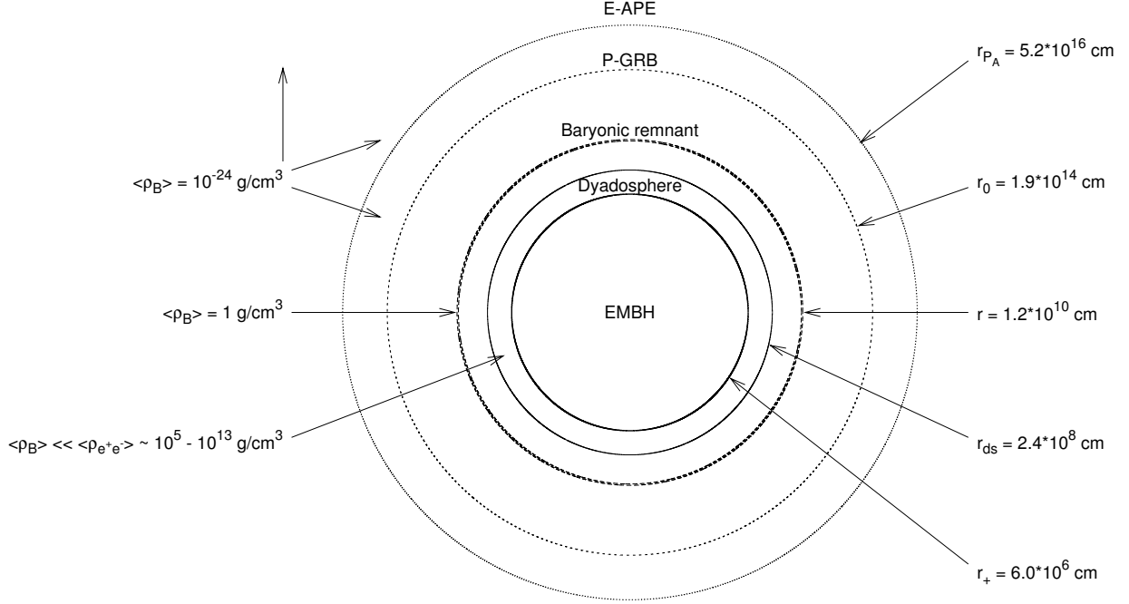
Figure 3.1: Selected events in the EMBH model are represented. For each one the values of the energy density of the medium and the distances from the EMBH in the laboratory frame are given for the prototype GRB 991216; logarithmic scale is used.
