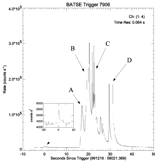
FIG. 4.—BATSE data on the E-APE of GRB 991216 (source: BATSE GRB light curves; see http://gammaray.mscf.nasa.gov/batse/grb/lightcurve ) together with an enlargement of the P-GRB data (source: BATSE rapid burst response; see http://gammaray.mscf.nasa.gov/~kippen/batserbr ). For convenience, each E-APE peak has been labeled by a different uppercase Latin letter.
