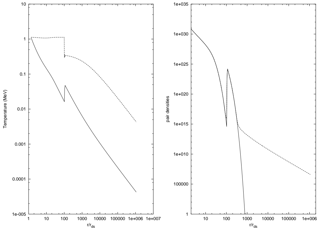
Figure 24: Left) The temperature of the plasma in the comoving frame T' (MeV) (the solid line) and in the laboratory frame \gamma T' (the dashed line) are plotted as functions of the radius in the unit of the dyadosphere radius r_{ds} . Right) The number densities n_{e^+e^-}(T) (the solid line) computed by the Fermi integral and n_{e^+e^-} (the dashed line) computed by the rate equation (see section IV) are plotted as functions of the radius. T' \ll m_e c^2 , two curves strongly divergent due to e^+e^- -pairs frozen out of the thermal equilibrium. The peak at r \simeq 100r_{ds} is due to the internal energy developed in the collision.
