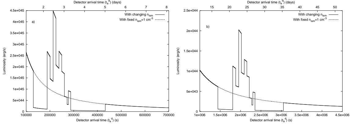
Figure 38: a) Same as Fig. 36b with the ISM cloud located at a distance of 3.17 \times 10^{17} cm from the EMBH, the time scale of the burst now extends to \sim 1.58 \times 10^5 s . b) Same as a) with the ISM cloud at a distance of 4.71 \times 10^{17} cm from the EMBH, the time scale of the burst now extends to \sim 1.79 \times 10^6 s .
