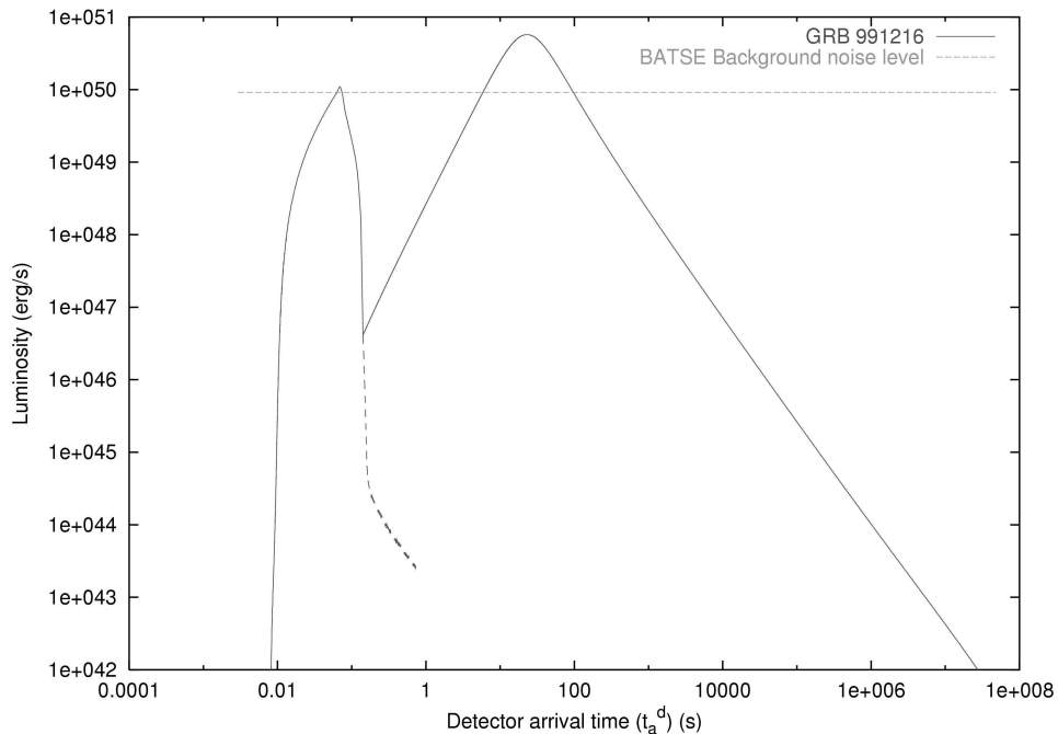
Fig. 14. A qualitative diagram showing the full picture of the model, with both P-GRB and E-APE.
