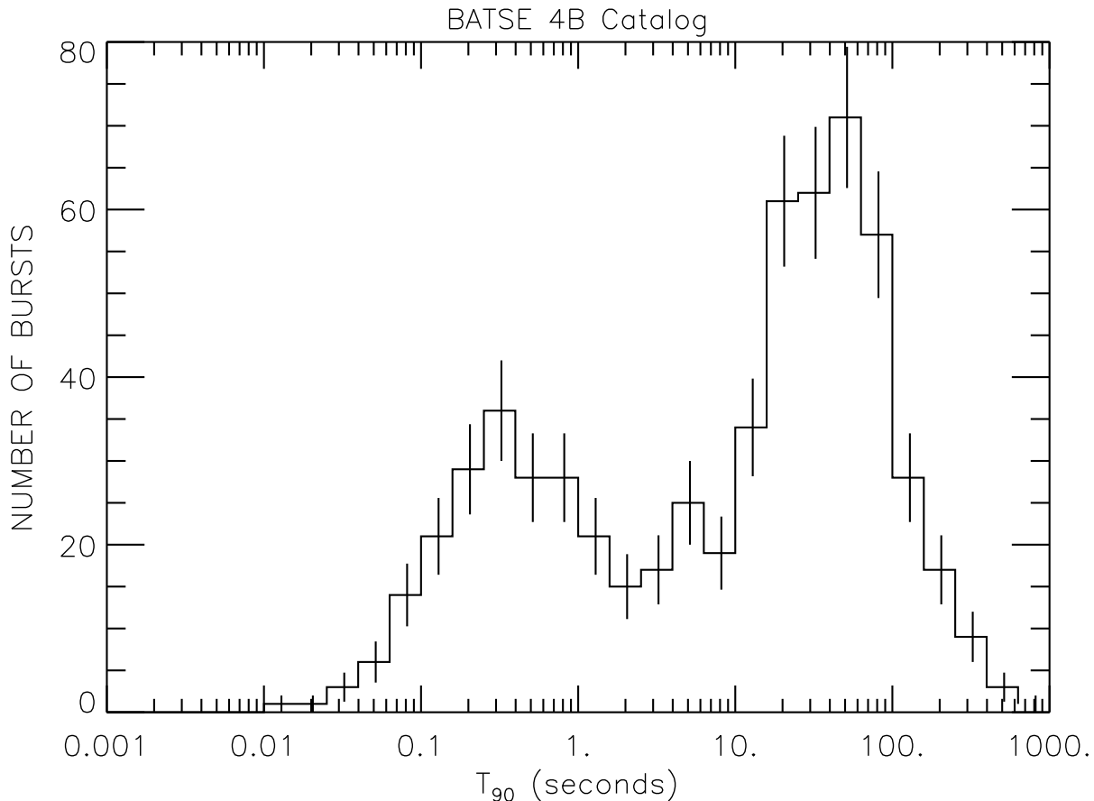
Figure 2.2: Histogram of GRB time duration from BATSE 4B catalog [6]. The duration is computed by the T_{90} ( T_{50} ) criterion, according to which the duration of an event is assumed to be the time interval during which is collected from 5% (25%) to 95% (75%) of the total energy emitted. A time interval is chosen because, due to background noise, it is never possible to determine the instant of beginning (0%) and of the end (100%) of the signal. From this histogram emerges that GRBs divide in two classes: “short GRBs” and “long GRBs”.
