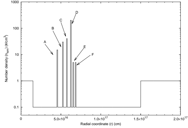
Figure 43: The density profile (“mask”) of an ISM cloud used to reproduce the GRB 991216 temporal structure. As before, the radial coordinate is measured from the black hole. In this cloud we have six “spikes” with overdensity separated by low density regions. Each spike has the same spatial extension of 10^{15} cm. The cloud average density is \langle n_{ism} \rangle = 1 particle/cm 3 .
