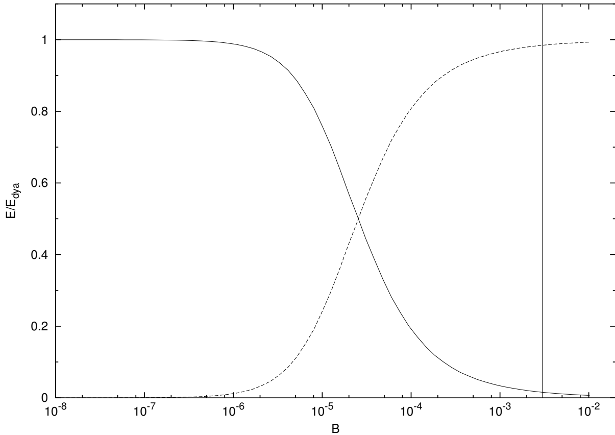
Figure 4.7: Prediction in the EMBH model of the relative energies, in units of E_{dya} = 4.83 \times 10^{53} erg, of P-GRB (solid line) and of afterglow (dashed line), computed as kinetic energy of baryons at transparency point. The vertical line corresponds to the value B = 3 \times 10^{-3} of best fit of GRB 991216.
