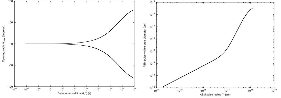
Figure 40: Left) Not all values of \vartheta are allowed. Only photons emitted at an angle such that \cos\vartheta \geq (v/c) can be viewed by the observer. Thus the maximum allowed \vartheta value \vartheta_{max} corresponds to \cos\vartheta_{max} = (v/c) . In this figure we represent \vartheta_{max} (i.e. the angular amplitude of the visible area of the ABM pulse) in degrees as a function of the arrival time at the detector for the photons emitted along the line of sight (see text). In the earliest GRB phases v \sim c and so \vartheta_{max} \sim 0 . On the contrary, in the latest phases of the afterglow the ABM pulse velocity decreases and \vartheta_{max} tends to the maximum possible value, i.e. 90^\circ . Right) The diameter of the visible area is represented as a function of the ABM pulse radius. In the earliest expansion phases ( \gamma \sim 310 ) \vartheta_{max} is very small (see left pane and Fig. 41), so the visible area is just a small fraction of the total ABM pulse surface. On the other hand, in the final expansion phases \vartheta_{max} \rightarrow 90^\circ and almost all the ABM pulse surface becomes visible.
