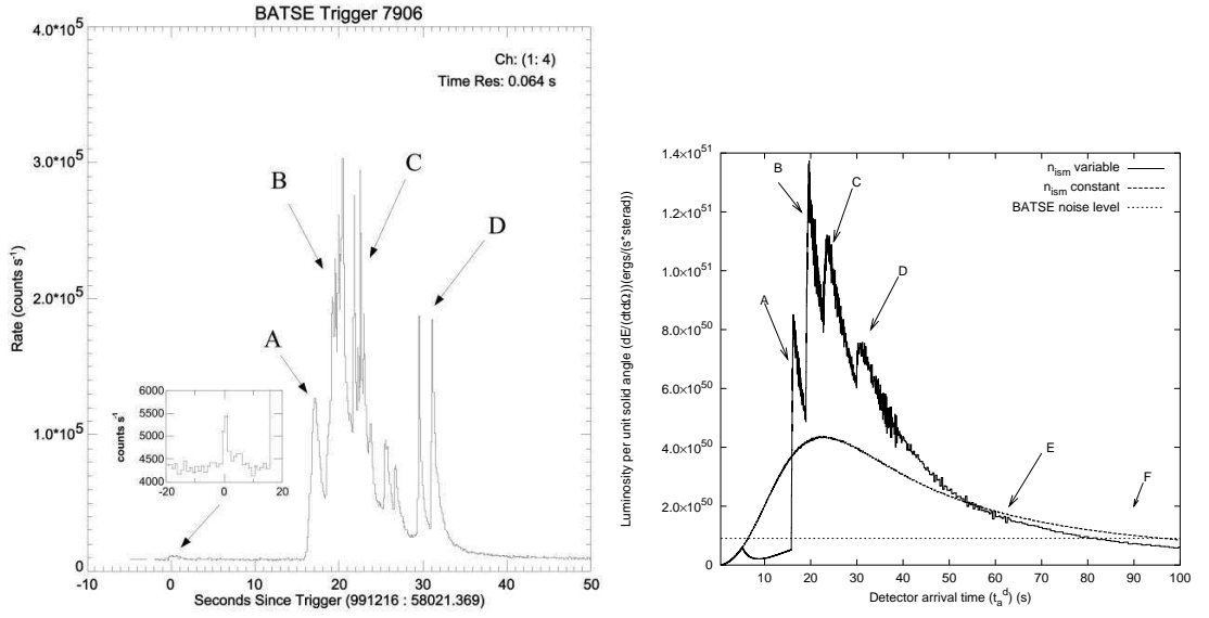
Figure 44: Left ) The BATSE data on the E-APE of GRB 991216 (source: BATSE GRB light curves [5]) together with an enlargement of the P-GRB data (source: BATSE Rapid Burst Response [6]). For convenience each E-APE peak has been labeled by a different uppercase Latin letter. Right ) The source luminosity connected to the mask in Fig. 43 is given as a function of the detector arrival time (solid “spiky” line) with the corresponding curve for the case of constant n_{ism} = 1 particle/cm 3 (dashed smooth line) and the BATSE noise level (dotted horizontal line). The “noise” observed in the theoretical curves is due to the discretization process adopted, described in Ruffini et al. [153], for the description of the angular spreading of the scattered radiation. For each fixed value of the laboratory time we have summed 500 different contributions from different angles. The integration of the equation of motion of this system is performed in 22,314,500 contributions to be considered. An increase in the number of steps and in the precision of the numerical computation would lead to a smoother curve.
