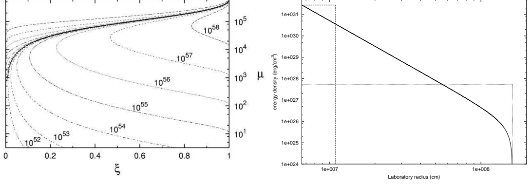
Figure 17: Left ) Selected lines corresponding to fixed values of the E_{dya} are given as a function of the two parameters \mu \xi , only the solutions below the continuous heavy line are physically relevant. The configurations above the continuous heavy lines correspond to unphysical solutions with r_{ds} < r_+ . Right ) Two different approximations for the energy density profile inside the dyadosphere. The first one (dashed line) fixes the energy density equal to its peak value, and computes an “effective” dyadosphere radius accordingly. The second one (dotted line) fixes the dyadosphere radius to its correct value, and assumes an uniform energy density over the dyadosphere volume. The total energy in the dyadosphere is of course the same in both cases. The solid curve represents the real energy density profile.
