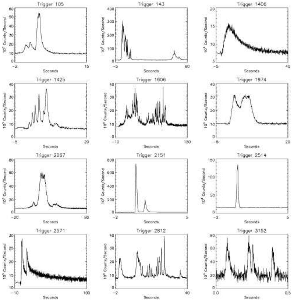
Figure 2.3: Variability of temporal profile of a single event with time scale down to ms and difference of temporal profile between different events is shown, making evident the difficulty of building a single model reproducing all observational features. Usually “long” events present a more complicated temporal structure than “short” ones.
