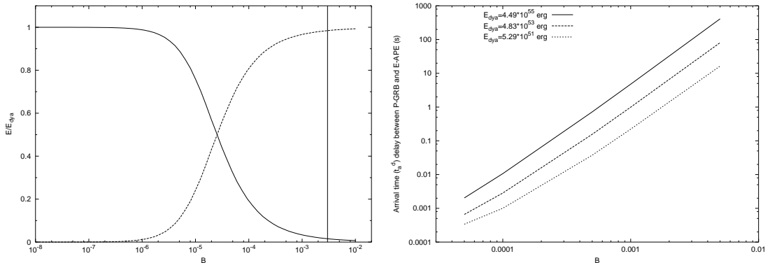
Figure 11: Left ) Relative intensities of the E-APE (dashed line) and the P-GRB (solid line), as predicted by the EMBH theory corresponding to the values of the parameters determined in Fig. 10, as a function of B . Details are given in section XVI. The vertical line corresponds to the value B = 3 \times 10^{-3} . Right ) The arrival time delay between the P-GRB and the peak of the E-APE is plotted as a function of the B parameter for three selected values of E_{dya} .
