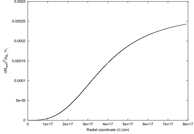
Figure 33: The factor \frac{\Delta M_{\text{ism}}^2}{\rho_{B1} V_1} is represented as a function of the radial coordinate. It is manifestly an increasing function.
