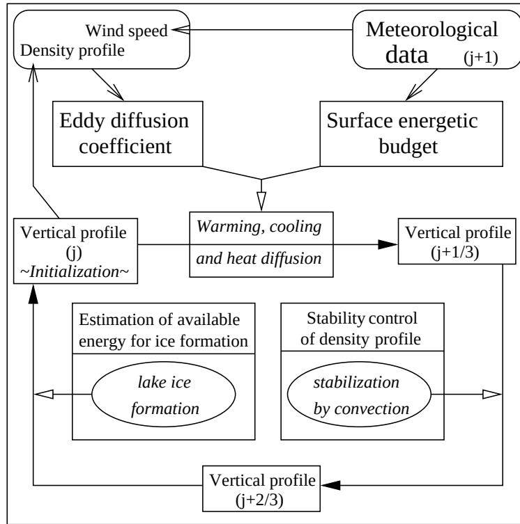
Figure 2.13: Algorithm of the one-dimensional eddy diffusion model. The simulation is initialized by an observed vertical lake water temperature profile (Vertical profile). The estimation of the vertical profile of the following day needs 1) the calculation of the eddy diffusion coefficient along the water column depending on the vertical water density profile of the previous day ( j ) and on the wind speed above the lake surface of the following day ( j+1 ); 2) the calculation of the surface energetic budget mainly depending on the meteorological data of the following day ( J+1 ); 3) after the warming and/or the cooling of each lake water layer of 1 m thick, the model controls the density stability of the new vertical profile ( j+1/3 ) and does the required stabilization; and 4) if the surface lake water temperature of the j+2/3 profile decreases below the freezing point of freshwater, the model induces lake ice formation and fixes the surface lake water temperature of the new profile ( j+1 ) at the temperature of this freezing point.
