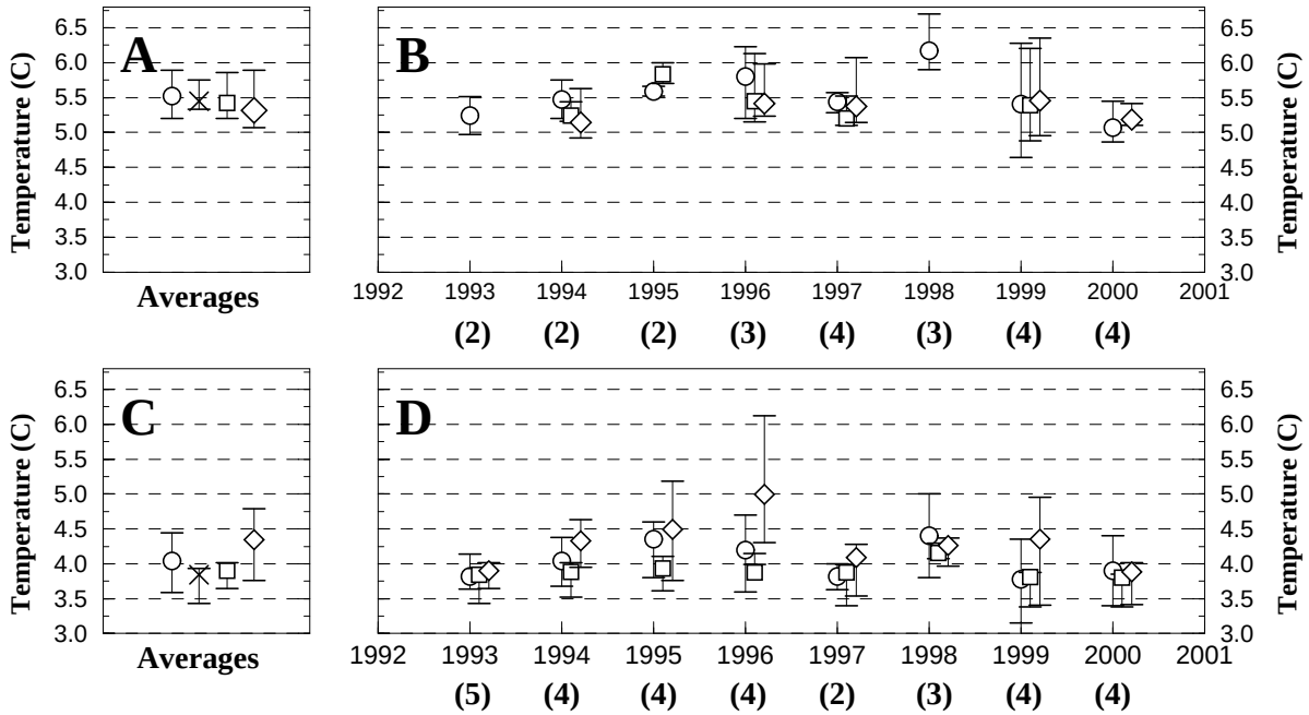
Figure 2.17: Observed (circles) and simulated (crosses, squares and diamonds) ostracod temperature (mean temperature for the calcification period of candonidae at the maximum depth, T_O ) in Lac d'Annecy (A and B) and in Ammersee (C and D). Numbers in parenthesis indicate how many instantaneous observed profiles were used for the calculation of the observed T_O . Crosses illustrate results of steady-state climatological simulations (A and C). Circles (observational data), squares (monthly simulations) and diamonds (daily simulations) simulated T_O illustrate decadal averages in figures A and C and, annual values in figures B and D. The error bars show the maximum and the minimum of the observed or simulated bottom water temperature used to calculate T_O .
