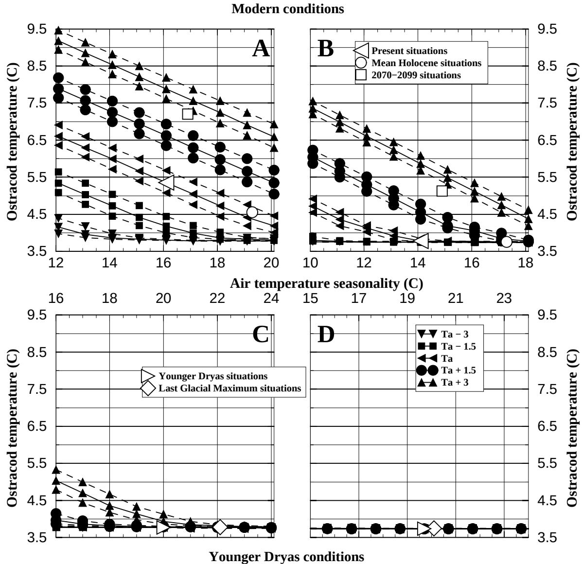
Figure 2.18: Sensitivity studies of the ostracod temperature for variations of the yearly air temperature ( T_a ), of the air temperature seasonality and of the yearly wind speed centered on the modern conditions (A : Lac d'Annecy and B : Ammersee) and centered on the Younger Dryas conditions (C : Lac d'Annecy and D : Ammersee). We considered T_a varying by \pm 1.5 and \pm 3^\circ\text{C} (filled symbols), the air temperature seasonality varying by \pm 1 , \pm 2 , \pm 3 , and \pm 4^\circ\text{C} (horizontal axis) and the yearly wind speed varying by \pm 10\% (upper dashed lines : -10\% and lower dashed lines : +10\% ), in order to bracket the probable extremes of the climatic development of the period recorded in the sediments of the two lakes. Opaque symbols point on the present situations (triangles left), the mid-Holocene climatic optimum situations (circles), a prediction of the climate for the end of the next century (squares), the Younger Dryas situations (triangles right) and the Last Glacial Maximum situations (diamonds). Climatic situations outputs result of PMIP (Paleoclimate Modeling Inter-comparison Project) boundary conditions [Masson et al. , 1999] for mid-Holocene (6000 B.P.) time periods, of ECHAM4/T42-REMO runs [Renssen et al. , 2001] for the Younger Dryas in Europe, of LMCELM5 runs [Masson et al. , 1998] for the Last Glacial Maximum (21,000 years B.P.) and of the coupled atmosphere-ocean Climate Model of the Centre National de Recherches Météorologiques using the SRES-B2 IPCC scenario [Douville et al. , 2002] for the end of the next century.
