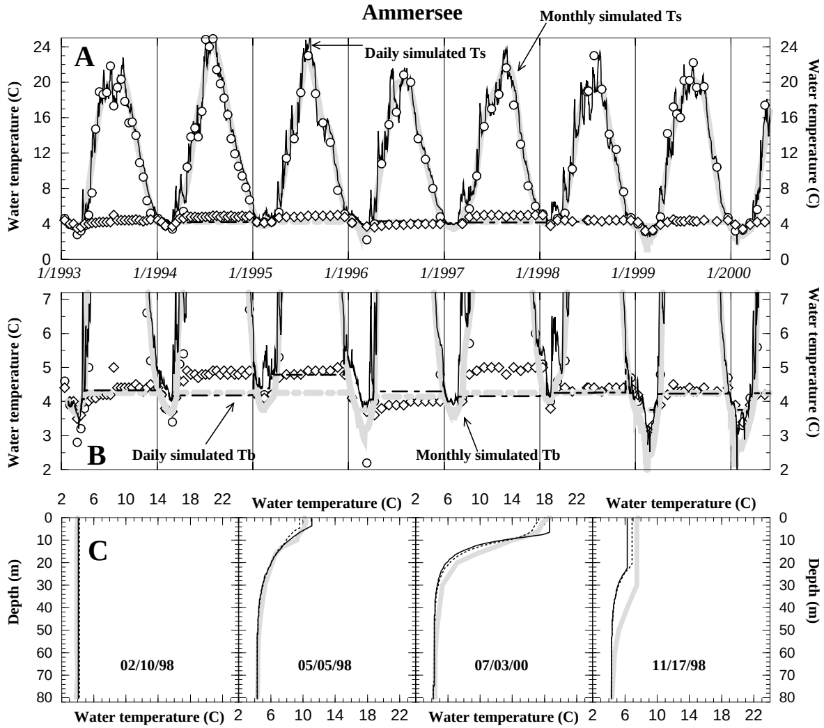
Figure 2.15: Best monthly and daily meteorological simulations. A : Monthly (large gray lines) and daily (fine black lines) simulations of surface and bottom water temperature. B : Zoom on the bottom water temperature. C : Typical monthly (solid lines) and daily (dotted lines) simulated vertical profiles. Circles (surface water temperature on A and B), diamonds (bottom water temperature on A and B) and large gray lines (vertical temperature profiles on C) are observational data from Ammersee.
