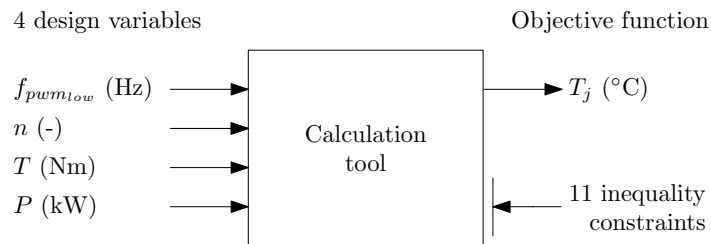
Figure 5.5: Optimization problem
