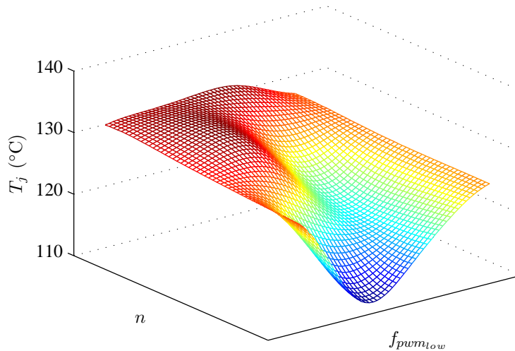
Figure 5.6: Surrogate model of the objective function
