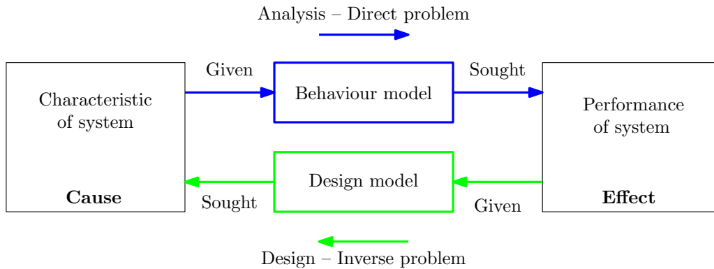
Figure 1.3: Input and output of direct and inverse problems
