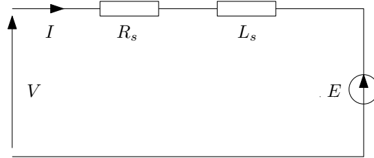
Figure B.9: Single-phase equivalent electric model
