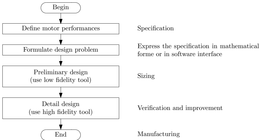
Figure 4.1: Traction motor design methodology
