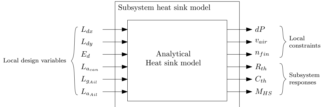
Figure 5.14: Subsystem heat sink model
