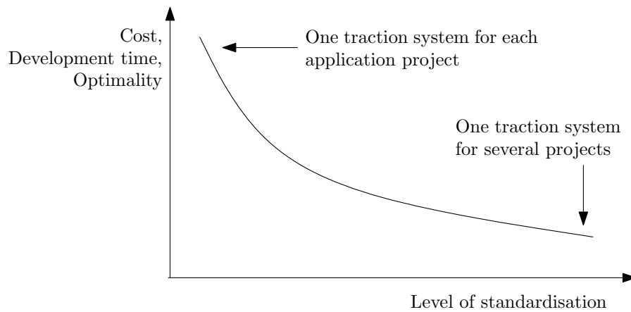
Figure 1.19: Standardisation
