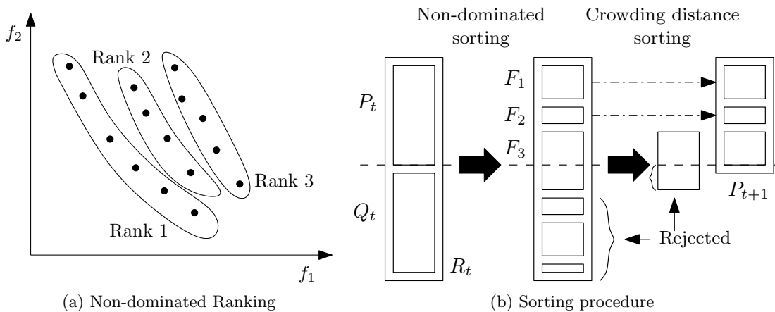
Figure 3.11: NSGA-II
