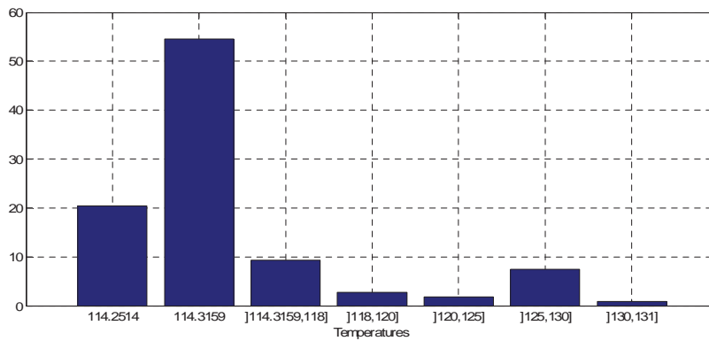
Figure 5.7: Multimodal problem
