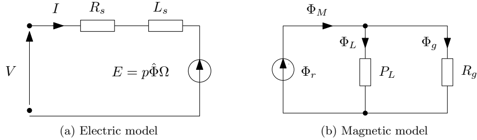
Figure 2.2: Analytical model of a permanent magnet motor
