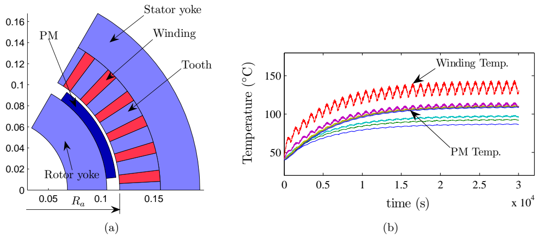
Figure 4.15: (a) Optimal motor, (b) Simulation of an optimal motor on the load cycle. The figure shows various temperatures.
