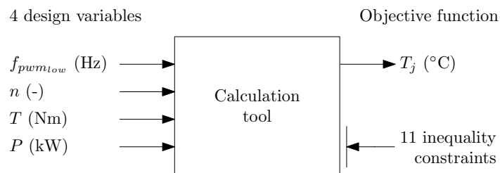
Figure 5.5: Optimization problem
