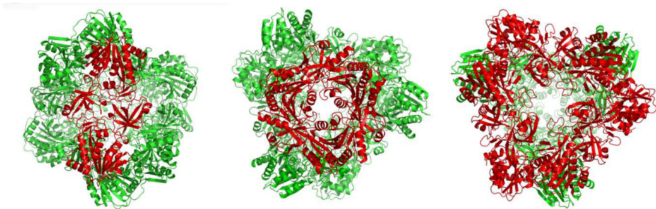
(c) Crystallographic model of the complex.
