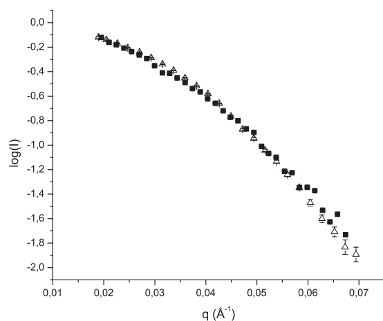
Fig. 5. Logarithm of the SANS intensities of PhTET3 at 20°C ( \Delta ) and 90°C ( \blacksquare ) as a function of the scattering vector q ( q = 4\pi l^{-1} \sin 2\theta , \lambda being the wavelength and \theta the scattering angle). Within the experimental errors, both curves show high similarity. Where no error bars can be seen, the error is smaller than the symbol of the curve.
