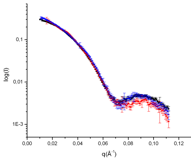
Figure 5.5: Superposition of scattering curves of PhTET3. The shape of the three curves, one at pH 7, 25°C and atmospheric pressure (■), one at pH 7, 60°C, 3000 bar (●) and one at pH 9, 90°C, 3000 bar (▲), is identical.
