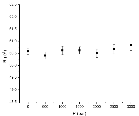
(a) Radius of gyration of PhTET3 at pH9
