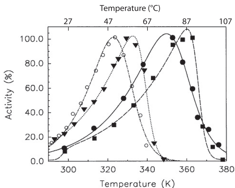
Figure 1.2: Activity at different temperatures for hydrogenases from M. igneus (squares), M. jannaschii (filled circles), M. thermolithotrophicus (triangles) and M. maripaludis from [50]. The first two organisms are hyperthermophiles, M. thermolithotrophicus is a thermophile and M. maripaludis is a mesophile. The enzymes display maximum activity at different temperatures as they are adapted to different habitat temperatures.
