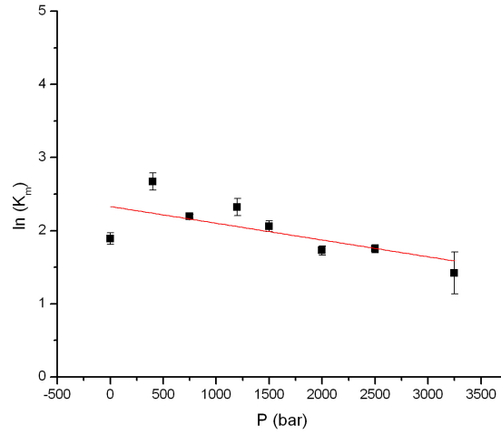
(a) K_m as a function of pressure.
