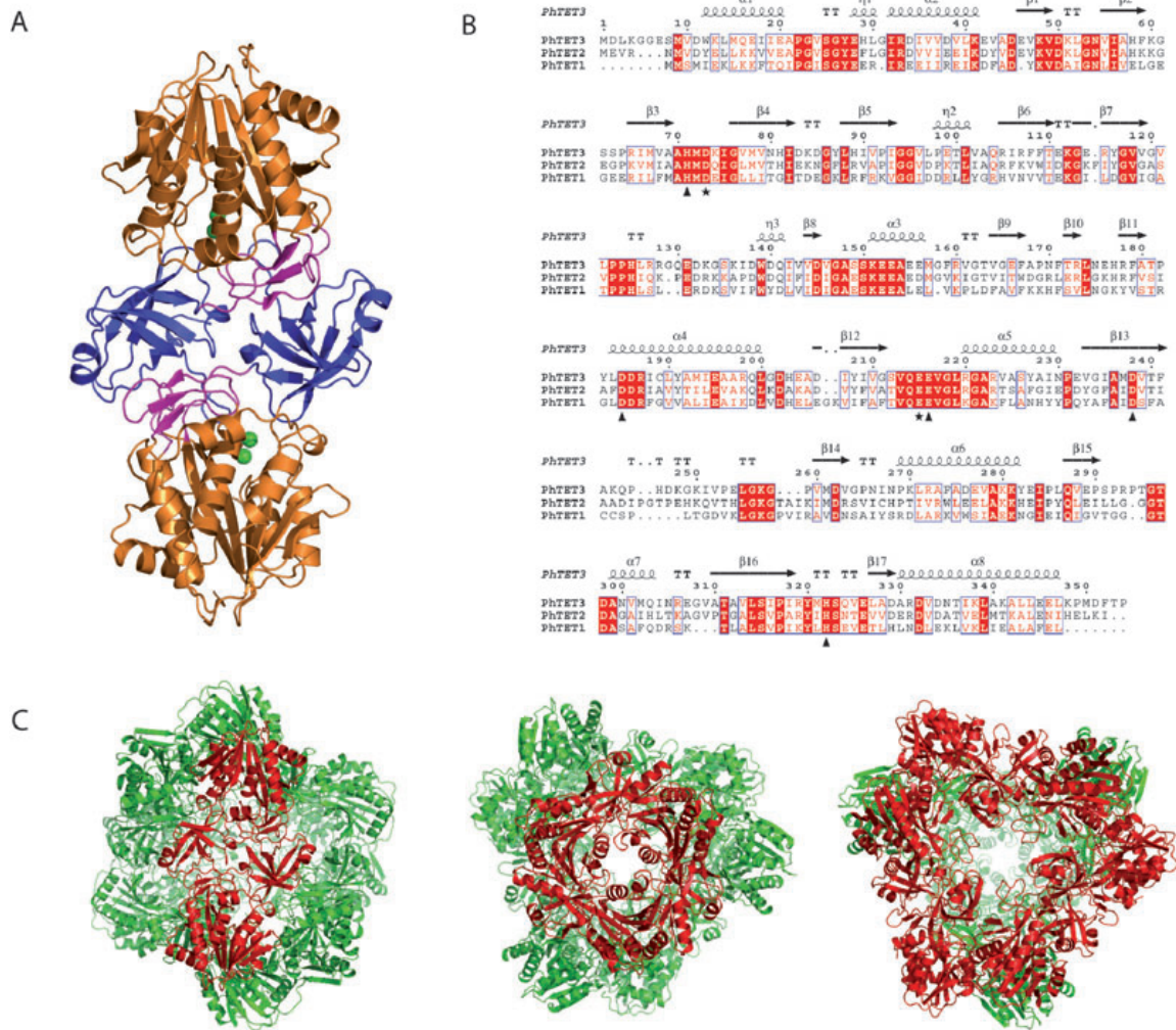
Fig. 1. A. View of the PhTET3 dimer along the twofold symmetry axis. The catalytic domain of each monomer is coloured in orange with the additional four-stranded \beta -sheet in magenta. The dimerization domain is represented in blue and the catalytic zinc ions are depicted as green spheres. The dimerization domain of each monomer interacts with the peripheral \beta -sheet of the catalytic domain of the other monomer to form the dimer.
