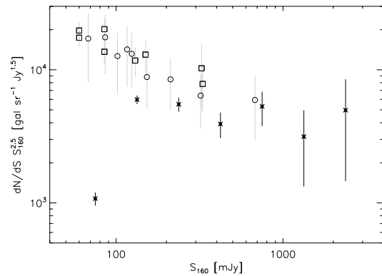
Fig. 1. 160 \mu\text{m} differential number counts for our sample of 372 galaxies individually detected at 8, 24, 70 and 160 \mu\text{m} (black stars) as compared to the counts obtained in the Marano and CDFS fields by Dole et al. (2004a) (open squares) and in the FLS by Frayer et al. (2006) (open circles). This shows that we are uniformly sampling the far-infrared population over a large range of 160 \mu\text{m} fluxes.
