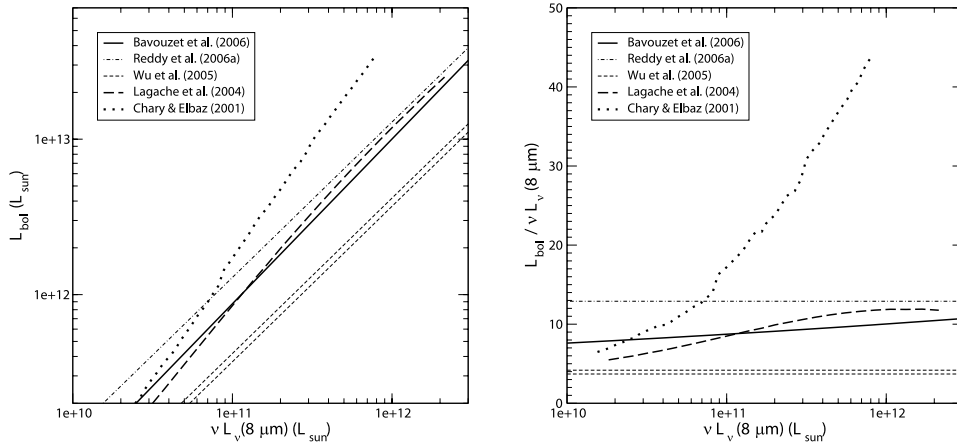
FIG. 12.—Comparison between different L_{\text{bol}}^{\text{IR}} vs. \nu L_{\nu}^{8 \mu\text{m}} relations ( left ) and derived conversion factors vs. \nu L_{\nu}^{8 \mu\text{m}} ( right ), as obtained from different calibrations available in the literature.
